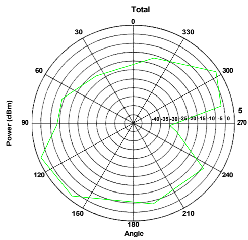
XY Plane at Freq = 2.450GHz
