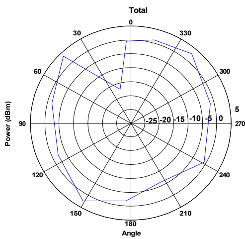
YZ Plane at Freq = 2.500GHz
