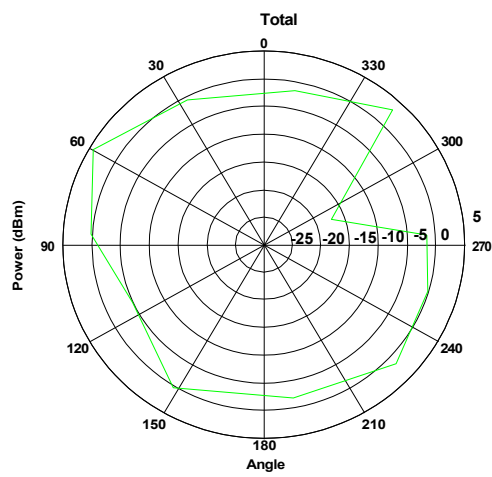
YZ Plane at Freq = 2.450GHz
