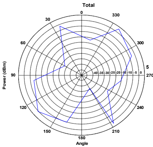
XZ Plane at Freq = 2.500GHz
