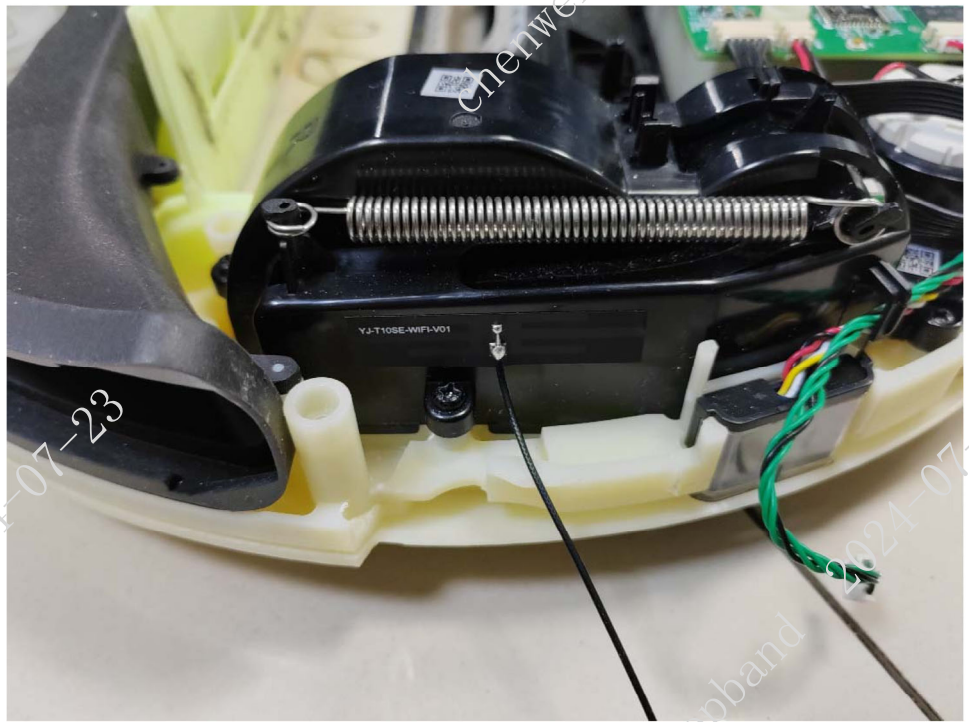
WIFI Antenna
