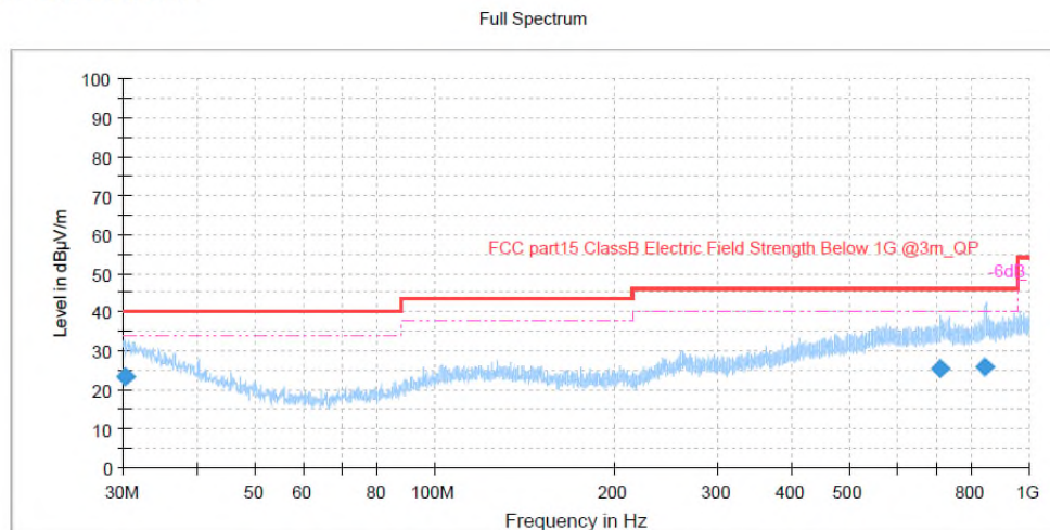
Figure 5: Spectral Diagrams, Radiated Emission, Below 1GHz, Horizontal, AC 120V
