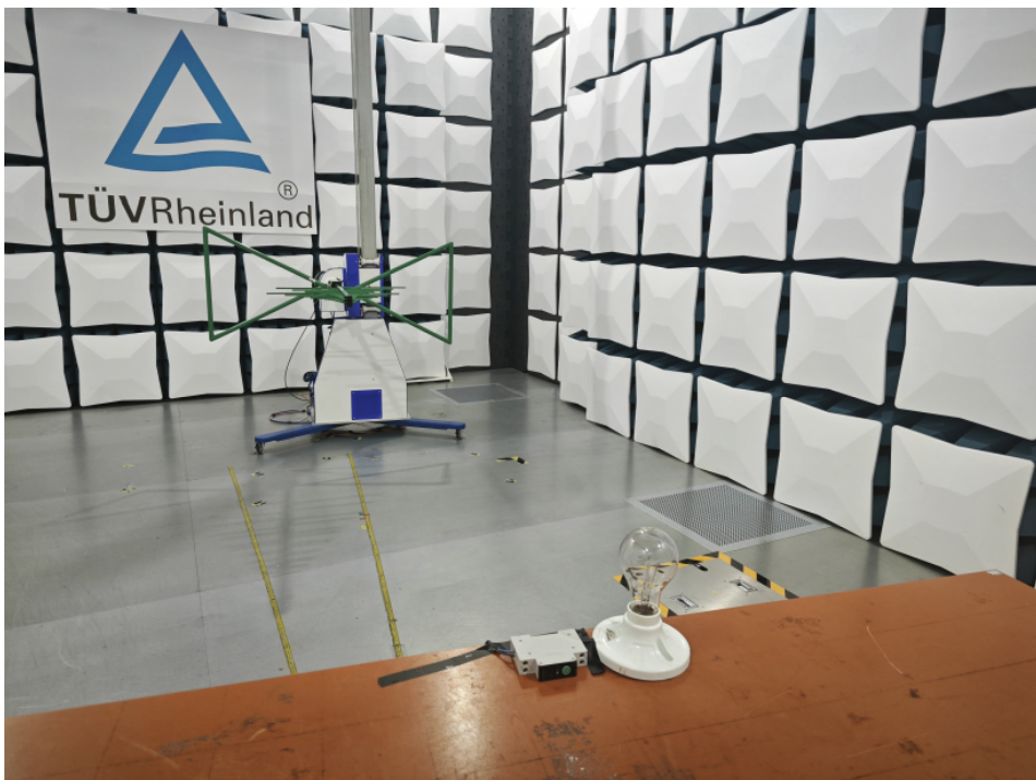
Test Set-up: Radiated Emission, Below 1GHz
