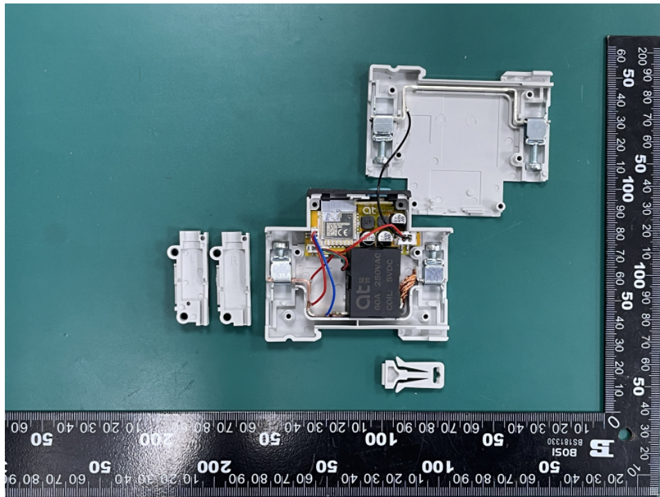
TO-Q-SY1-JZT Internal view
