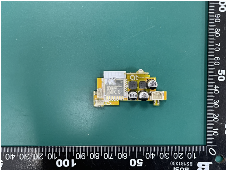
TO-Q-SY1-JZT Internal view: PCB
