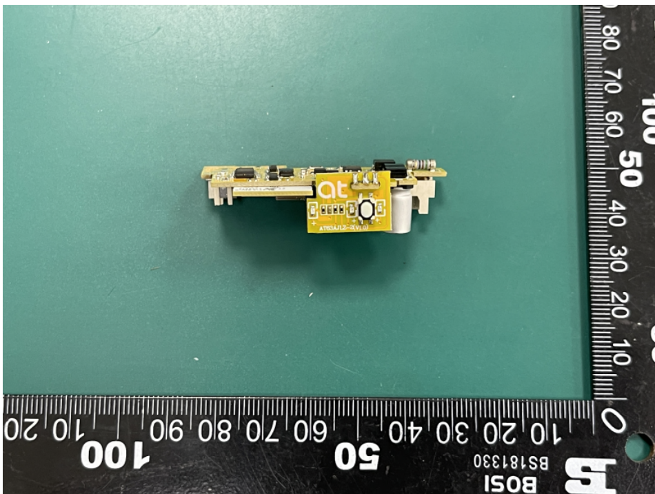
TO-Q-SY2-JZT Internal view: PCB
