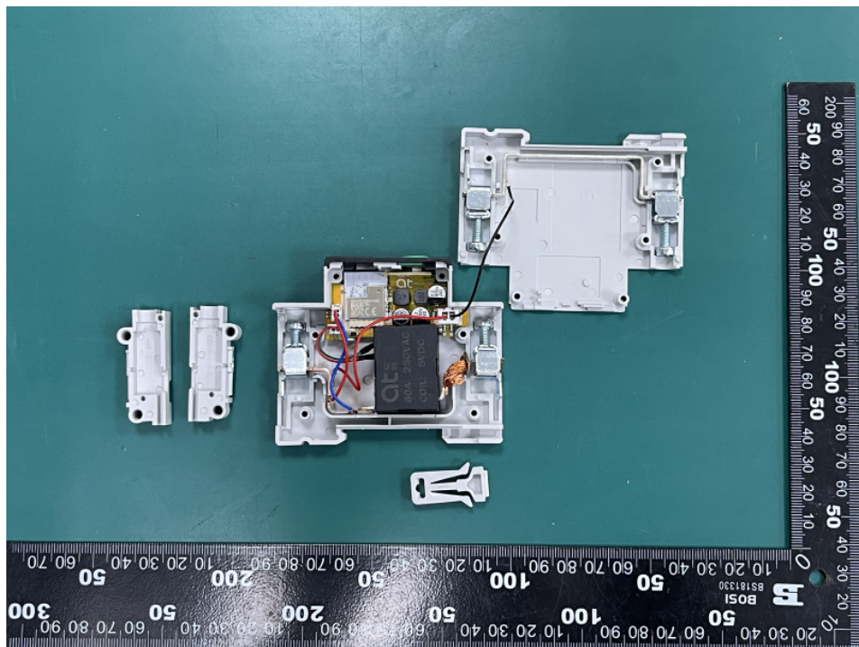
TO-Q-SY2-JZT Internal view
