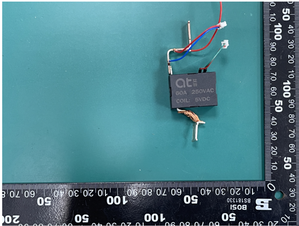
TO-Q-SY1-JZT& TO-Q-SY2-JZT Internal view: Latching Relay
