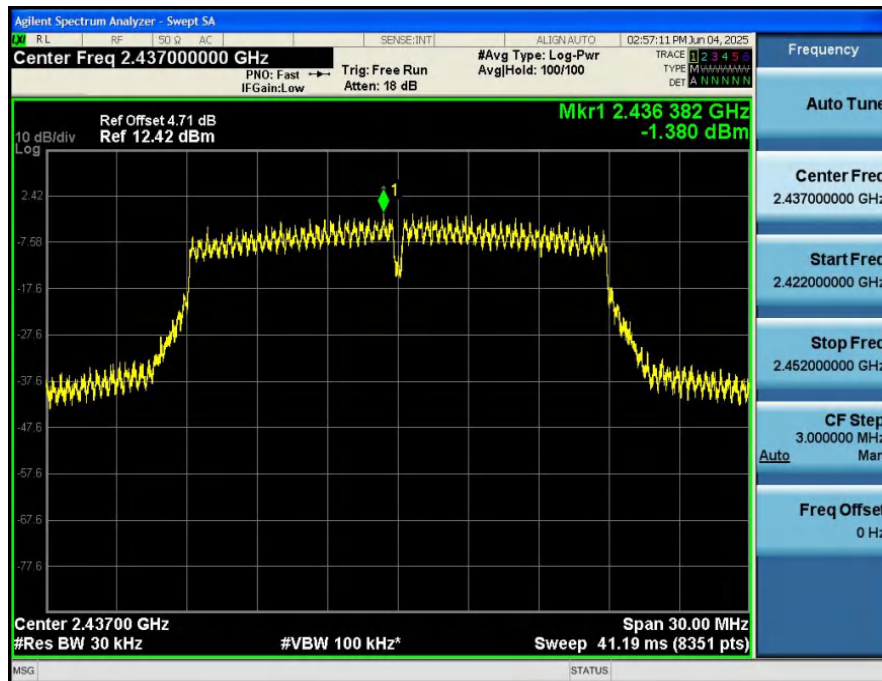
Power_Spectral_Density_NVNT_ANT1_802_11n(HT20)_2437
