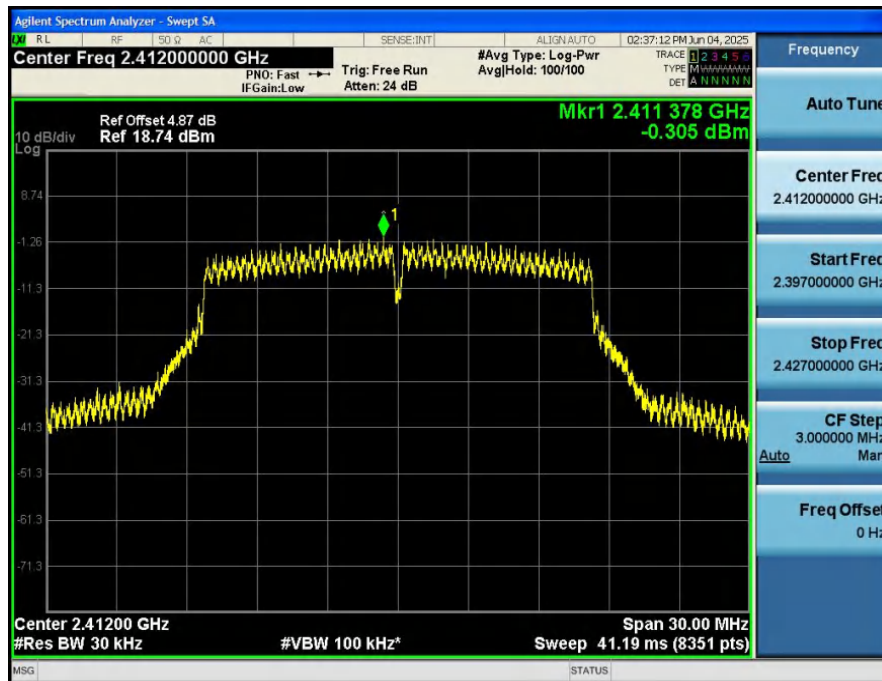
Power_Spectral_Density_NVNT_ANT1_802_11g_2412
