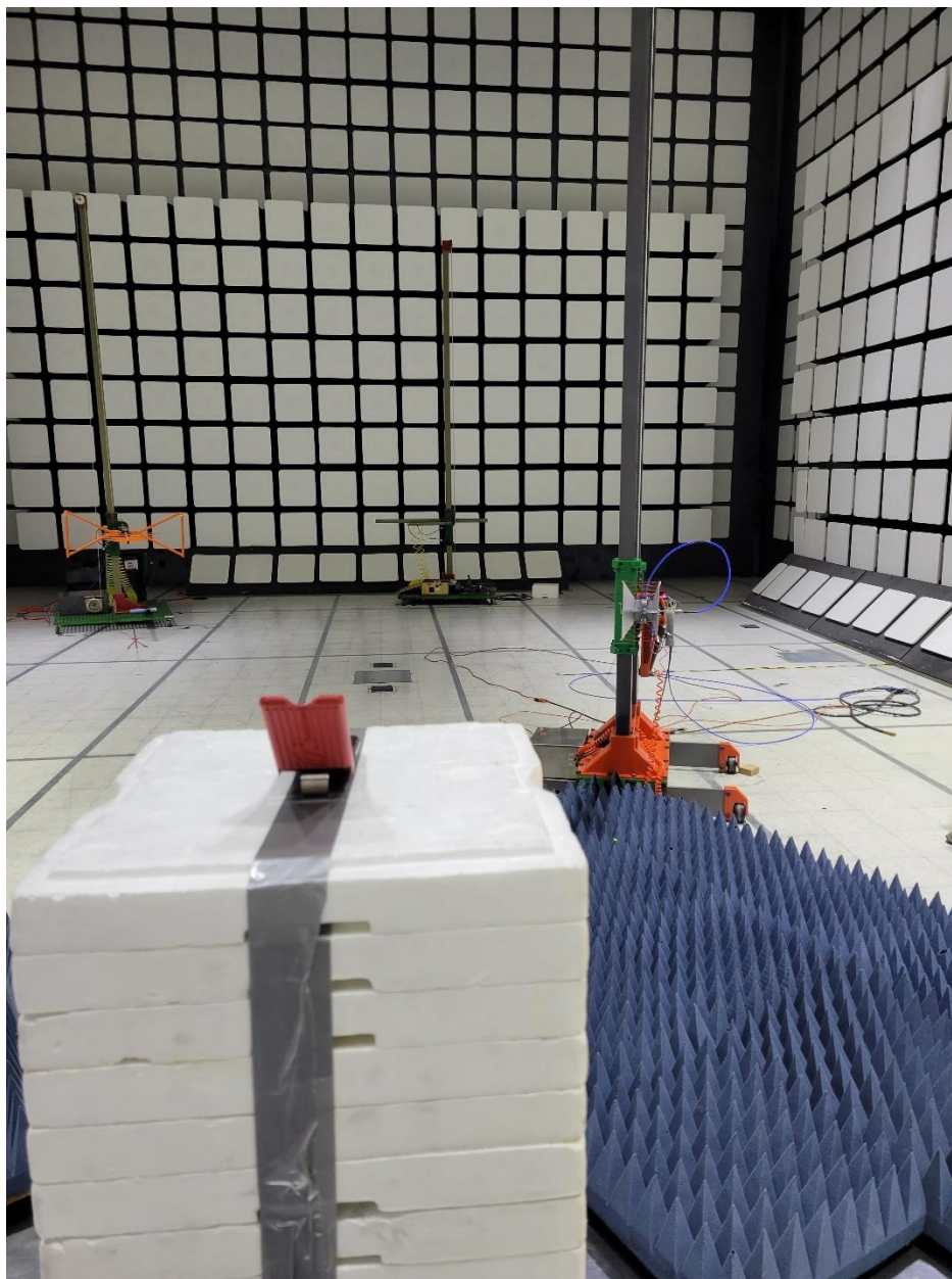
1 – 18 GHz Test Setup
