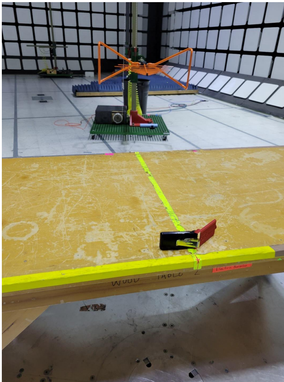
30 MHz – 1 GHz Test Setup
