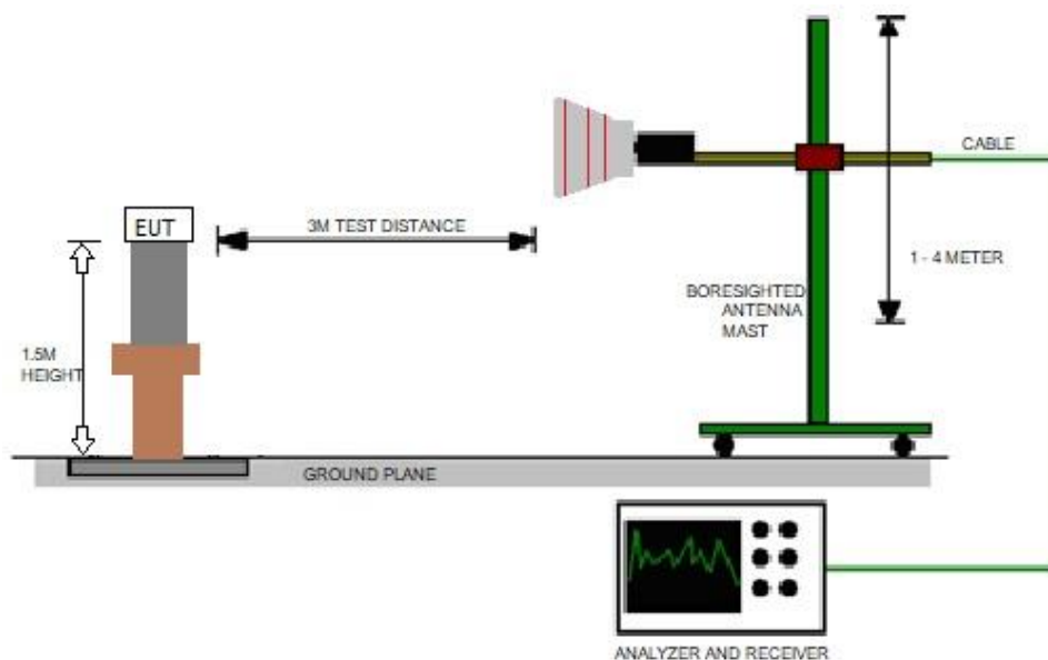
Figure 3 - Radiated Emissions Test Setup, >1GHz
