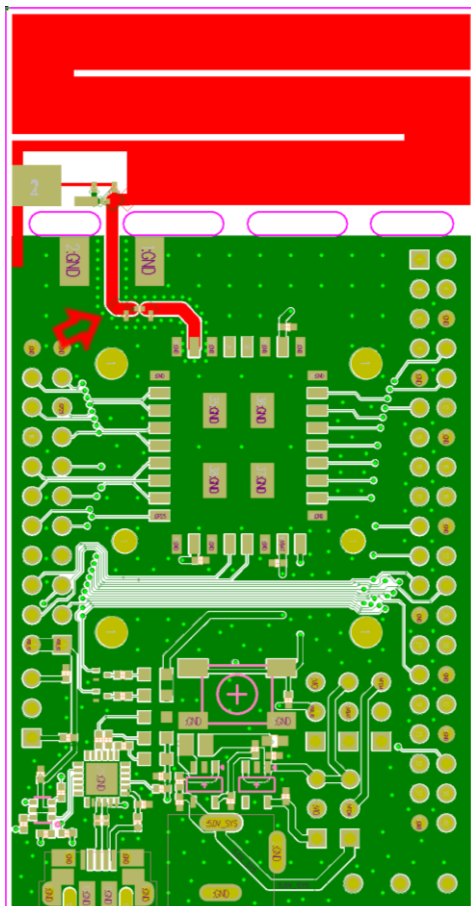
➔ : 50 ohm matching Transmission Line [PCB Top]
