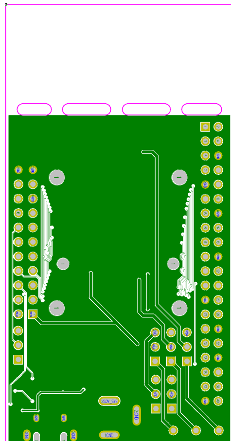
[PCB Bottom]
