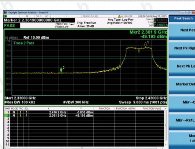
Left bandedge
