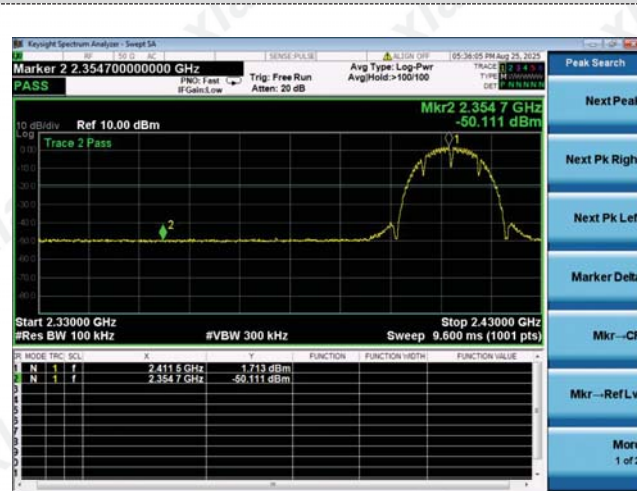
Left bandedge
