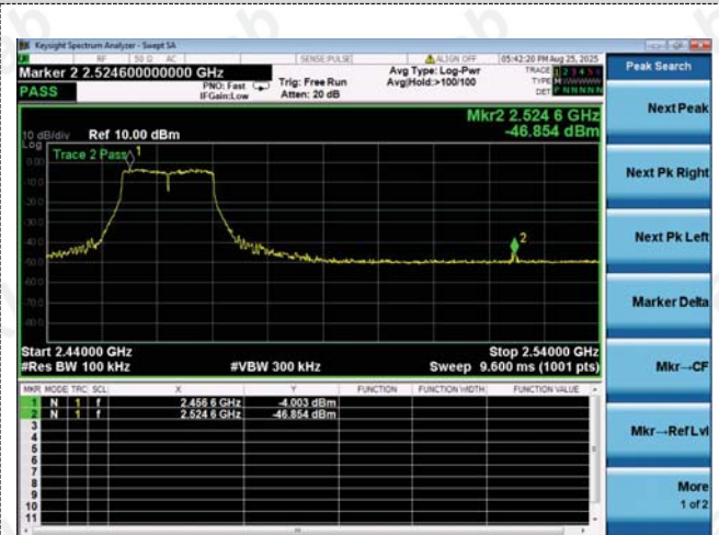
Right bandedge
