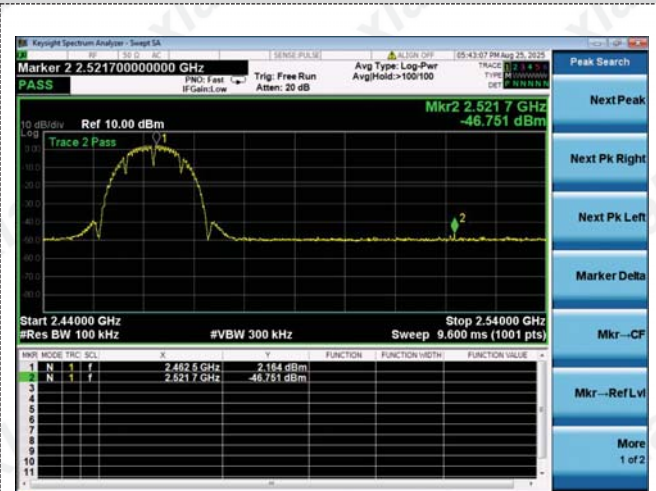
Right bandedge
