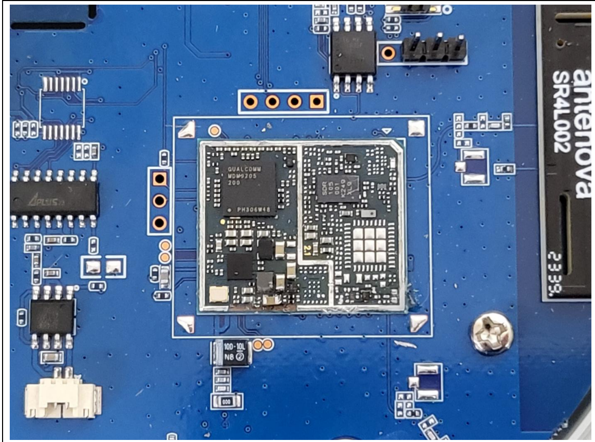
Inside shieldcan
