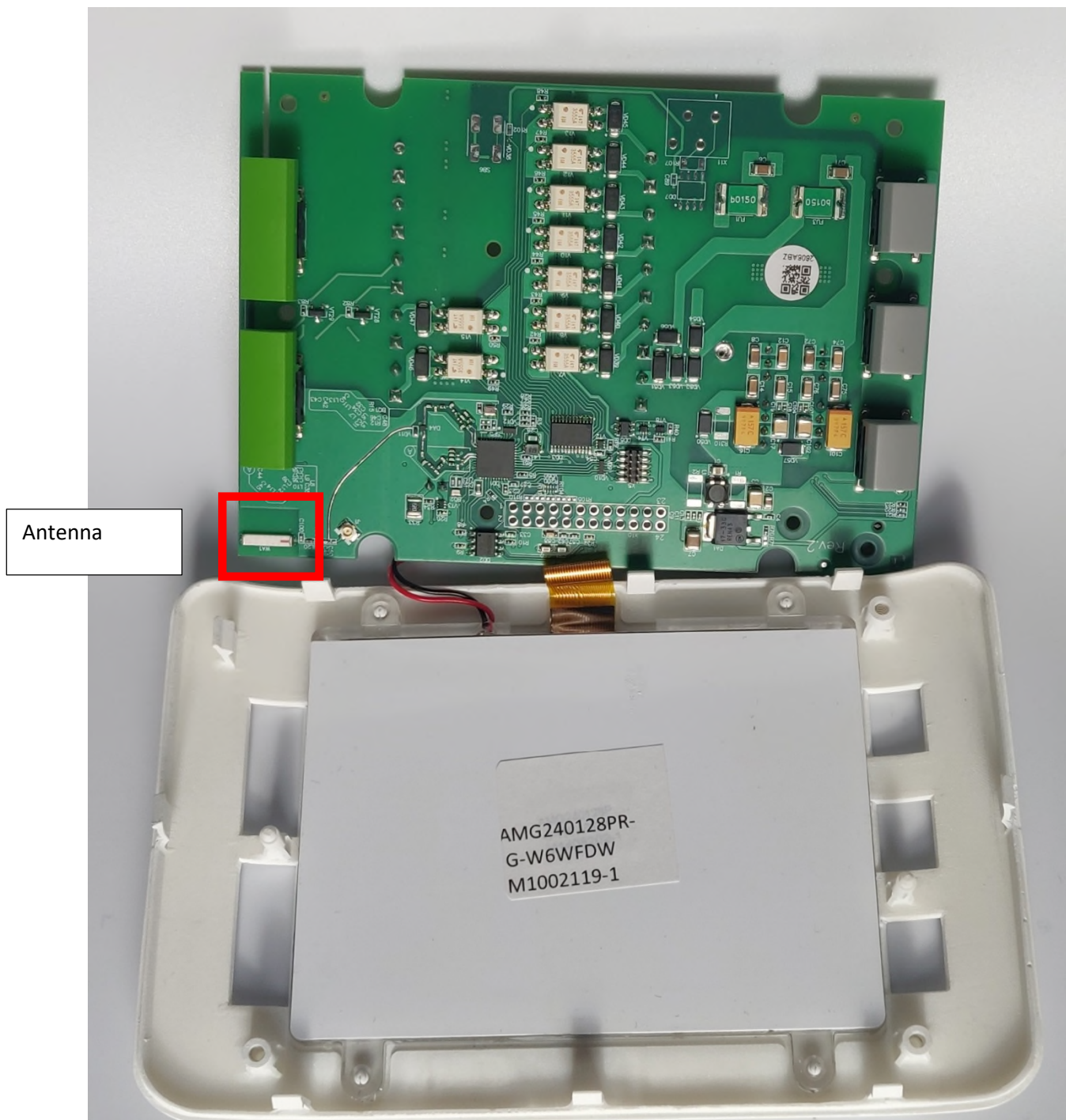
Figure 2 – Back Thermostat
