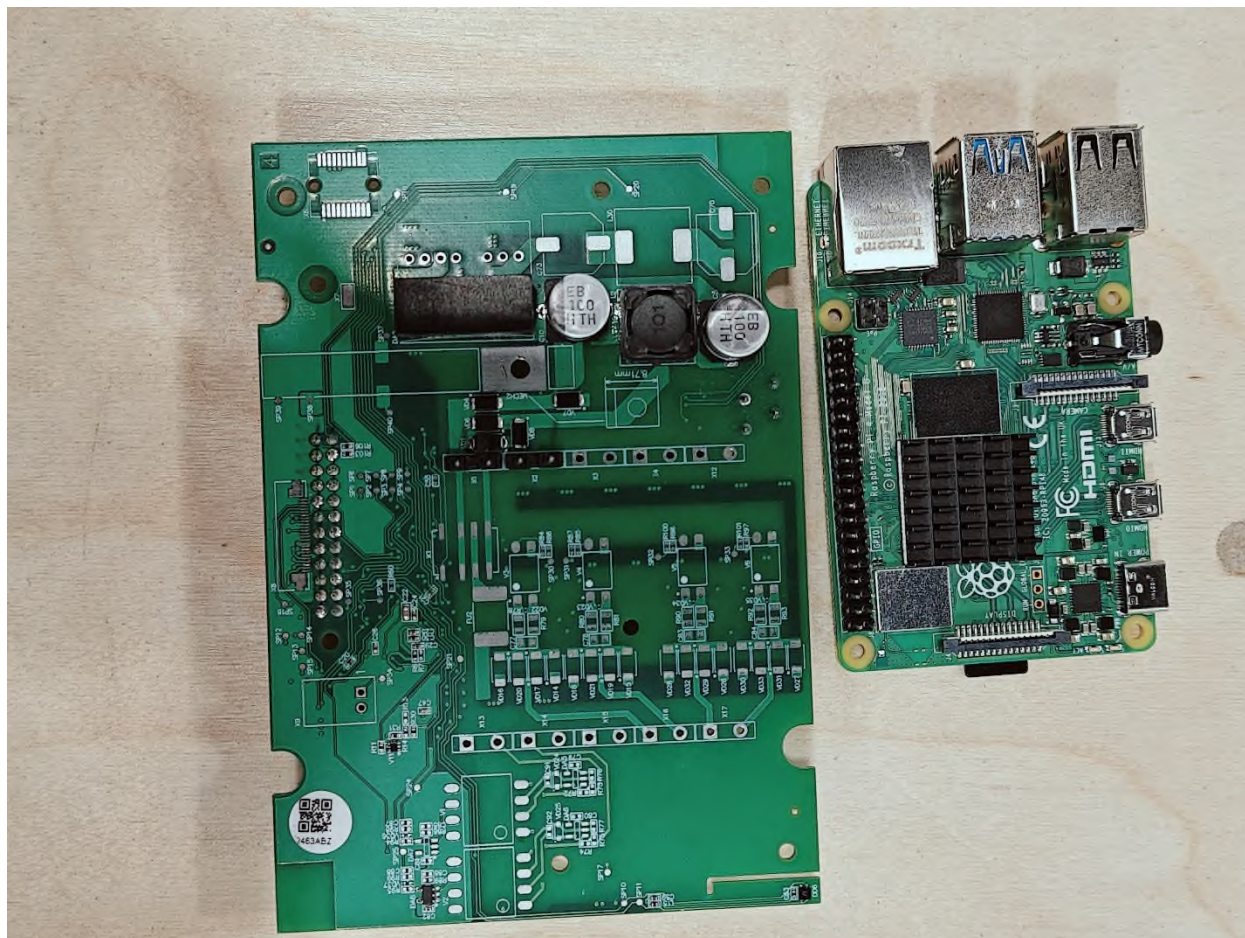
Figure 3 – Back Gateway
