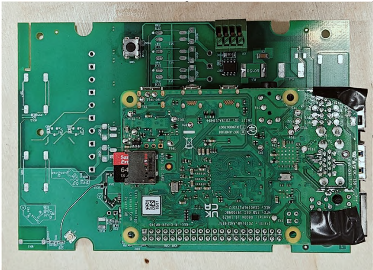
Figure 1 – Front Gateway
