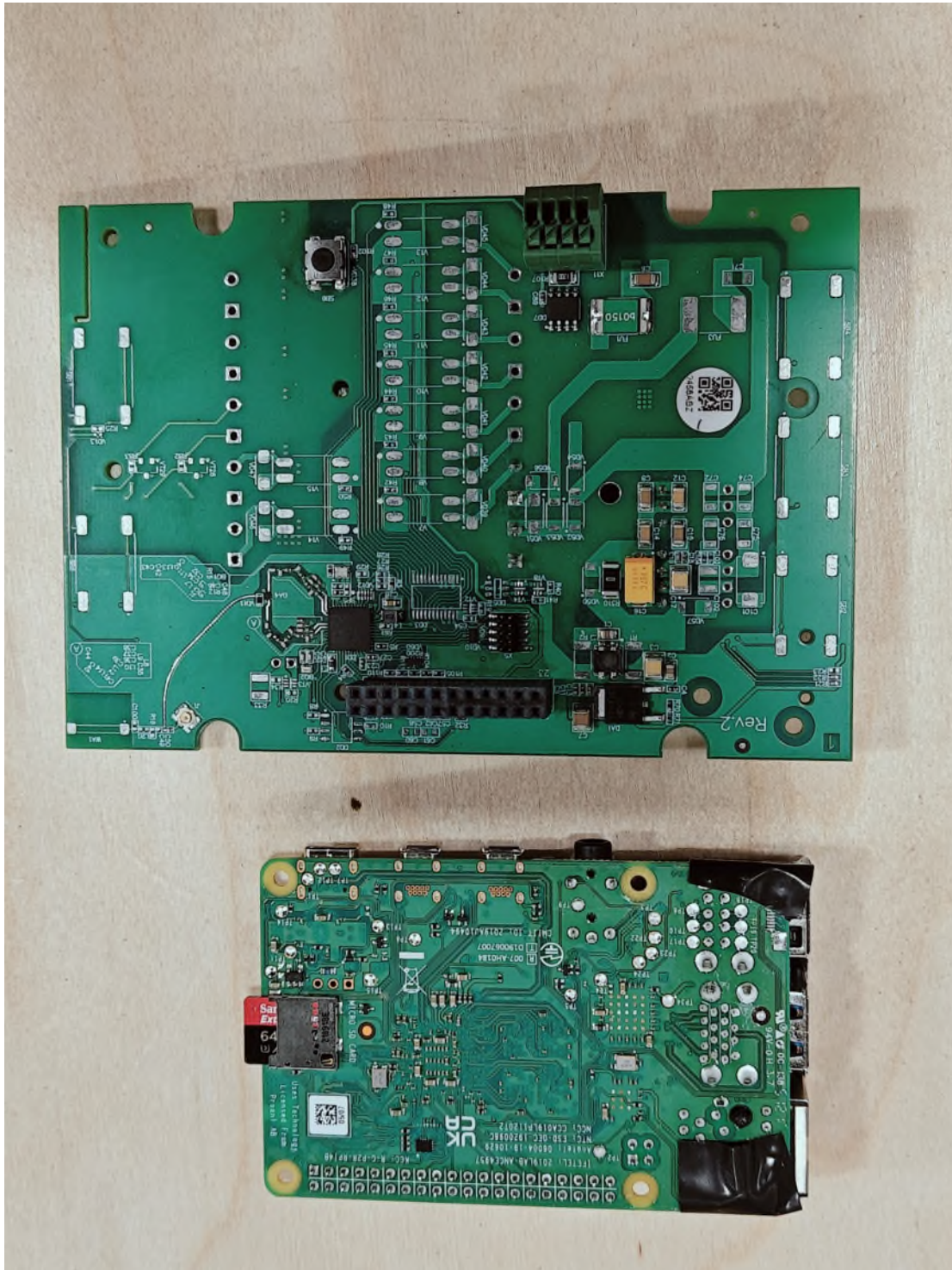
Figure 2 – Front Gateway
