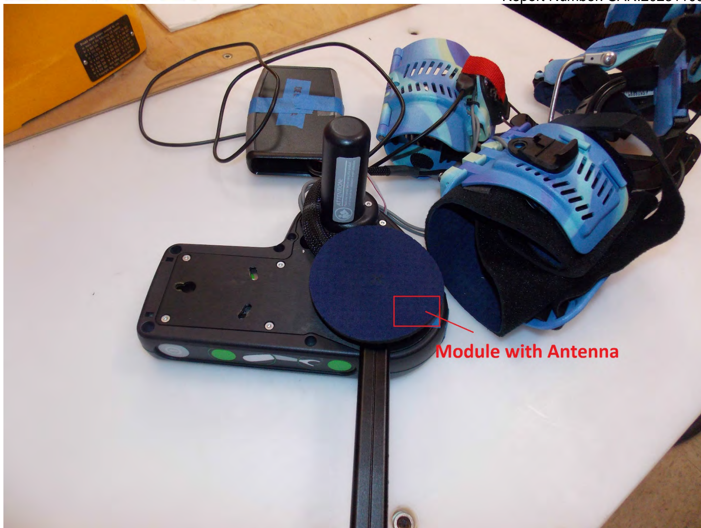
Back of Device Disassembled
