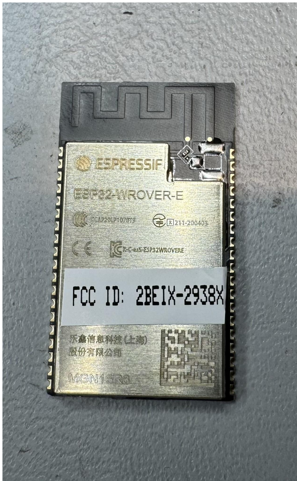
Figure 2: Label Location
