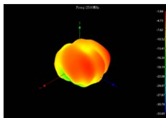
Freq:2500MHz
