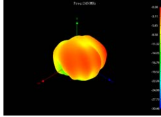
Freq:2450MHz
