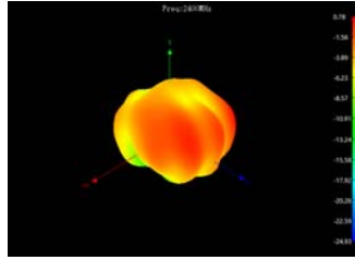
Freq:2400MHz
