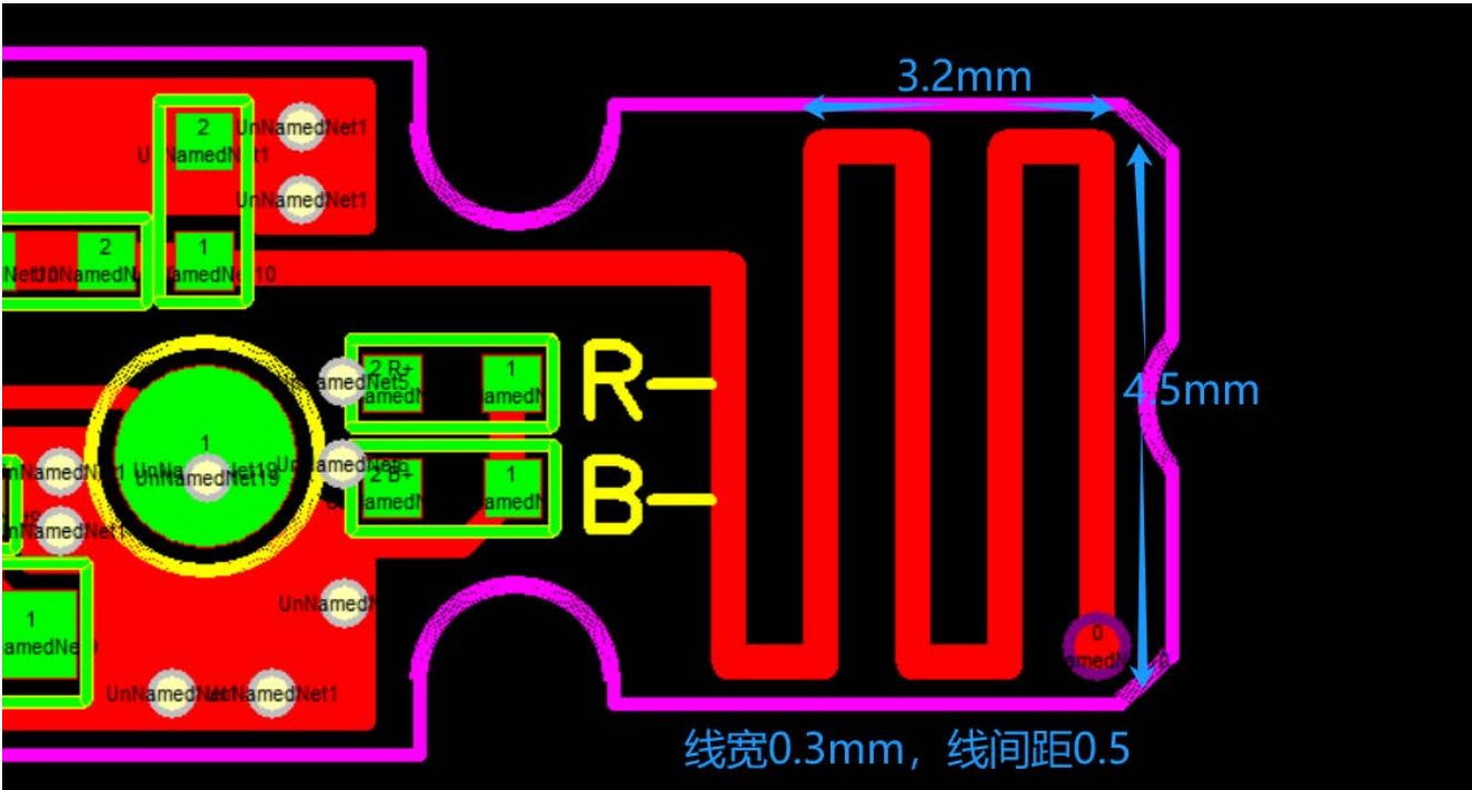
Antenna shape
