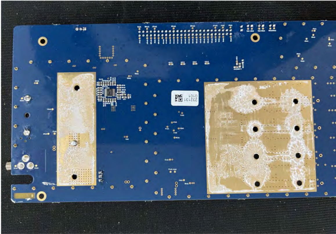
MARS – ATR Diplexer board (bottom zoom view)
