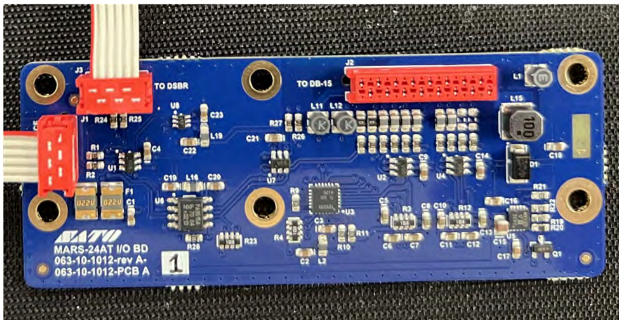
Universal MARS IO board (top zoom view)
