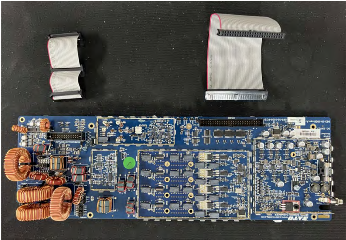
MARS – ATR Diplexer board (top zoom view)
