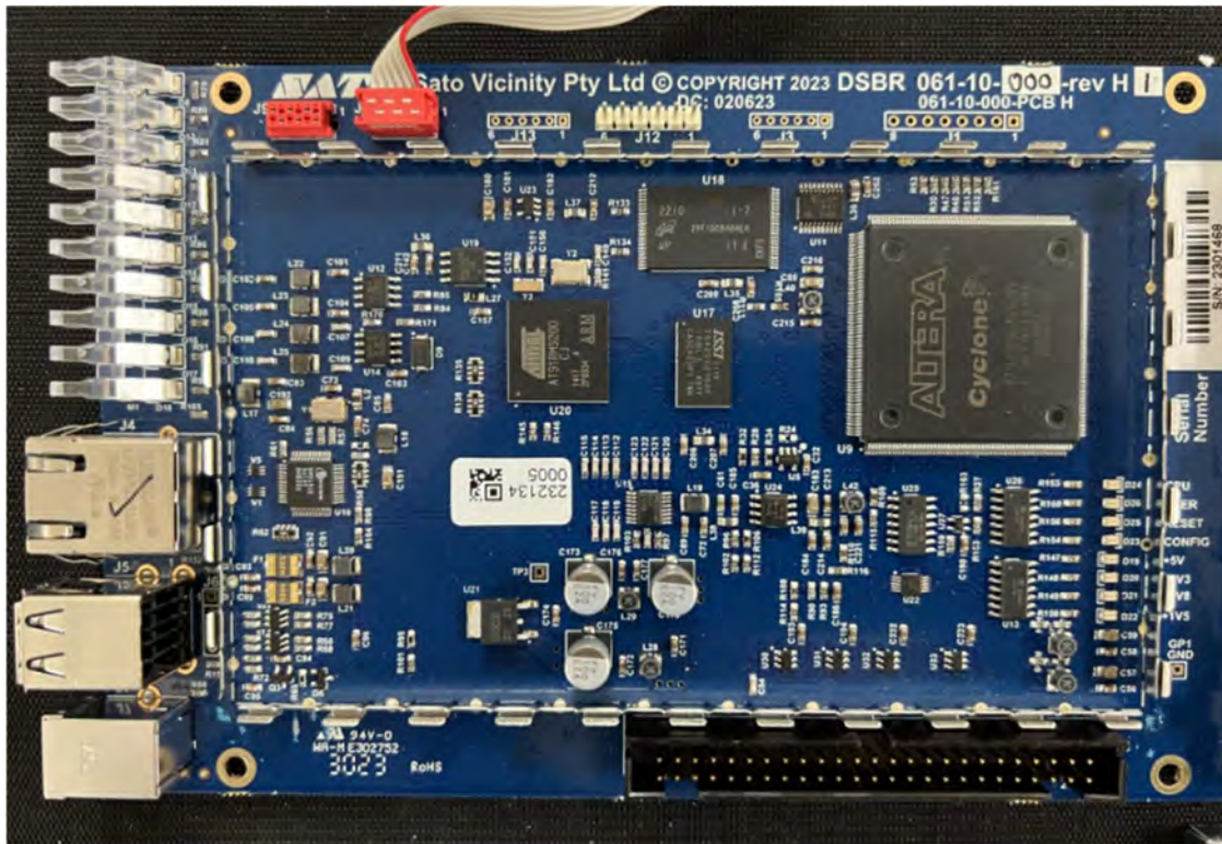
DSBR board (top zoom view)
