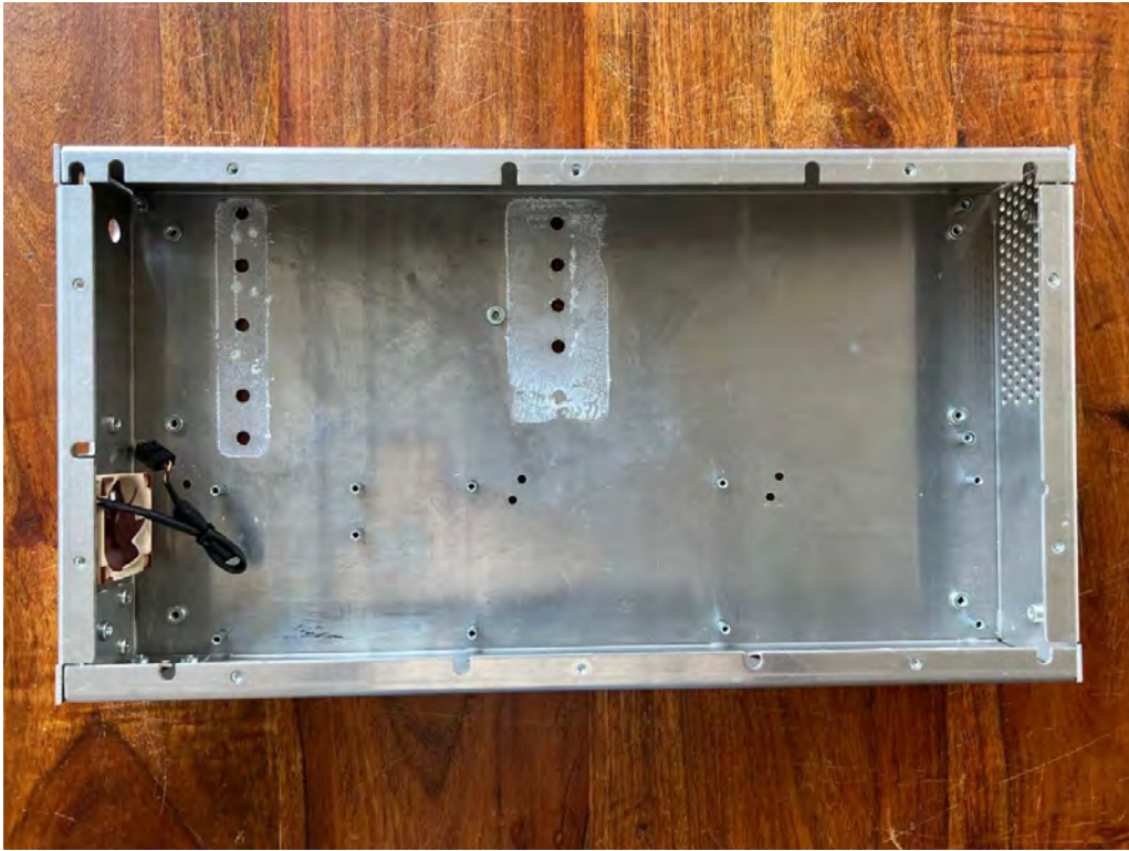
Enclosure (bottom view)
