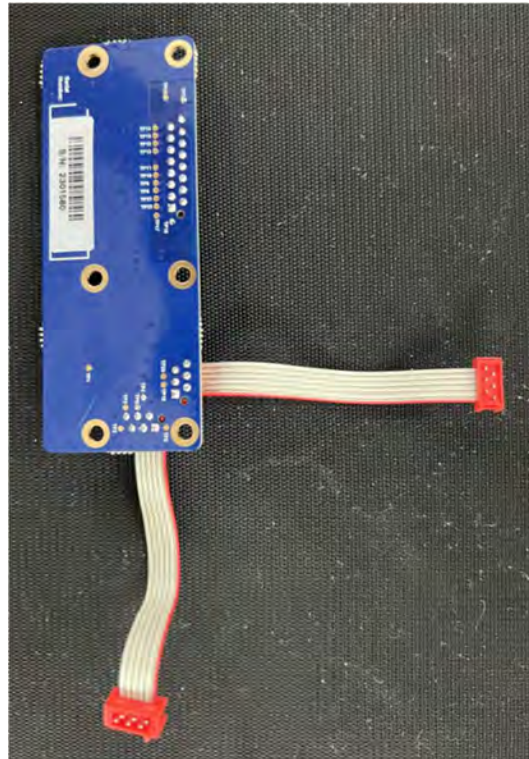
Universal MARS IO board (bottom view)
