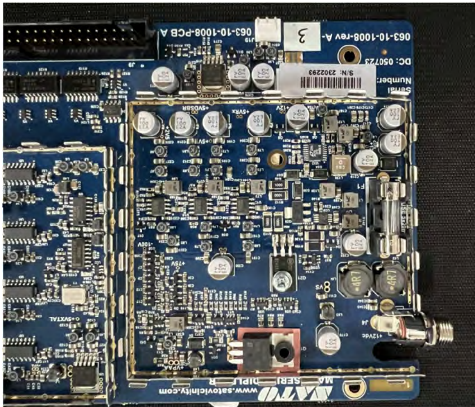
MARS – ATR Diplexer board (top zoom view)
