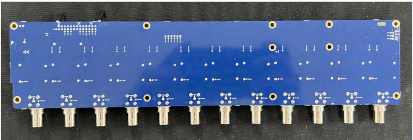
2 nd Antenna Interface board (bottom view)
