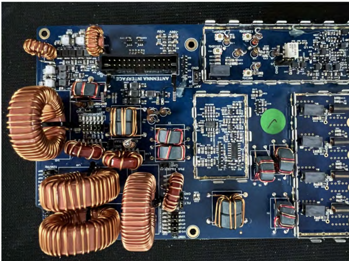
MARS – ATR Diplexer board (top zoom view)
