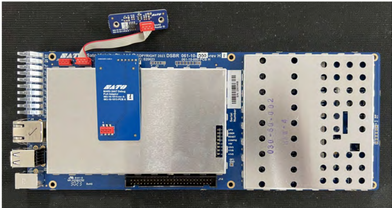
DSBR board (top view)
