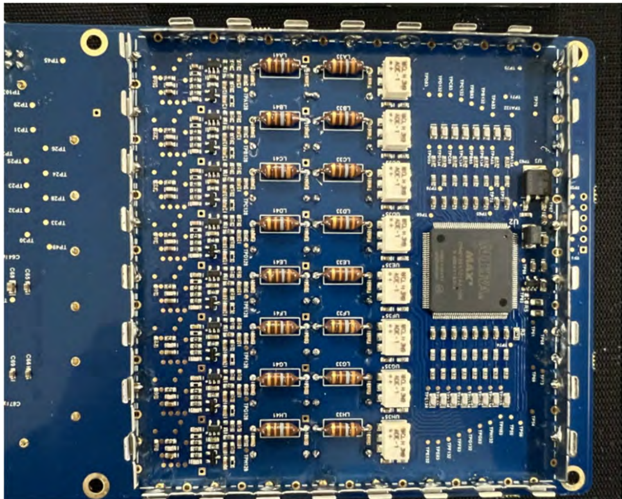
DSBR board (bottom zoom view)
