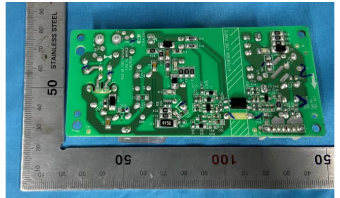
PCB8 Back
