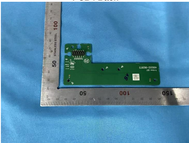
PCB5 Back
