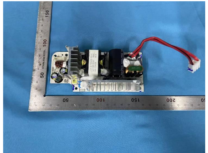
PCB4 Front
