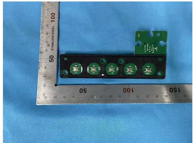
PCB5 Front
