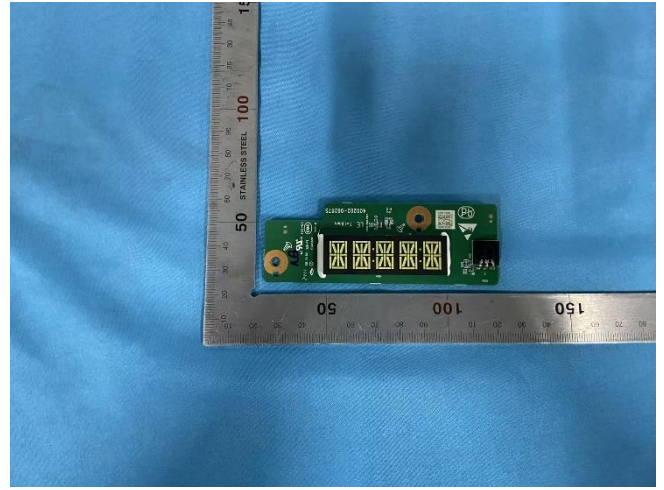
PCB1 Front
