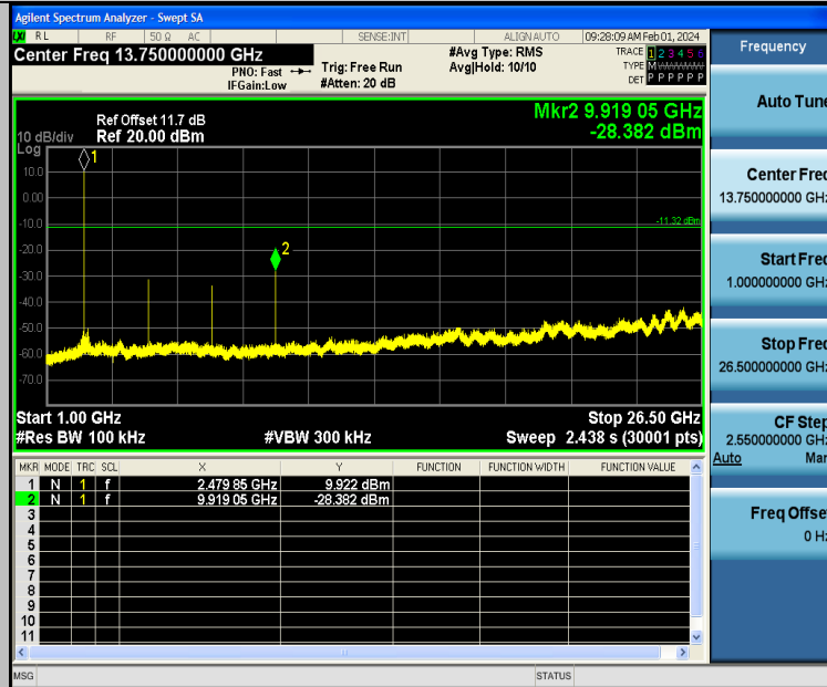
BLE_1M-Ant2-2480-1000~26500-PASS
