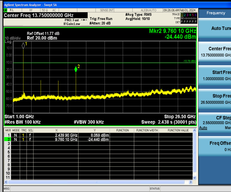
BLE_1M-Ant2-2440-1000~26500-PASS
