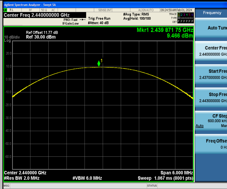
BLE_1M-Ant2-2440-PASS
