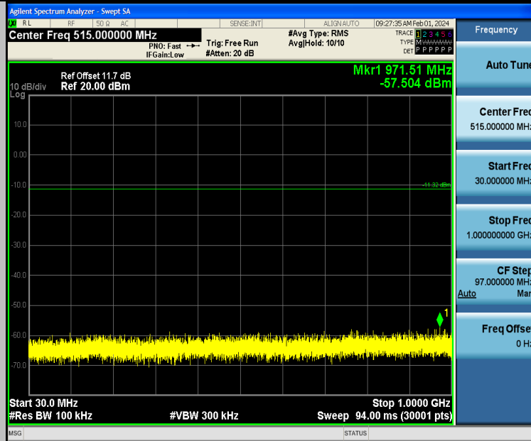
BLE_1M-Ant2-2480-30~1000-PASS
