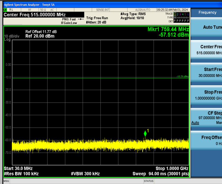
BLE_1M-Ant2-2440-30~1000-PASS
