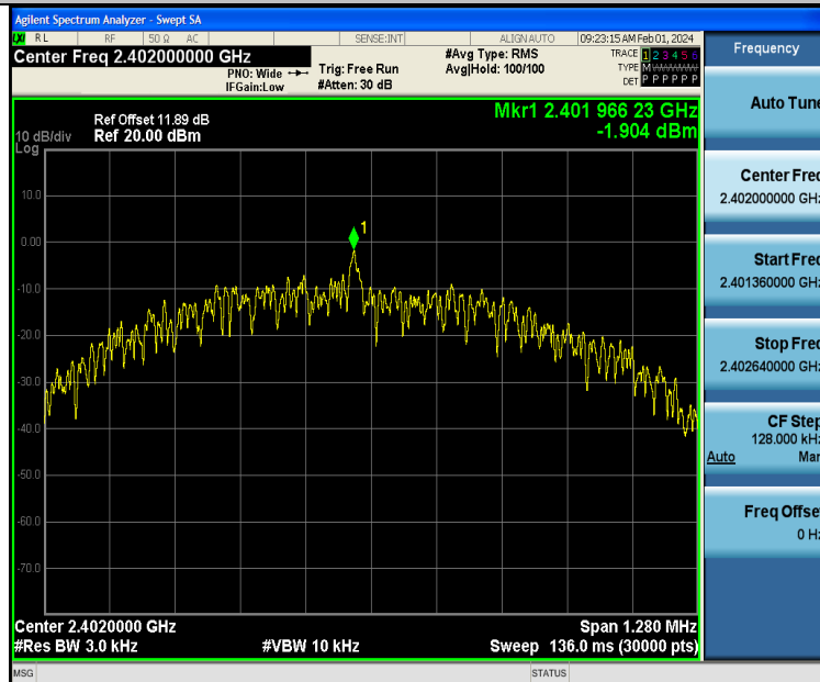
BLE_1M-Ant2-2402-PASS
