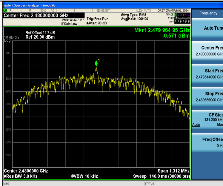
BLE_1M-Ant2-2480-PASS
