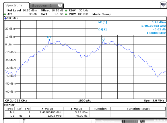
GFSK_Low
