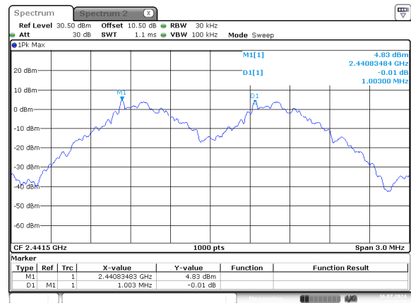
GFSK_Middle
