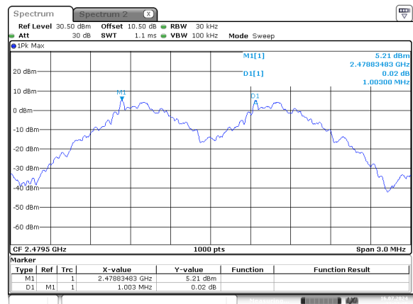
GFSK_High
