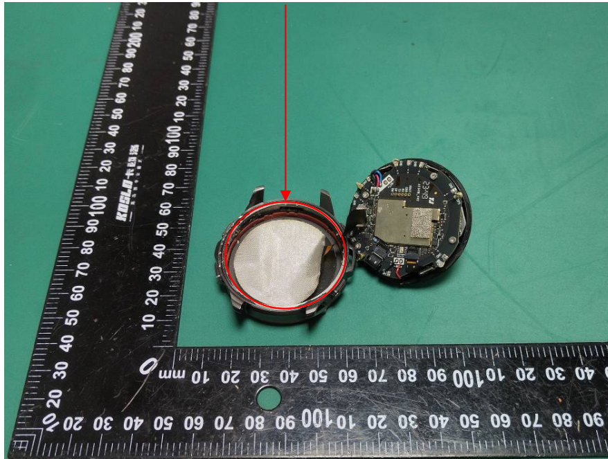
Antenna location
