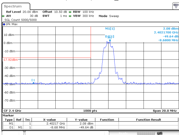
EDR(8DPSK) 3DH1_Low
