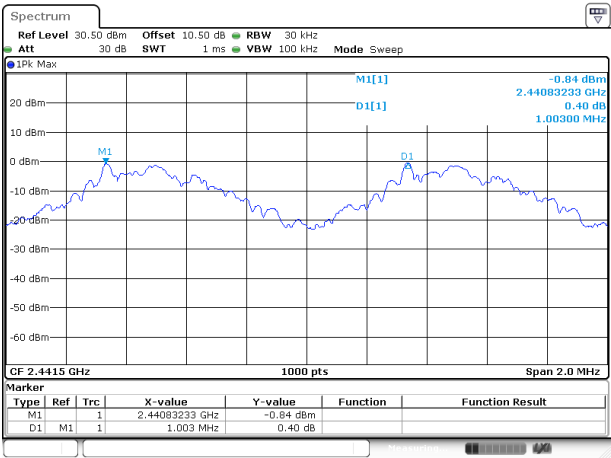
BDR(GFSK) DH1_Middle
