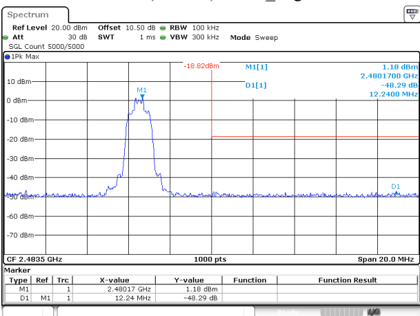
EDR(8DPSK) 3DH1_High
