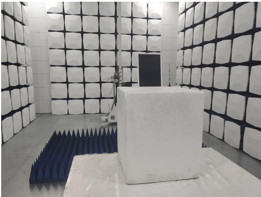
Above 1GHz for LTE test
