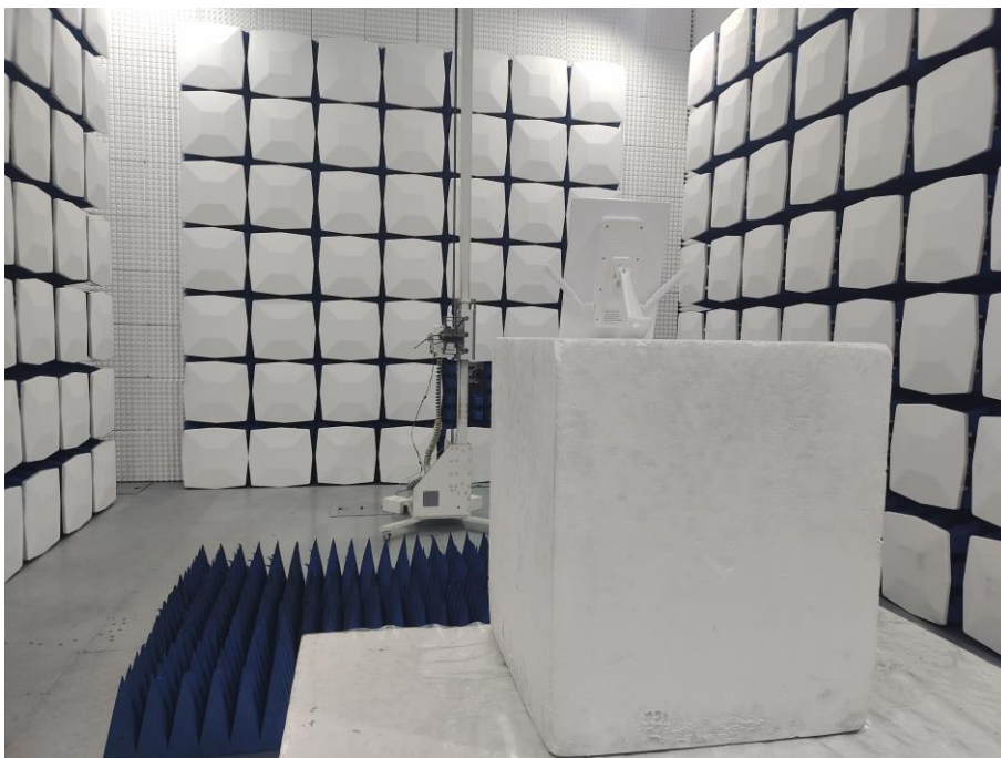
Above 1GHz for WIFI test
