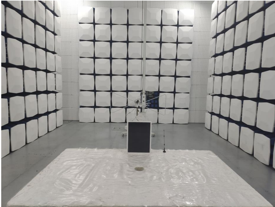
30MHz to 1GHz For LTE test
