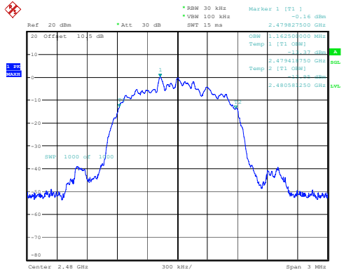
3DH1_High 1.163MHz
