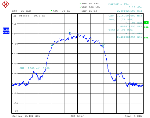
3DH1_Low 1.163MHz
