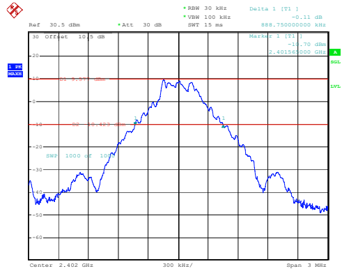
DH1_Low 0.889MHz
