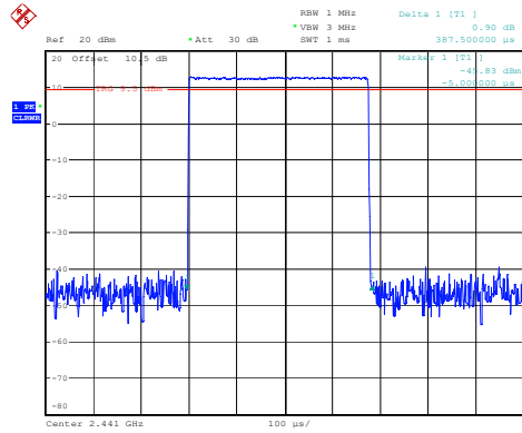
DH1_Hopping 0.388ms
