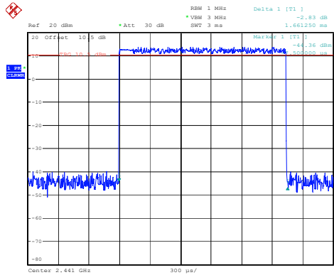
3DH3_Hopping 1.661ms
