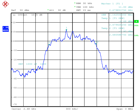
2DH1_High 1.163MHz
