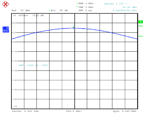
3DH1_Middle 14.34dBm
