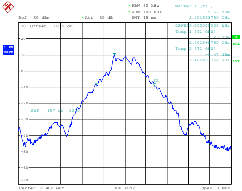
DH1_Low 0.825MHz
