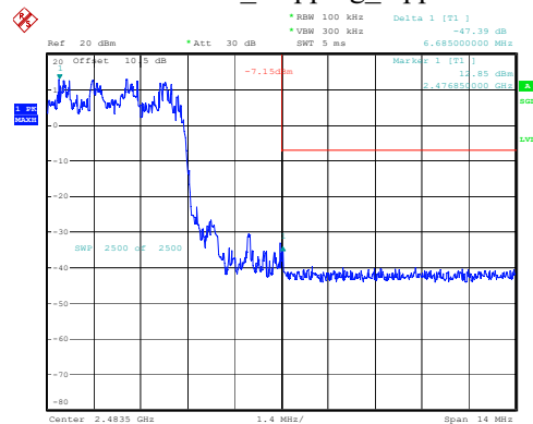
3DH1_Hopping_Upper
