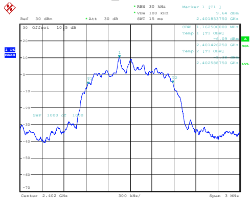
2DH1_Low 1.163MHz
