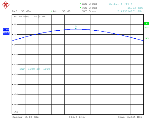
3DH1_High 15.03dBm
