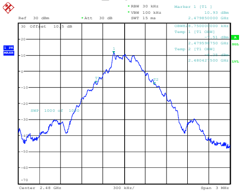
DH1_High 0.829MHz
