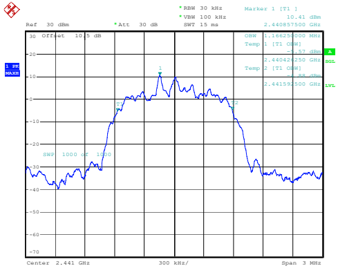
2DH1_Middle 1.166MHz
