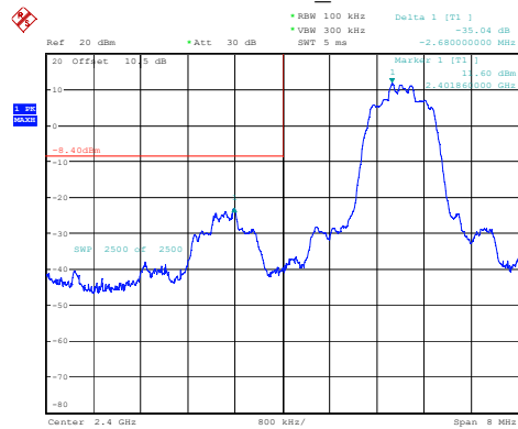
3DH1_Low
