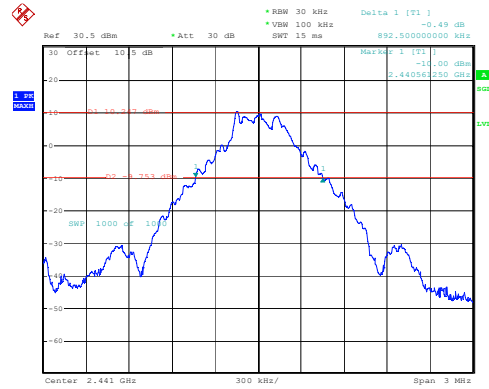
DH1_Middle 0.893MHz
