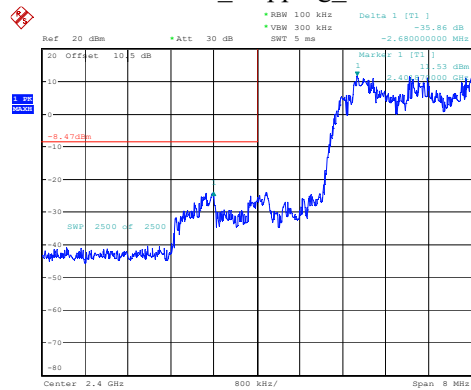
2DH1_Hopping_Lower
