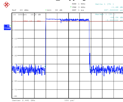
2DH1_Hopping 0.398ms
