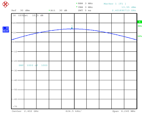
3DH1_Low 13.55dBm
