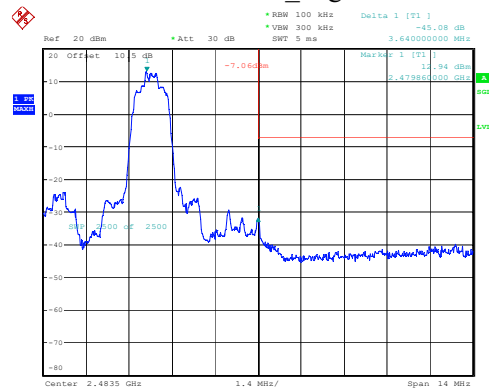
3DH1_High
