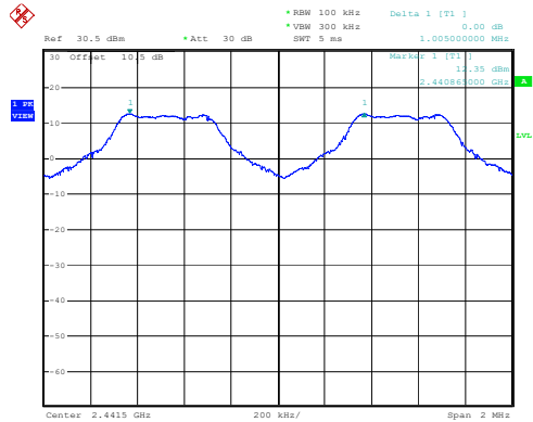
DH1_Middle 1.005MHz
