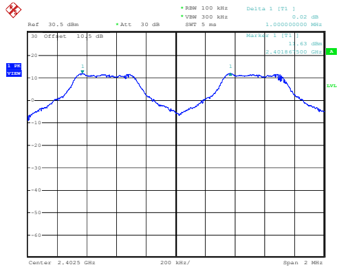
DH1_Low 1.000MHz
