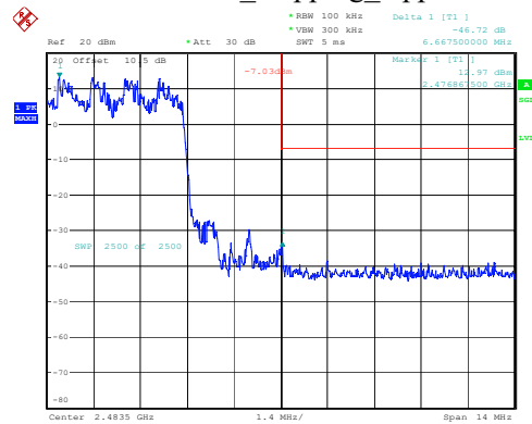
2DH1_Hopping_Upper
