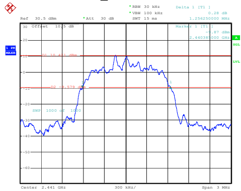
2DH1_Middle 1.256MHz
