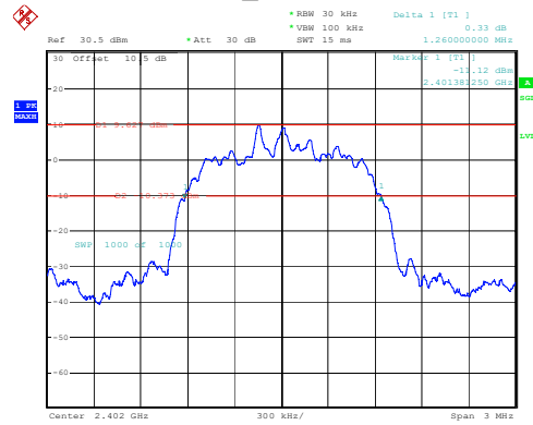
2DH1_Low 1.260MHz
