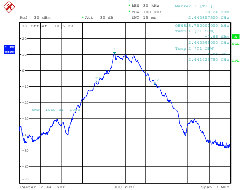
DH1_Middle 0.829MHz
