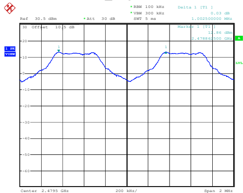
DH1_High 1.003MHz
