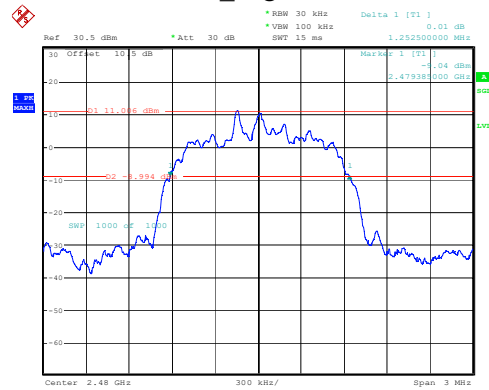
2DH1_High 1.252MHz
