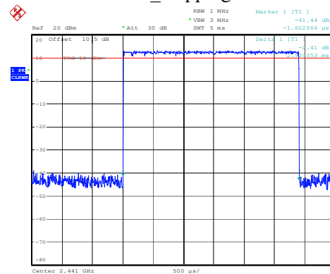
2DH5_Hopping 2.920ms
