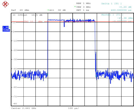
3DH1_Hopping 0.400ms
