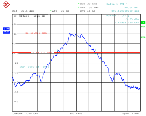
DH1_High 0.893MHz
