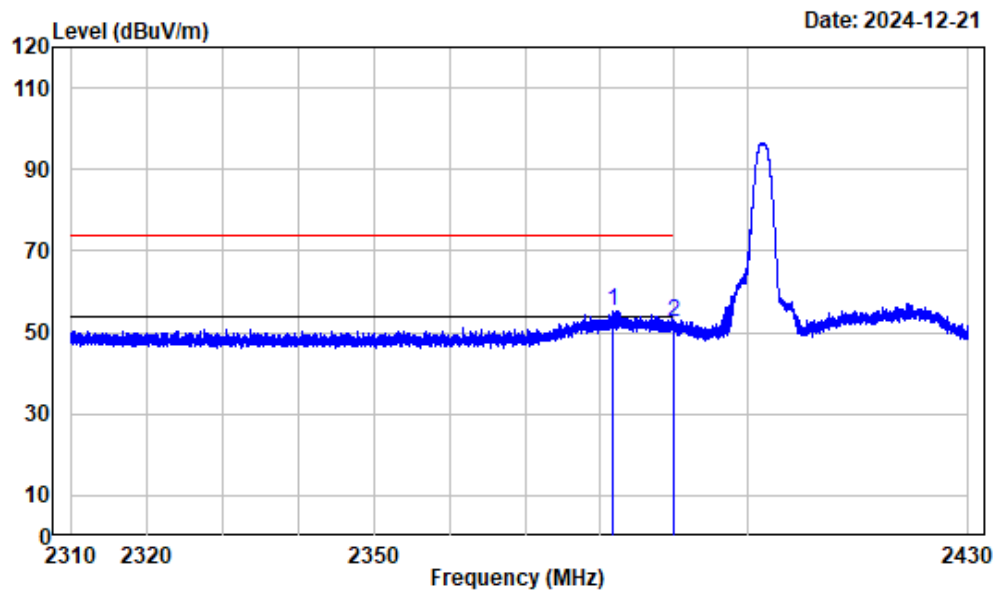
Left Band edge_Horizontal_Peak_BLE 1M
