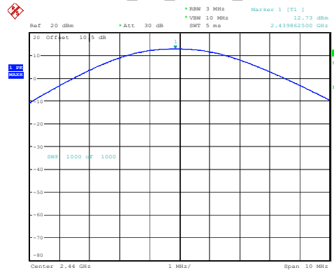
BLE_1M_Middle_Channel
