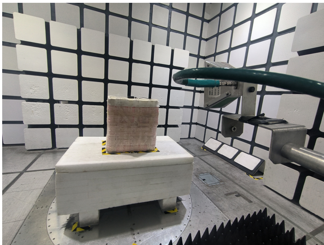
Radiated Emissions View (18-40 GHz)
