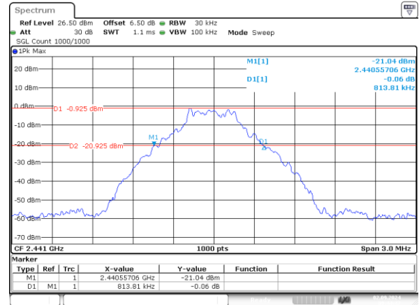
GFSK_Middle 0.814MHz
