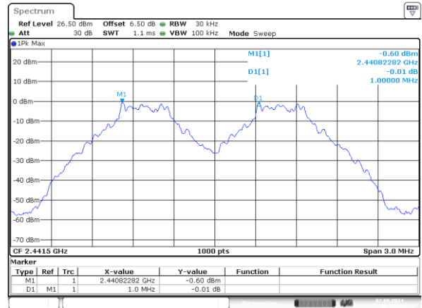
GFSK_Middle 1MHz
