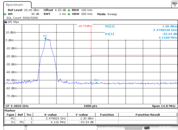
GFSK_High 53.54dB
