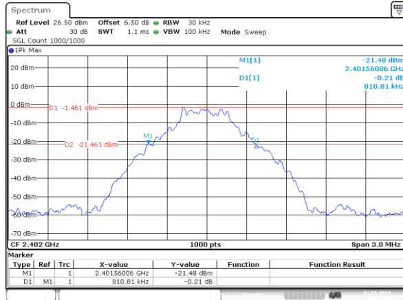
GFSK_Low 0.811MHz
