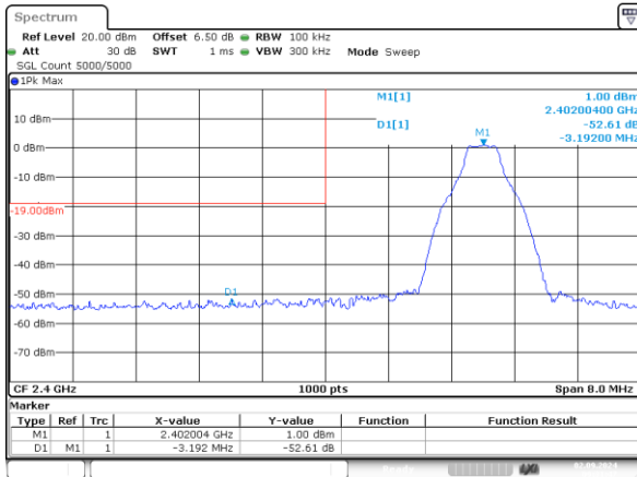
GFSK_Low 52.61dB
