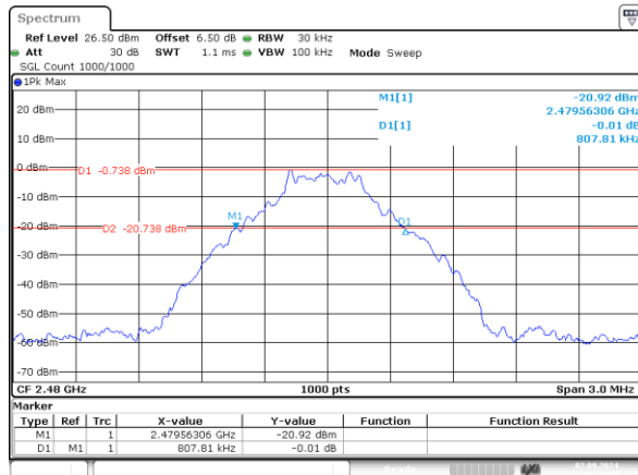
GFSK_High 0.808MHz
