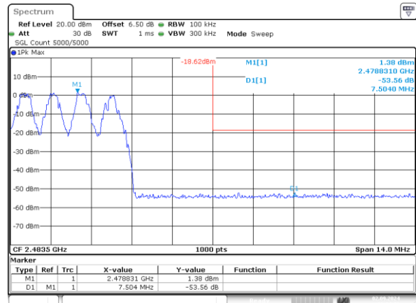
GFSK_Hopping_Upper 53.56dB
