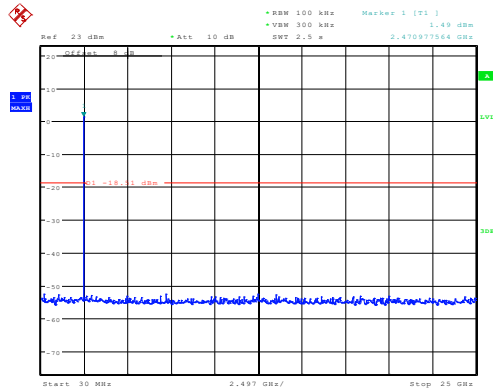
GFSK_High
