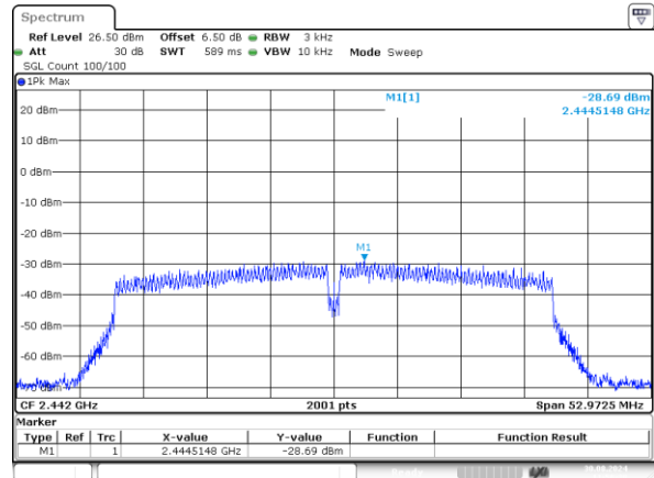
802.11n40_2442MHz_Chain 0 -28.69dBm/3kHz
