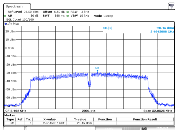
802.11n40_2462MHz_Chain 1 -28.45dBm/3kHz
