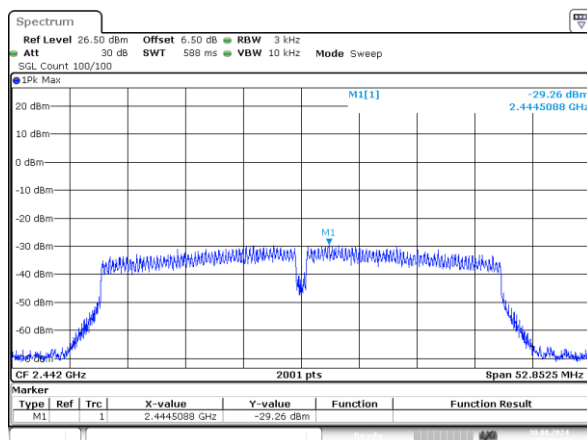
802.11n40_2442MHz_Chain 1 -29.26dBm/3kHz
