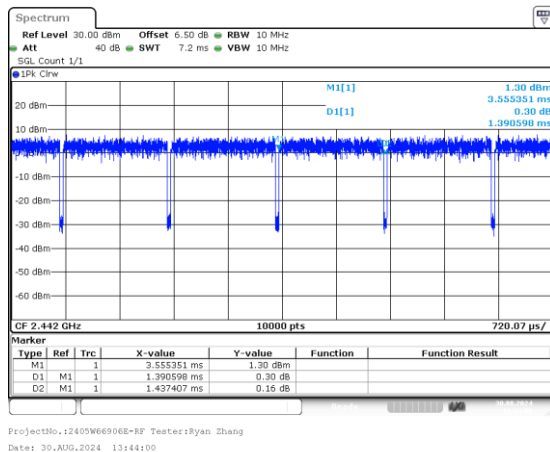
802.11g_2442MHz_Chain 1 1.391ms,1.437ms
