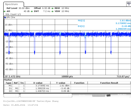
802.11g_2472MHz_Chain 1 1.390ms,1.437ms
