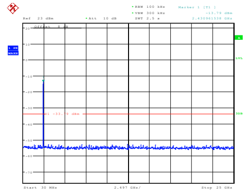
802.11n40_2442MHz_Chain 0
