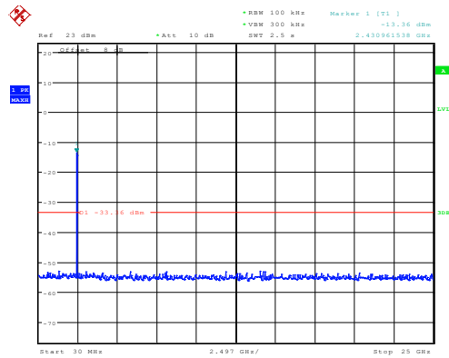
802.11n40_2462MHz_Chain 0
