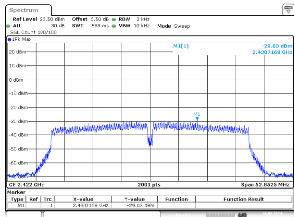
802.11n40_2422MHz_Chain 1 -29.03dBm/3kHz
