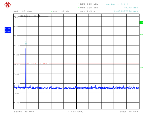
802.11g_2472MHz_Chain 1
