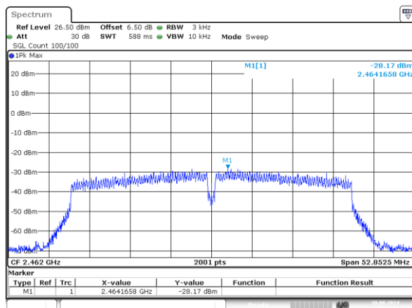
802.11n40_2462MHz_Chain 0 -28.17dBm/3kHz
