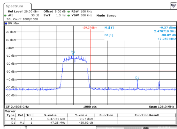
802.11n20_2472MHz_Chain 0
