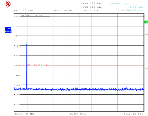
802.11g_2442MHz_Chain 0
