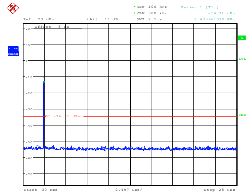
802.11n40_2422MHz_Chain 1
