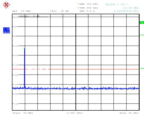
802.11n40_2422MHz_Chain 0
