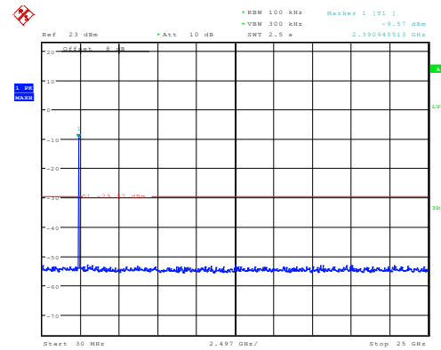
802.11g_2412MHz_Chain 1
