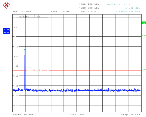
802.11n40_2442MHz_Chain 1
