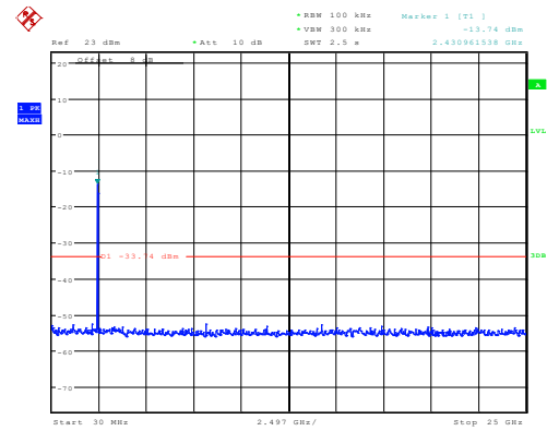
802.11n40_2462MHz_Chain 1
