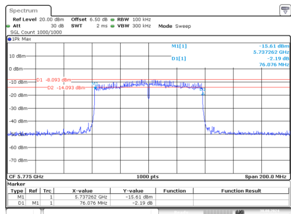
ac80_5775MHz_Chain 1 76.076MHz
