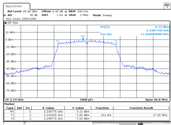
n20_5240MHz_Chain 1 17.550MHz
