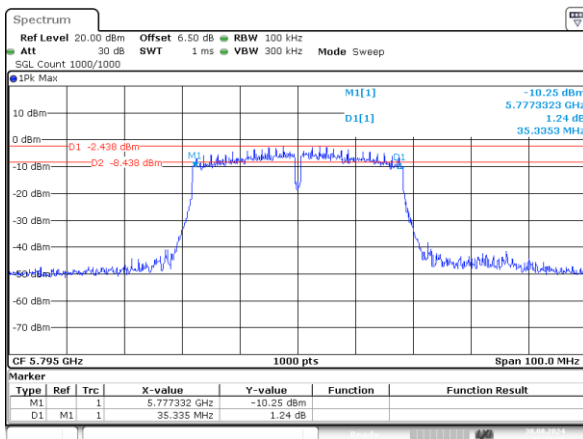
n40_5795MHz_Chain 0 35.335MHz
