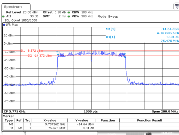
ac80_5775MHz_Chain 0 75.475MHz
