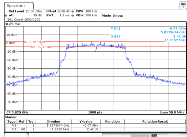
a_5825MHz_Chain 1 15.215MHz
