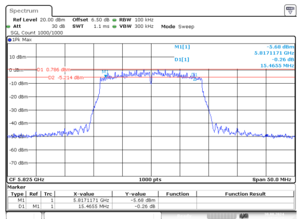
n20_5825MHz_Chain 1 15.465MHz
