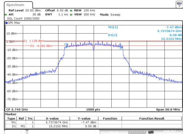
a_5745MHz_Chain 1 15.215MHz
