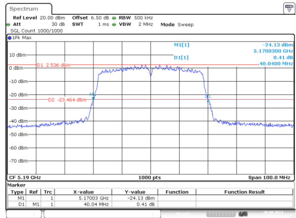
n40_5190MHz_Chain 1 40.040MHz
