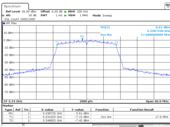
n20_5240MHz_Chain 0 17.600MHz
