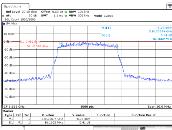
n20_5825MHz_Chain 0 16.166MHz
