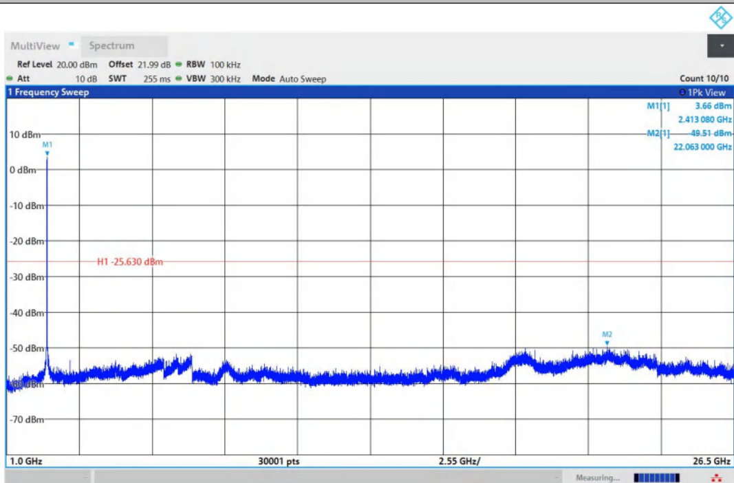
11G-Ant2-2412-1000~26500-PASS
