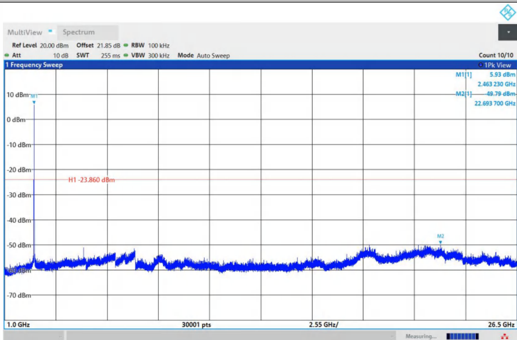
11B-Ant2-2462-1000~26500-PASS
