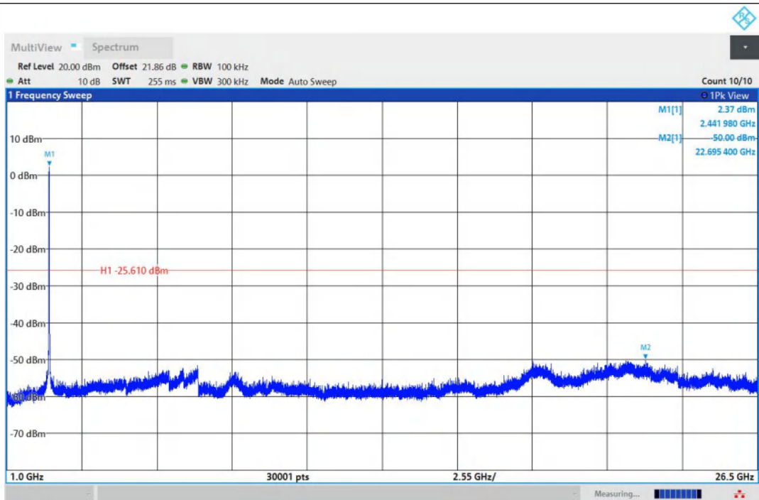
11G-Ant1-2437-1000~26500-PASS
