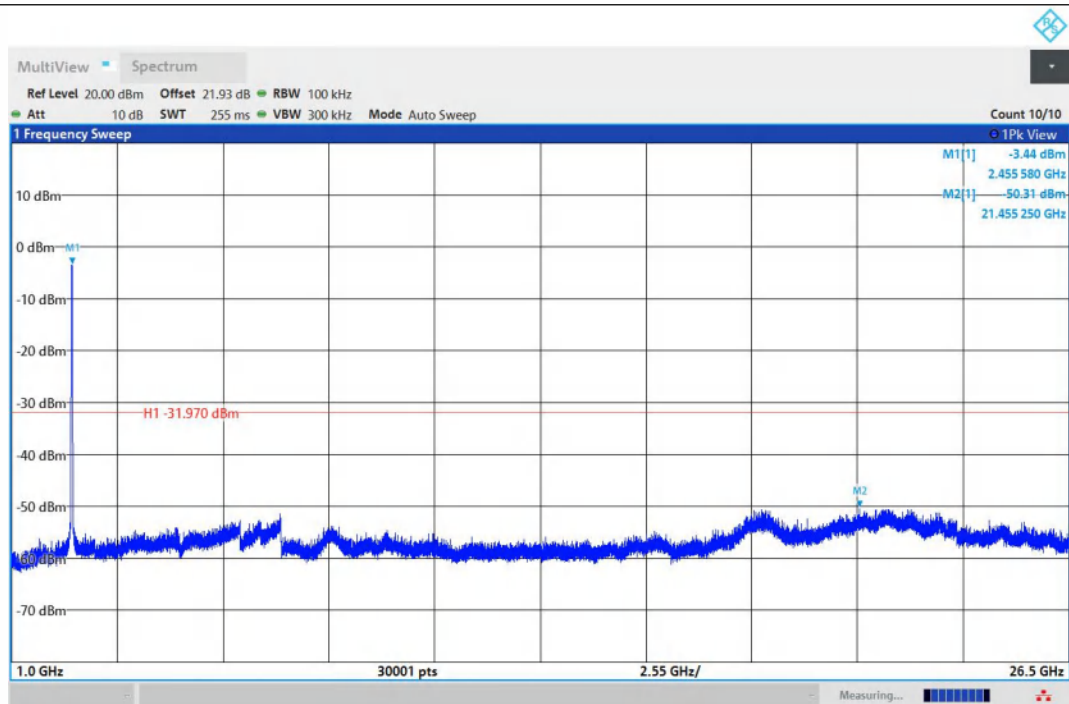
11N40MIMO-Ant1-2452-1000~26500-PASS
