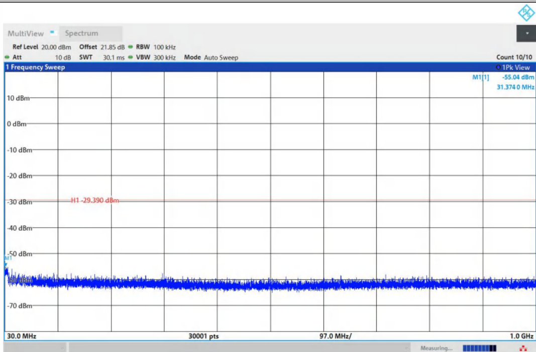
11N20MIMO-Ant2-2462-30~1000-PASS
