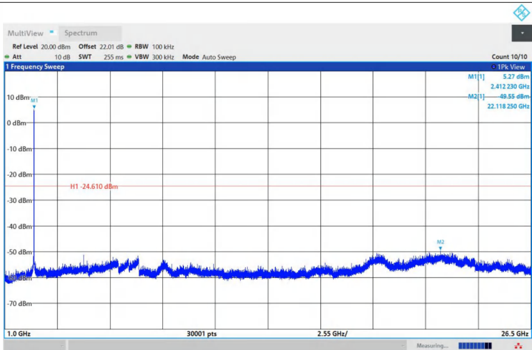
11B-Ant1-2412-1000~26500-PASS
