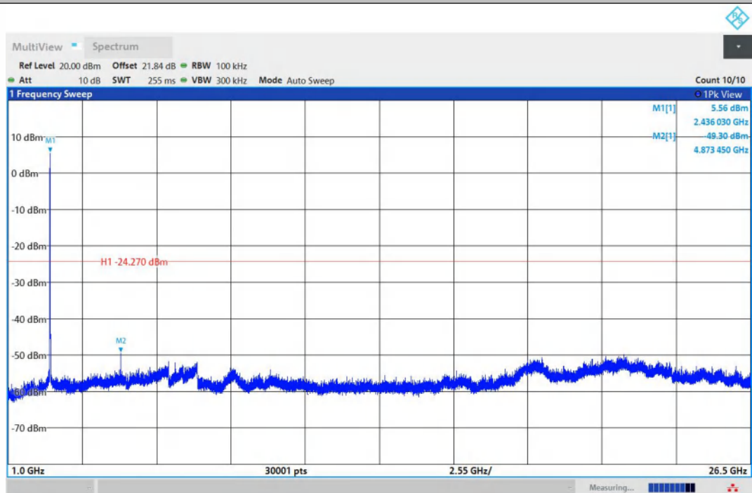
11B-Ant2-2437-1000~26500-PASS
