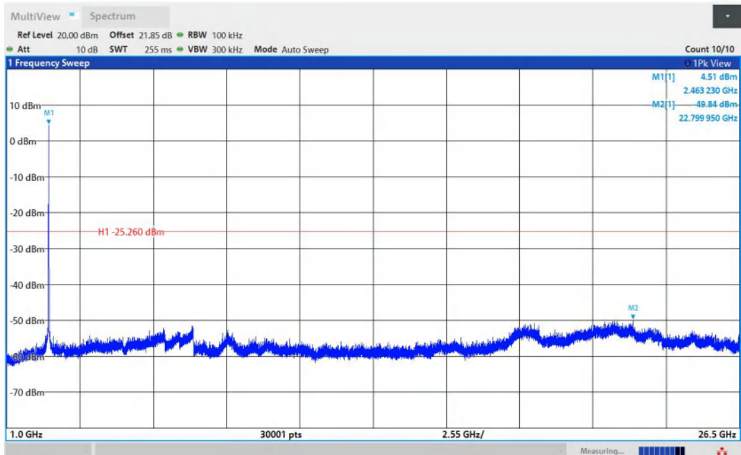
11G-Ant2-2462-1000~26500-PASS
