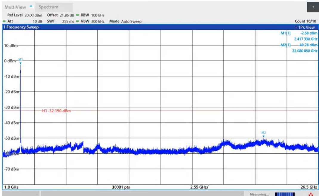
11N40MIMO-Ant2-2422-1000~26500-PASS
