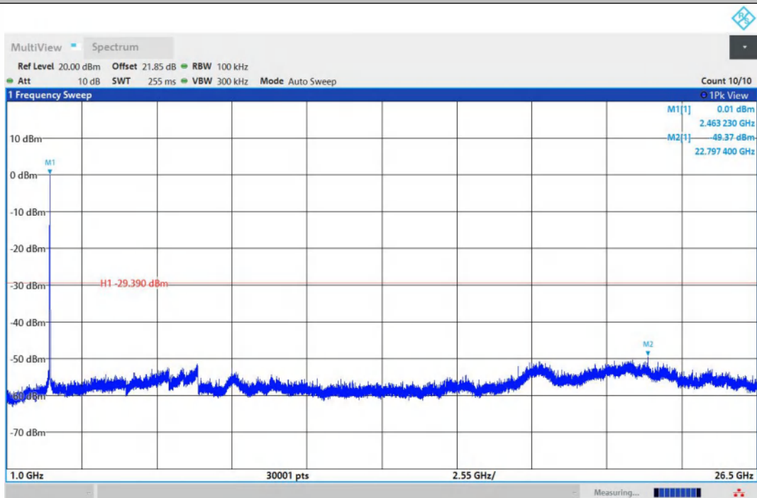
11N20MIMO-Ant2-2462-1000~26500-PASS
