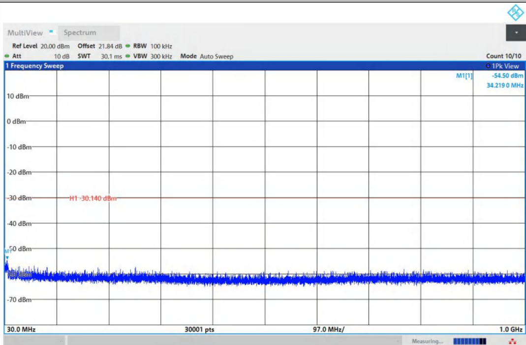
11N20MIMO-Ant2-2437-30~1000-PASS
