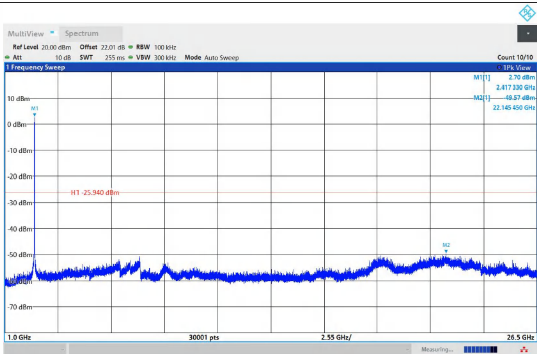
11G-Ant1-2412-1000~26500-PASS
