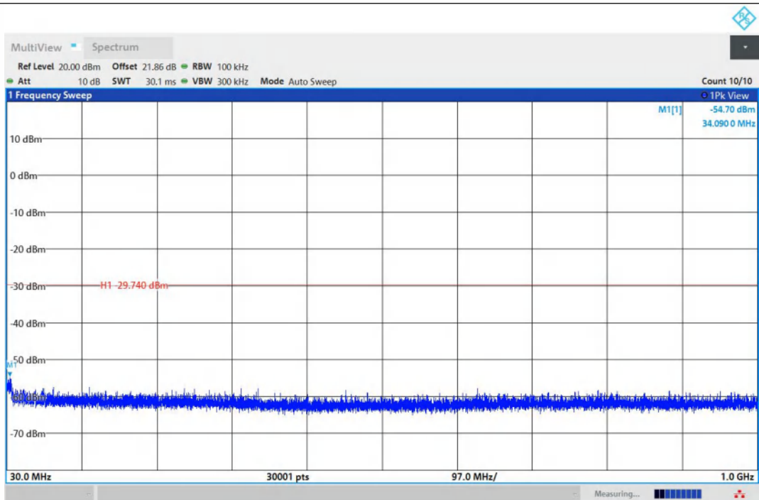
11N20MIMO-Ant1-2437-30~1000-PASS
