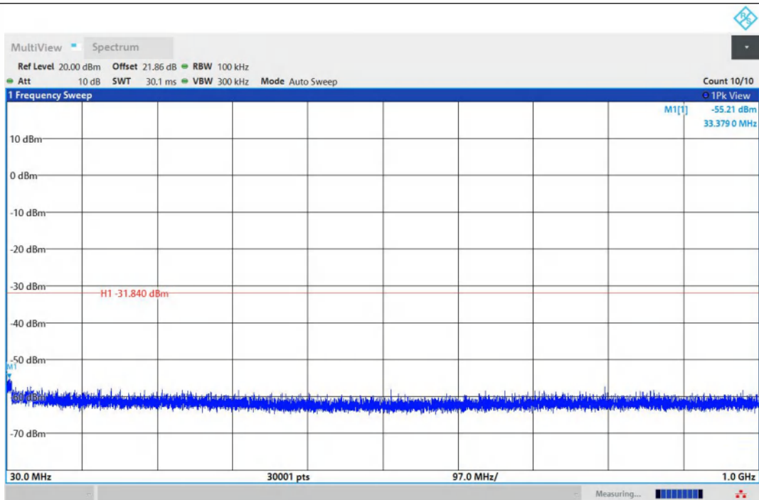
11N40MIMO-Ant1-2437-30~1000-PASS
