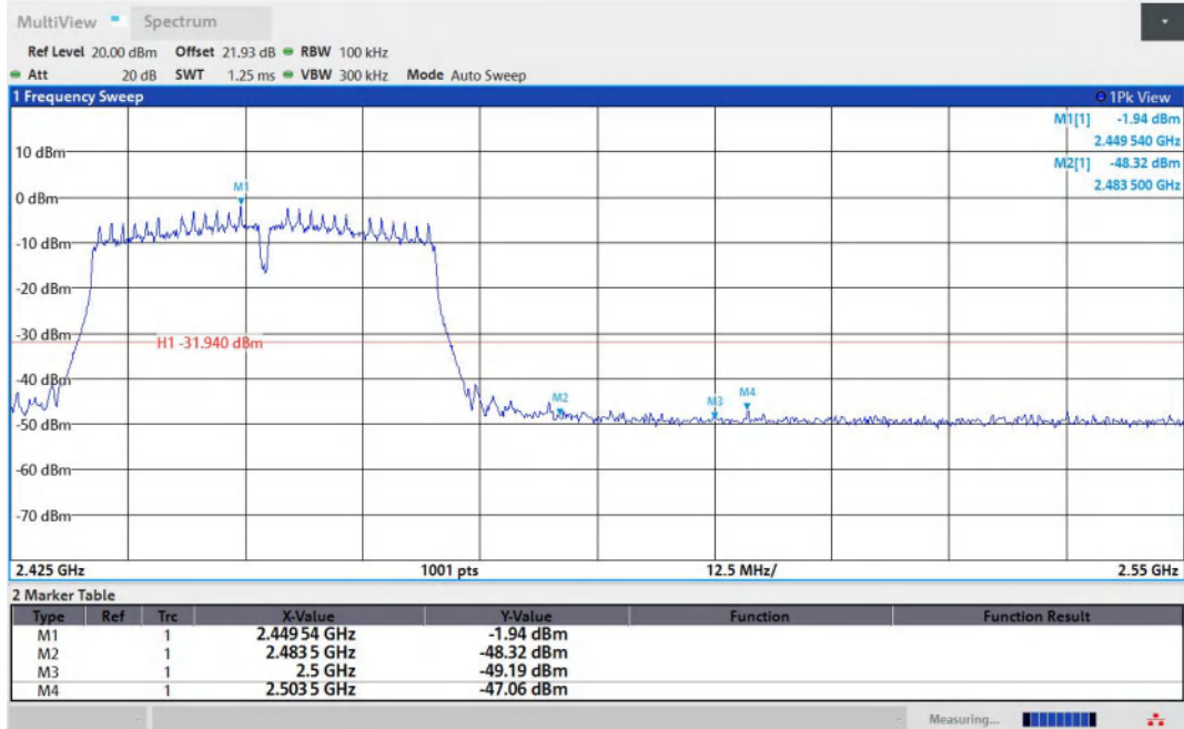
11N40MIMO-Ant1-2452-PASS
