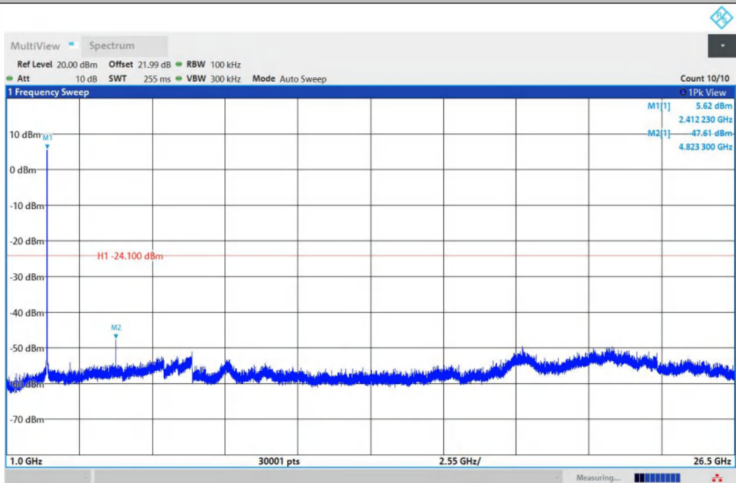
11B-Ant2-2412-1000~26500-PASS
