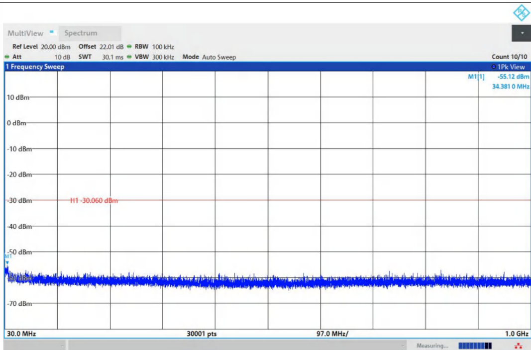
11N20MIMO-Ant1-2412-30~1000-PASS
