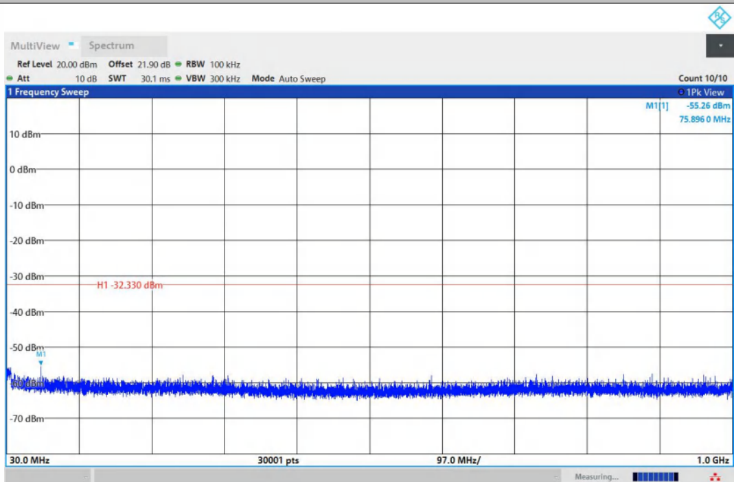
11N40MIMO-Ant2-2452-30~1000-PASS
