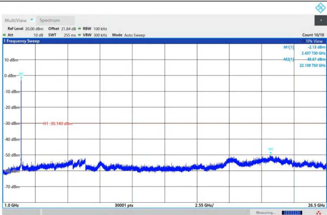
11N20MIMO-Ant2-2437-1000~26500-PASS
