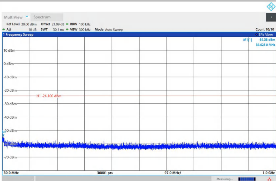
11B-Ant2-2412-30~1000-PASS
