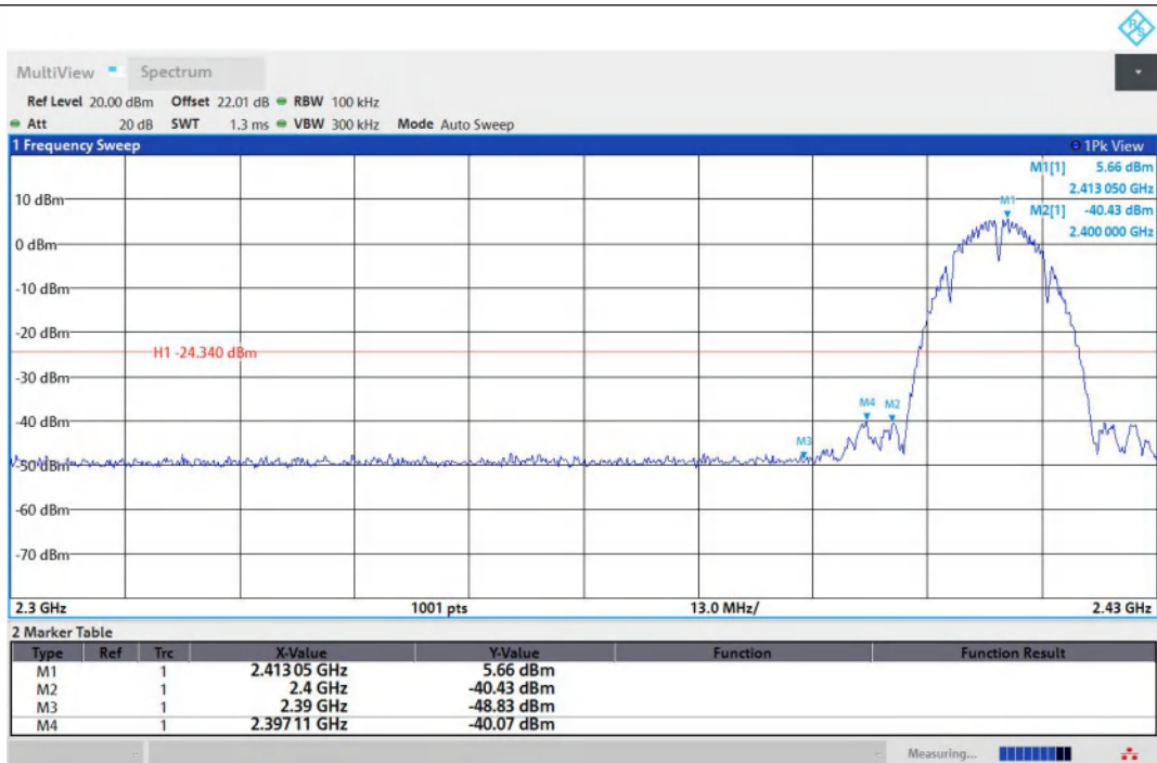
11B-Ant1-2412-PASS
