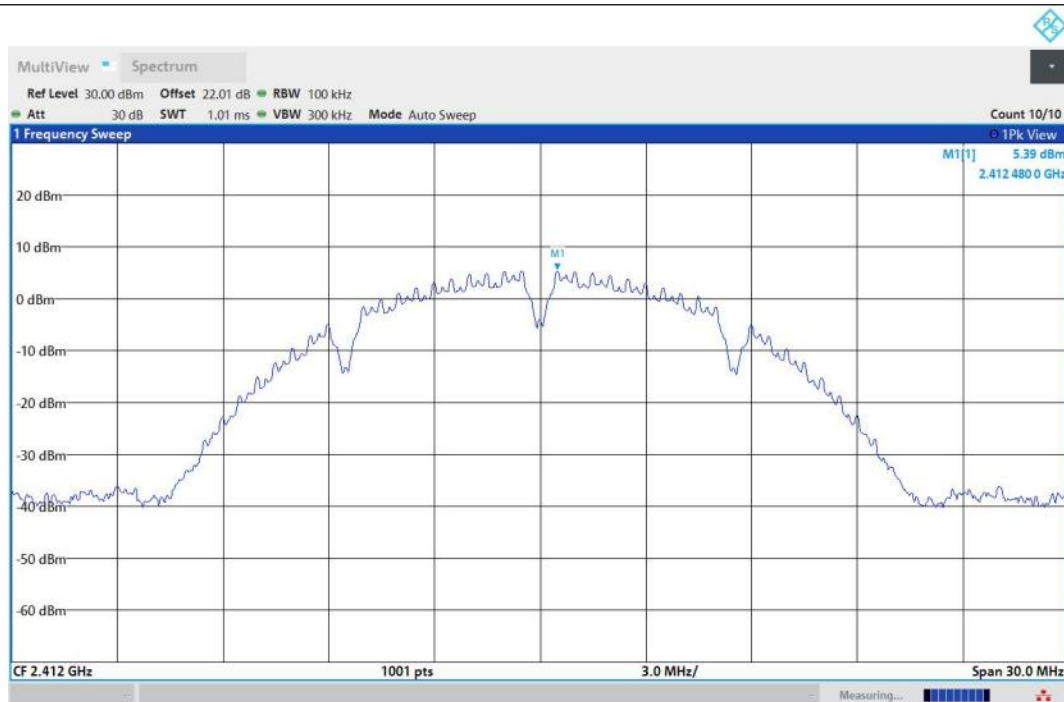
11B-Ant1-2412-0~Reference-PASS
