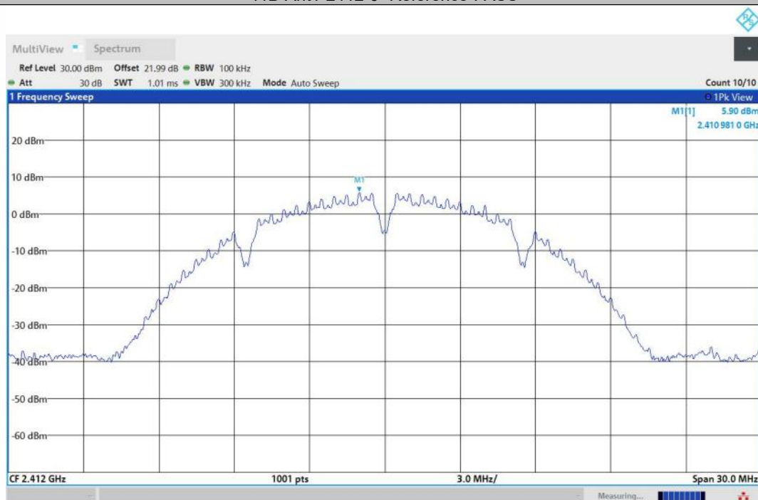
11B-Ant2-2412-0~Reference-PASS
