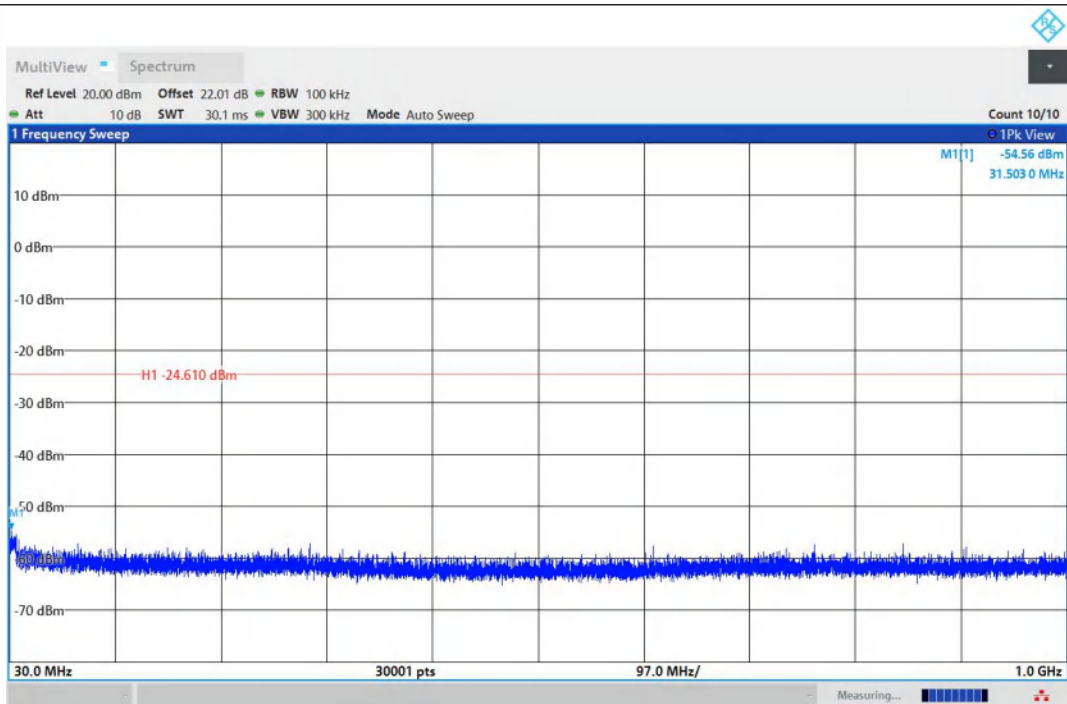
11B-Ant1-2412-30~1000-PASS
