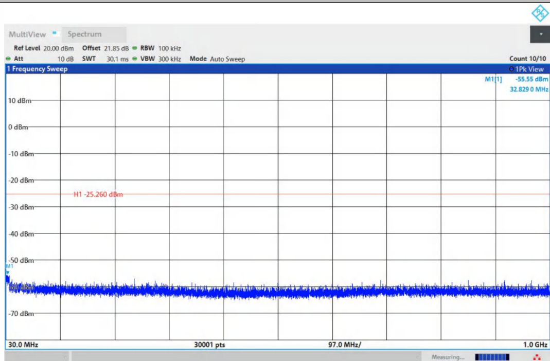
11G-Ant2-2462-30~1000-PASS
