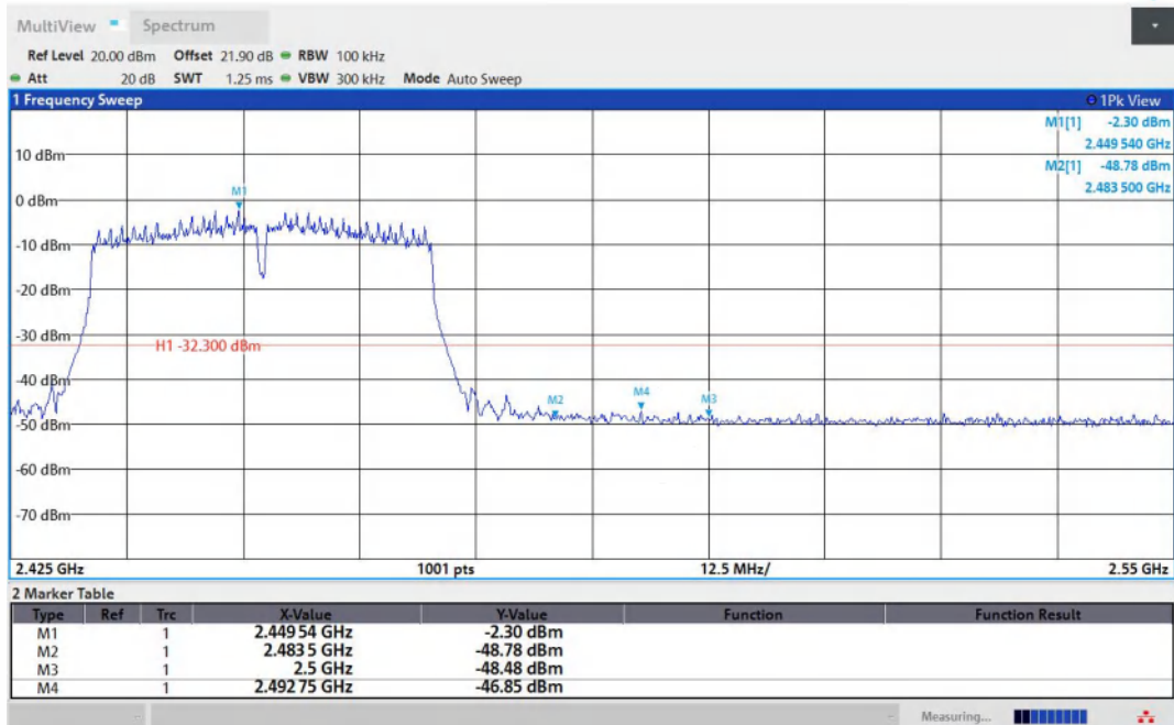
11N40MIMO-Ant2-2452-PASS
