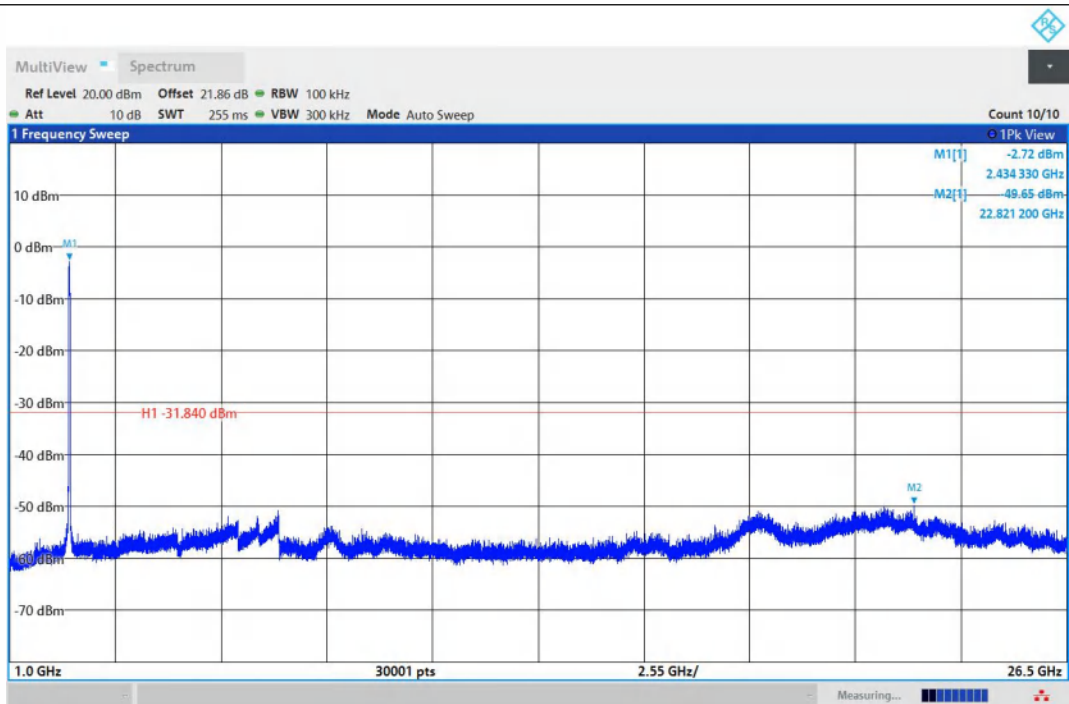
11N40MIMO-Ant1-2437-1000~26500-PASS
