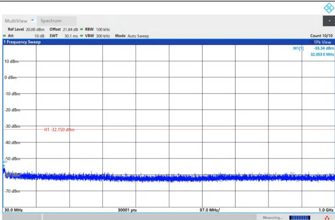
11N40MIMO-Ant2-2437-30~1000-PASS
