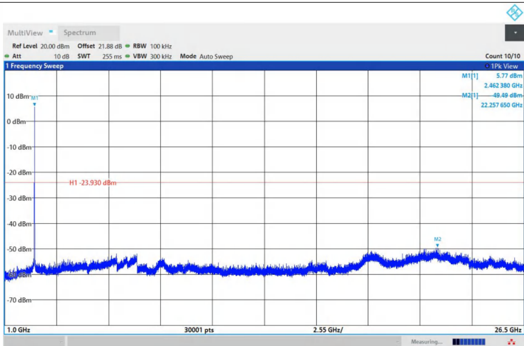
11B-Ant1-2462-1000~26500-PASS
