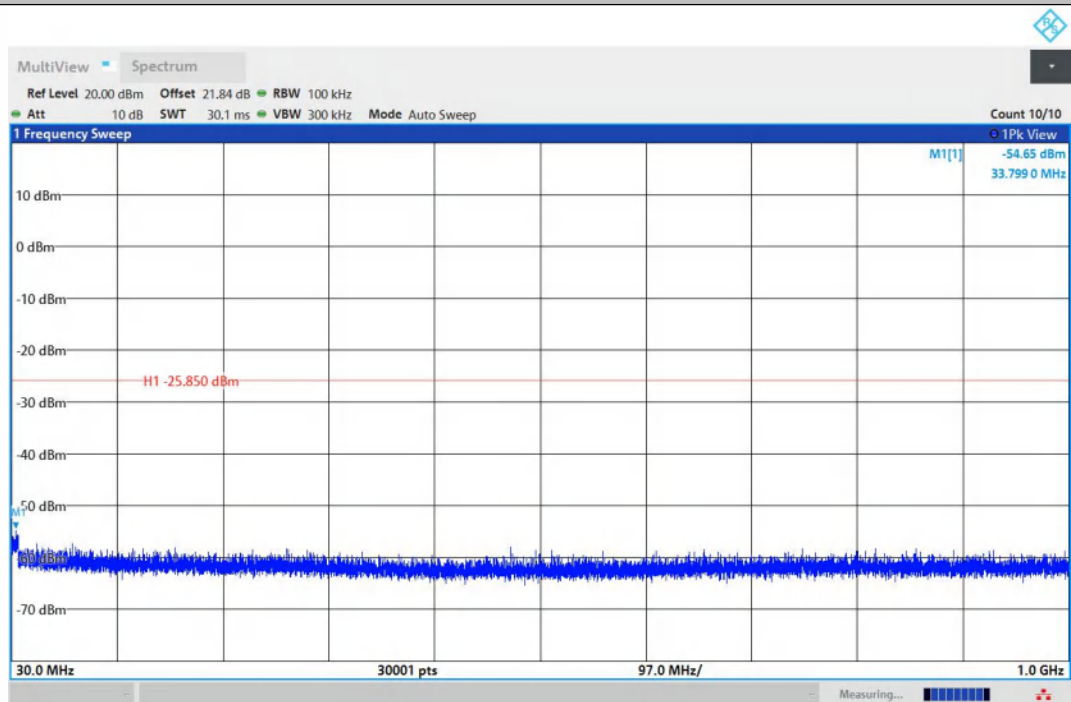
11G-Ant2-2437-30~1000-PASS
