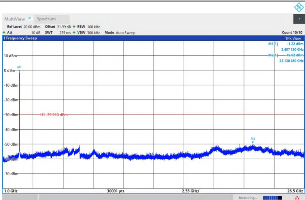
11N20MIMO-Ant2-2412-1000~26500-PASS
