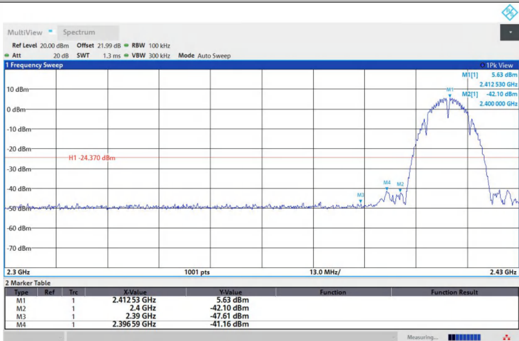
11B-Ant2-2412-PASS
