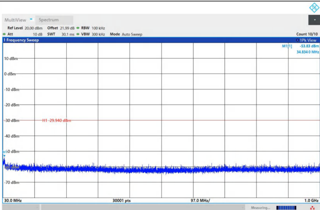
11N20MIMO-Ant2-2412-30~1000-PASS
