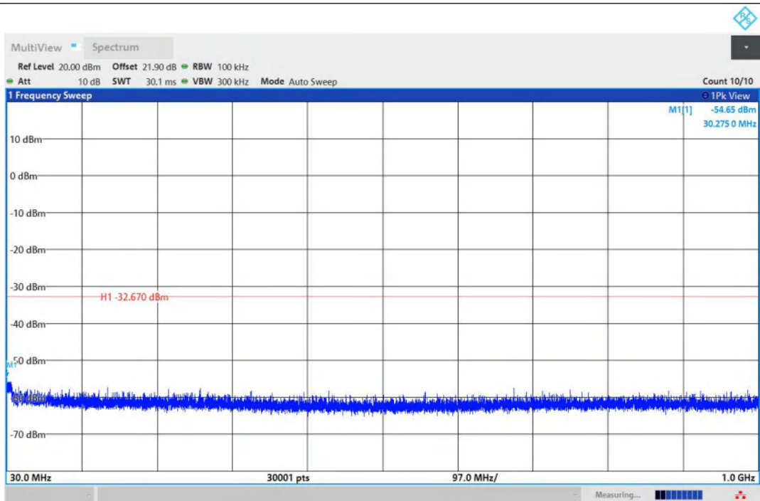
11N40MIMO-Ant1-2422-30~1000-PASS
