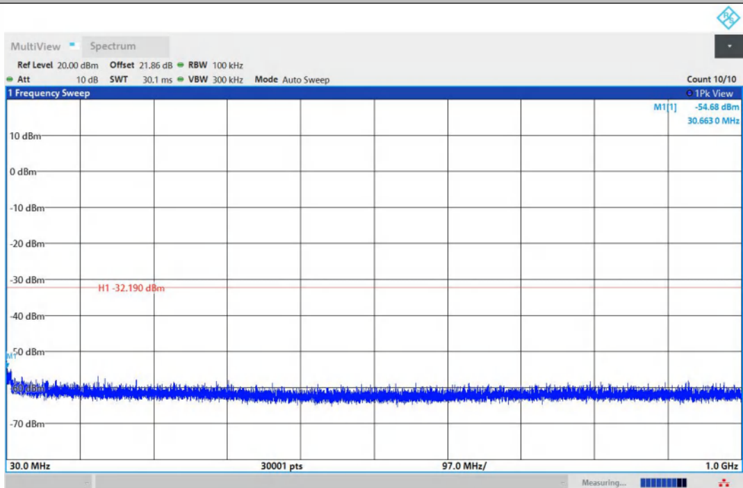
11N40MIMO-Ant2-2422-30~1000-PASS
