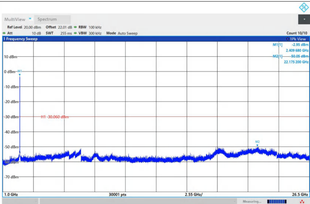
11N20MIMO-Ant1-2412-1000~26500-PASS
