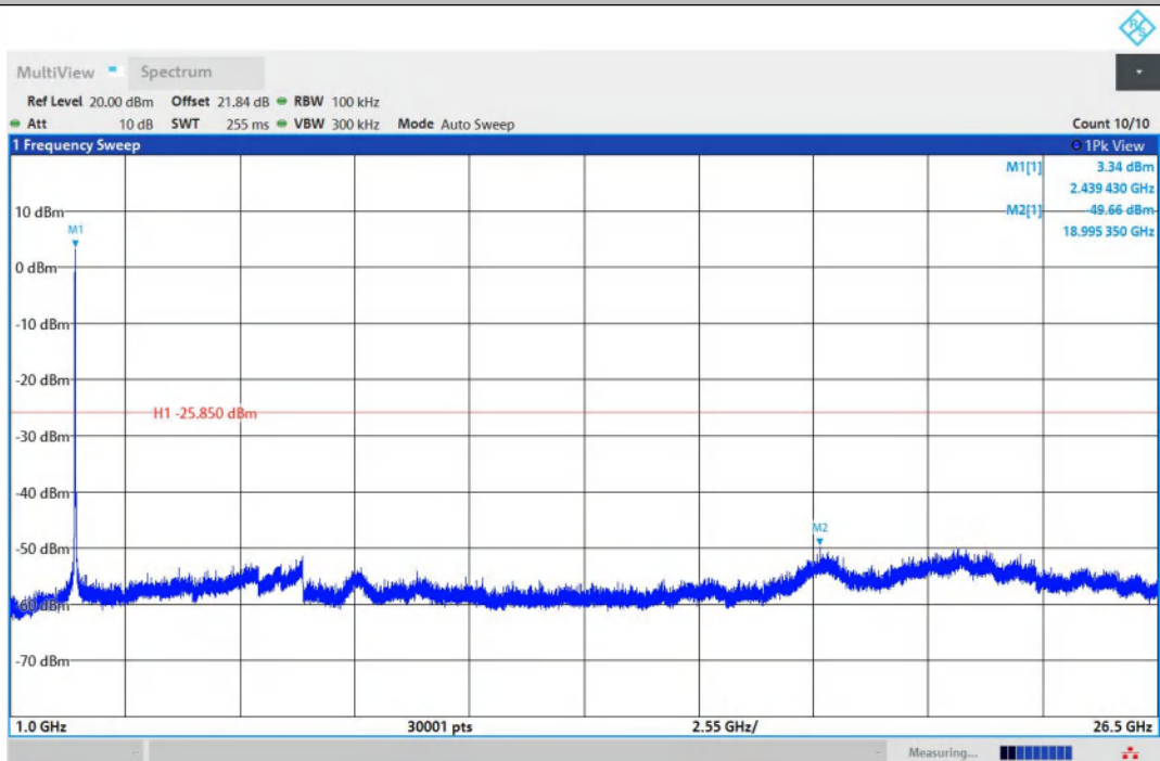
11G-Ant2-2437-1000~26500-PASS
