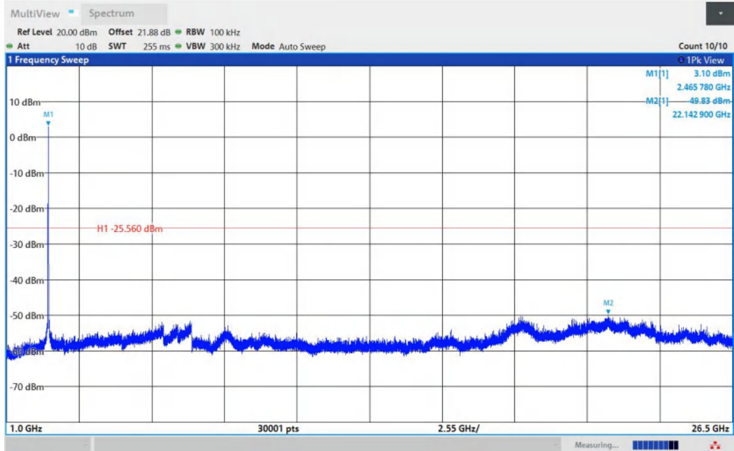
11G-Ant1-2462-1000~26500-PASS
