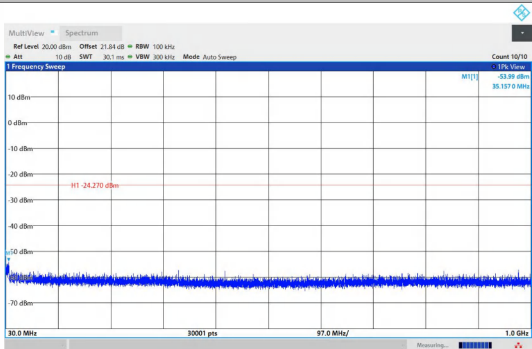
11B-Ant2-2437-30~1000-PASS
