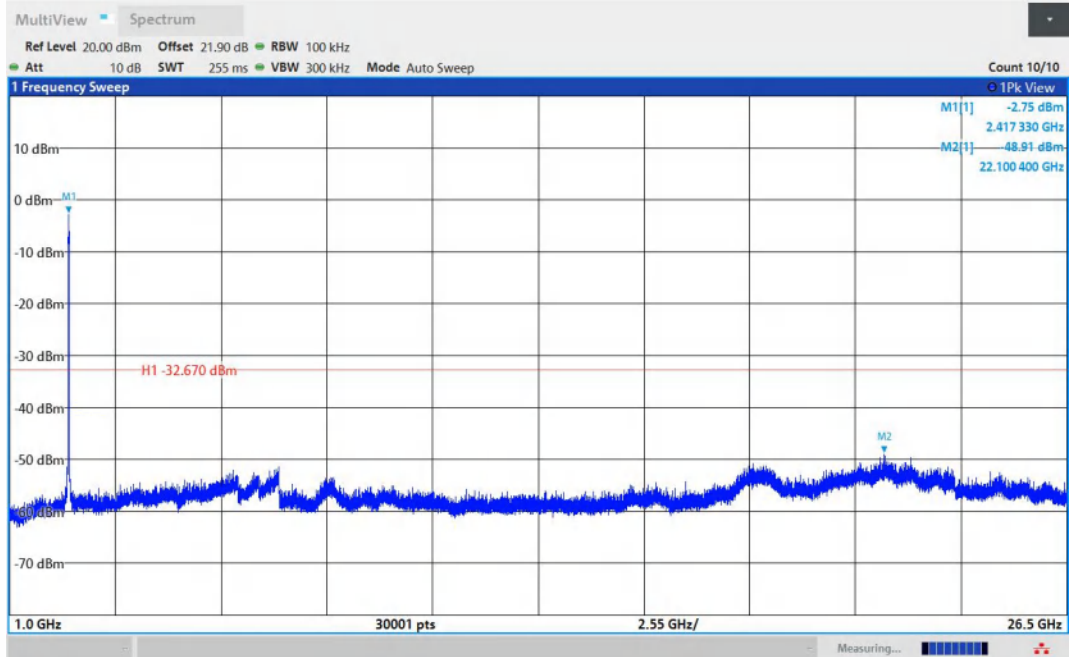
11N40MIMO-Ant1-2422-1000~26500-PASS
