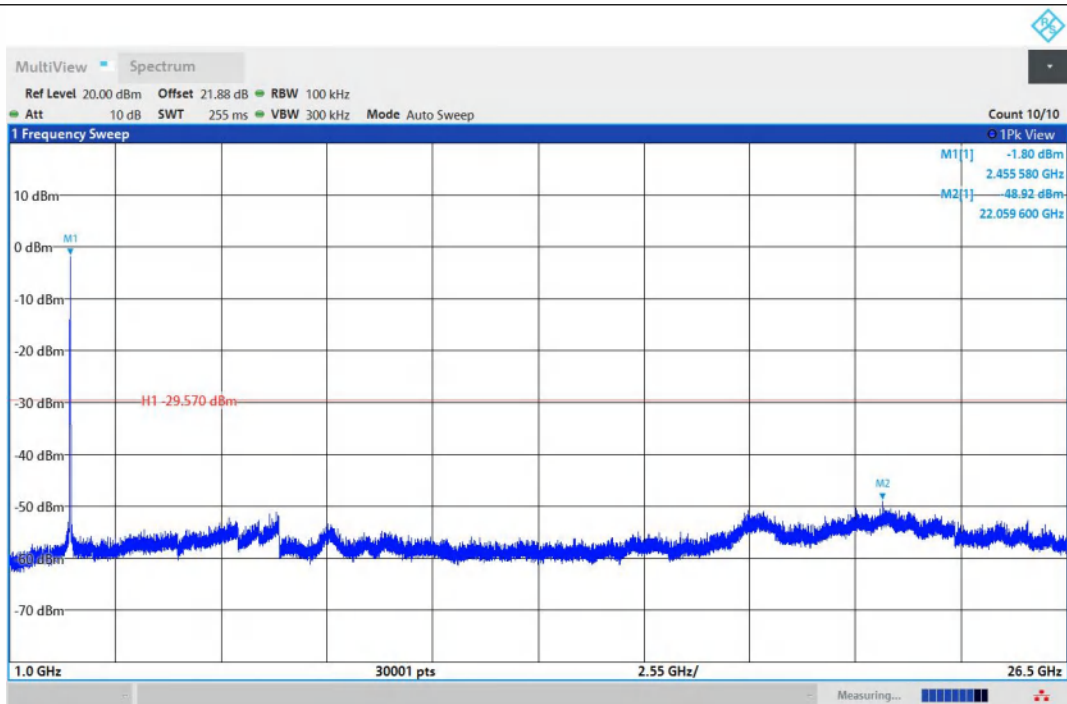
11N20MIMO-Ant1-2462-1000~26500-PASS
