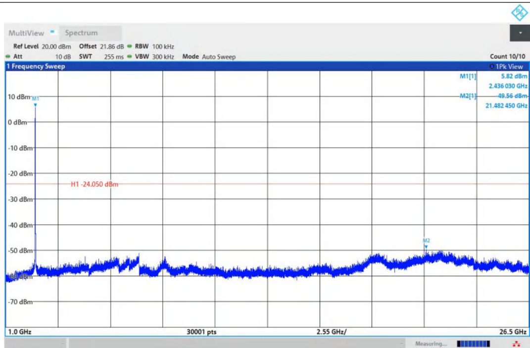
11B-Ant1-2437-1000~26500-PASS
