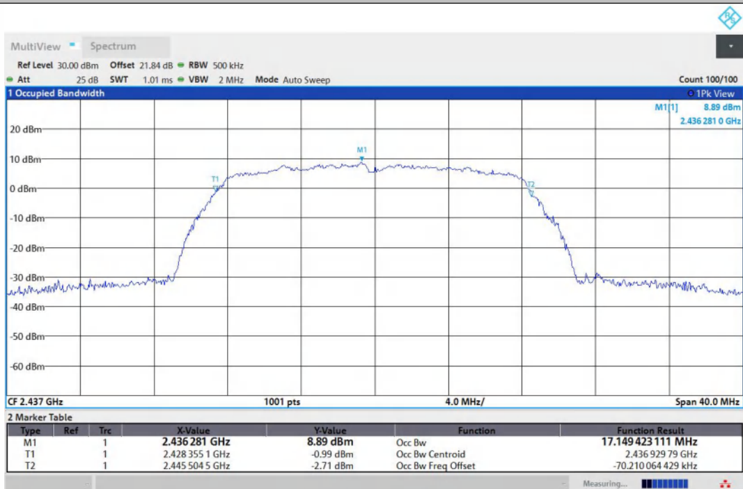
11G-Ant2-2437
