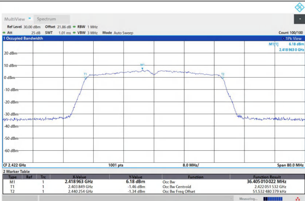
11N40MIMO-Ant2-2422
