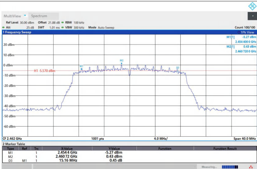
11N20MIMO-Ant1-2462-PASS
