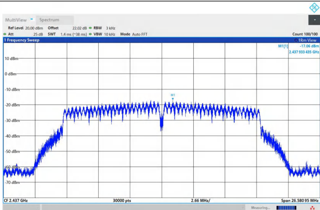
11G-Ant2-2437-PASS
