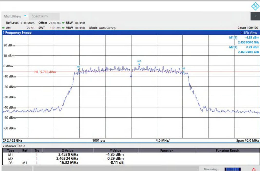
11N20MIMO-Ant2-2462-PASS
