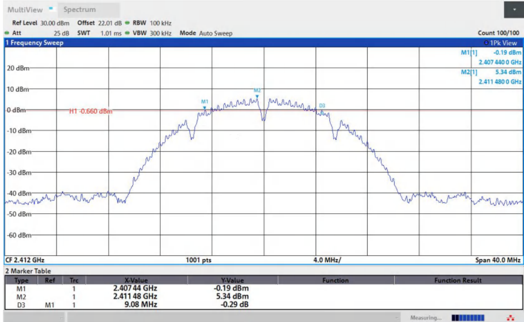
11B-Ant1-2412-PASS
