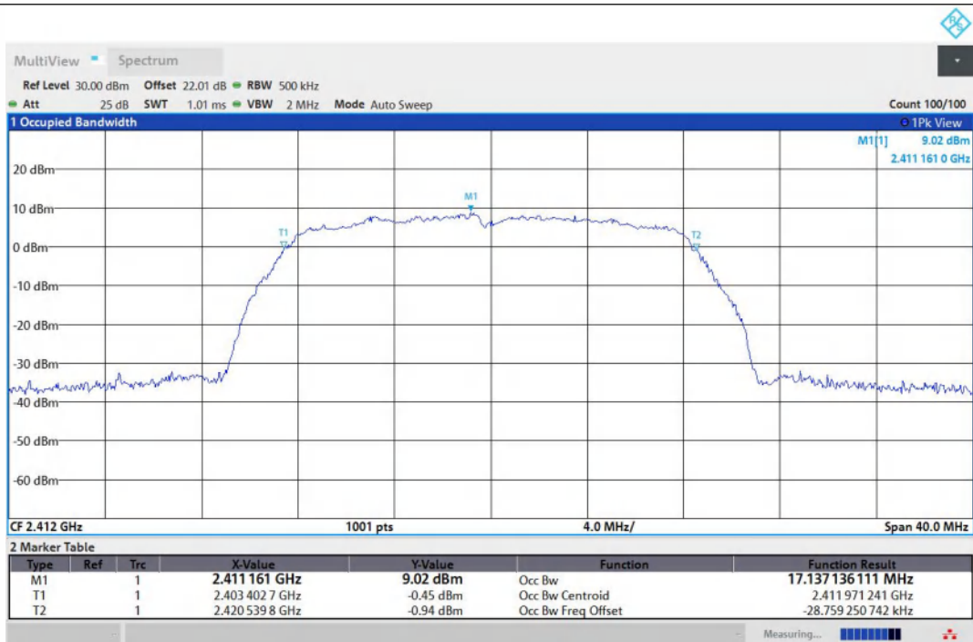
11G-Ant1-2412
