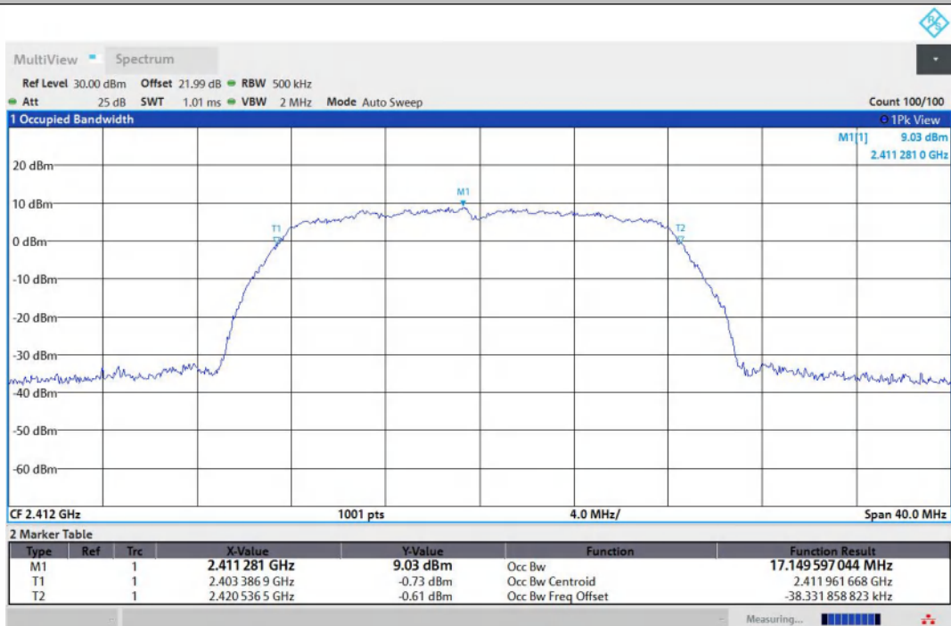
11G-Ant2-2412
