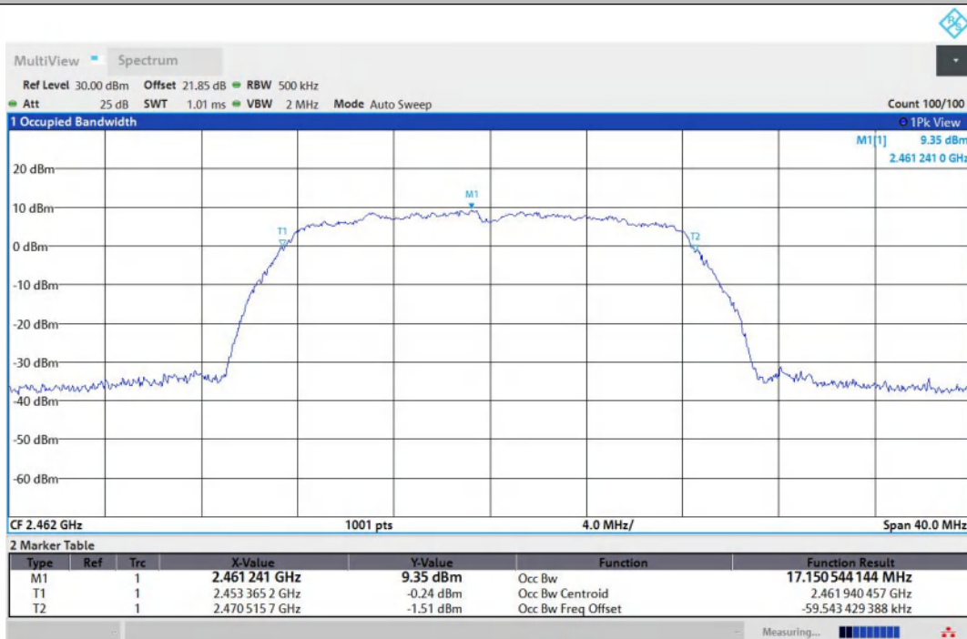
11G-Ant2-2462
