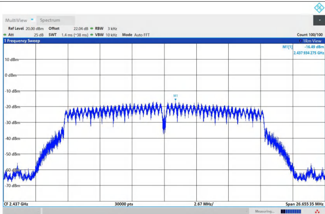
11G-Ant1-2437-PASS
