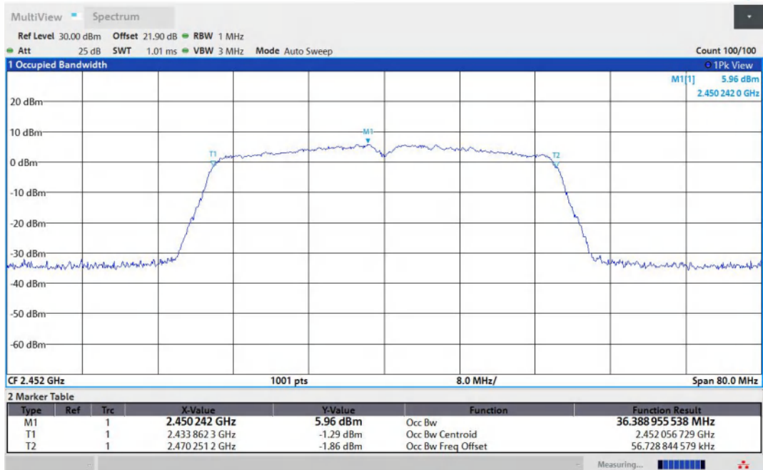
11N40MIMO-Ant2-2452
