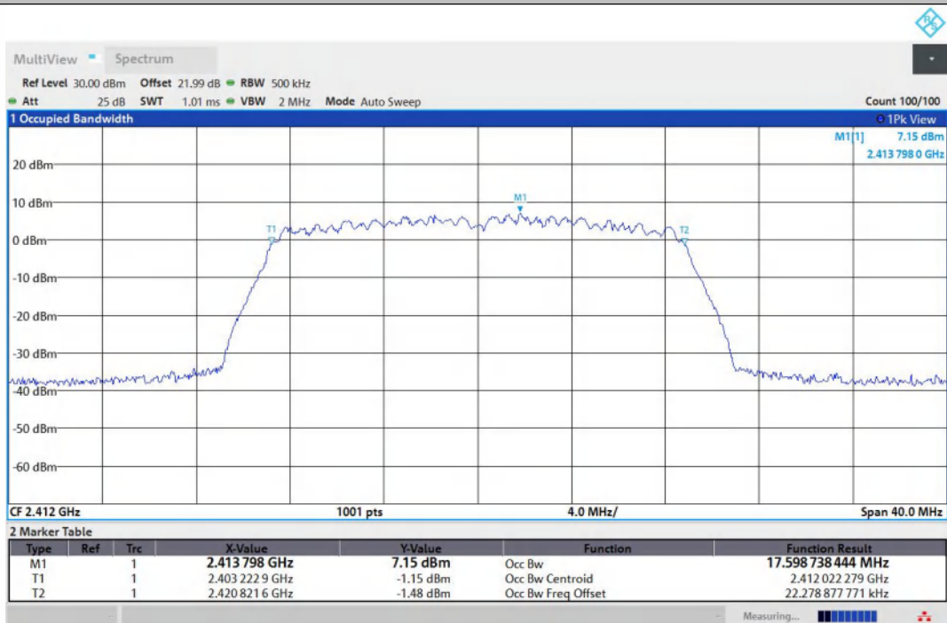
11N20MIMO-Ant2-2412
