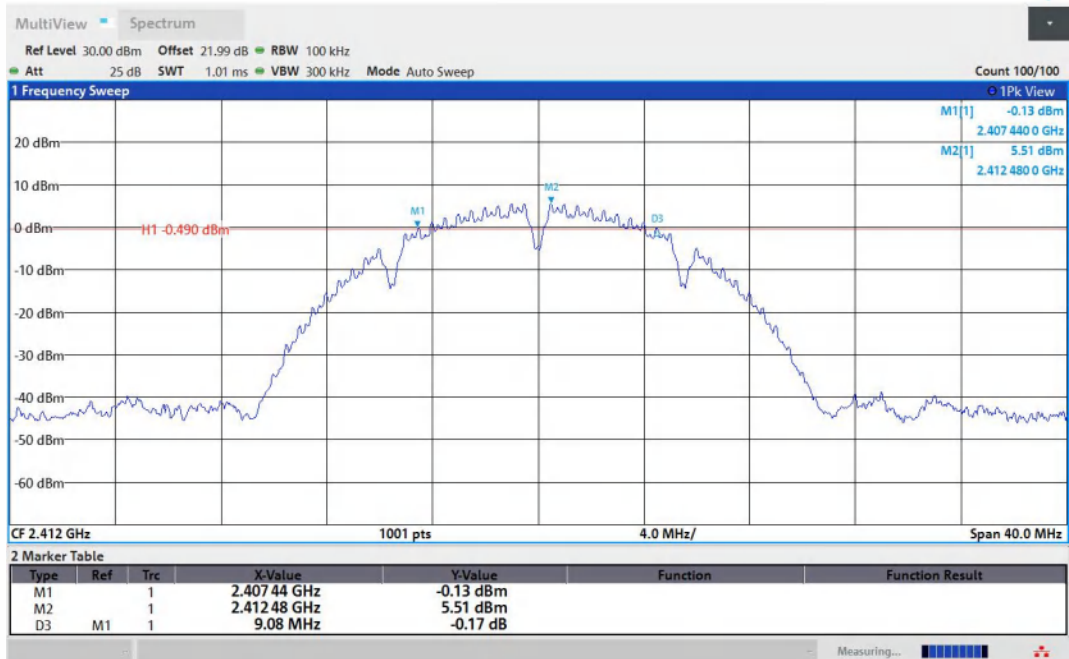
11B-Ant2-2412-PASS
