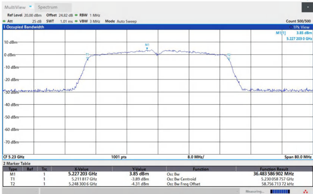
11AC40MIMO-Ant2-5230
