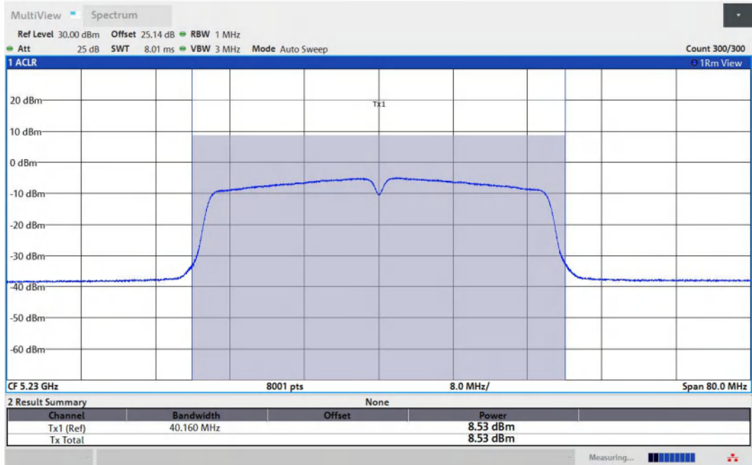
11AC40MIMO-Ant2-5230-PASS
