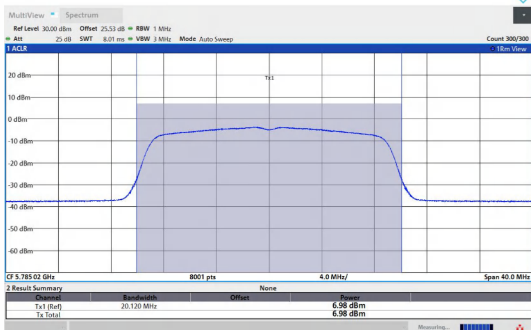
11AC20MIMO-Ant1-5785-PASS
