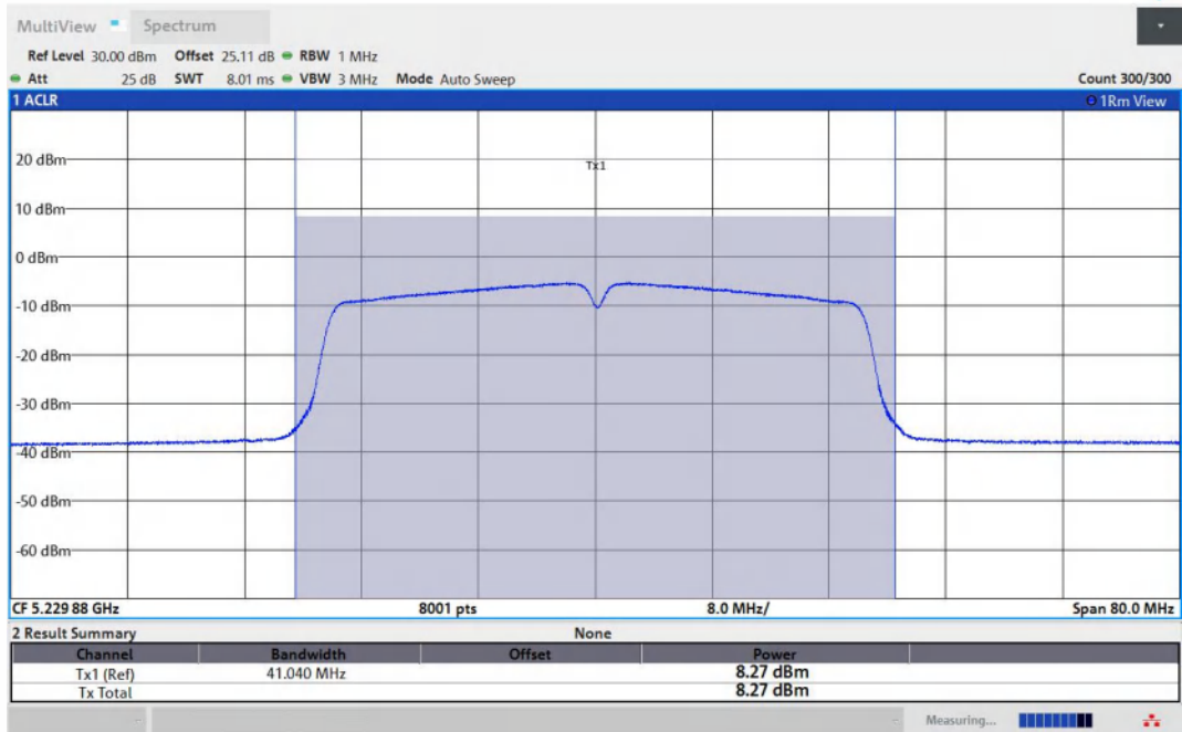
11AC40MIMO-Ant1-5230-PASS
