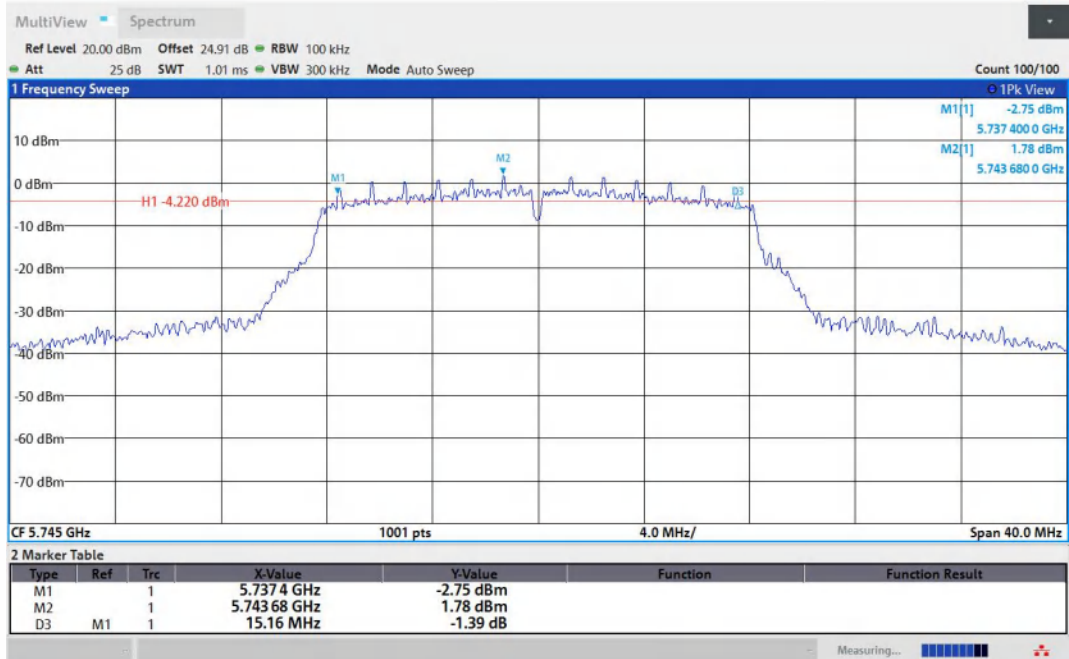
11A-Ant2-5745-PASS
