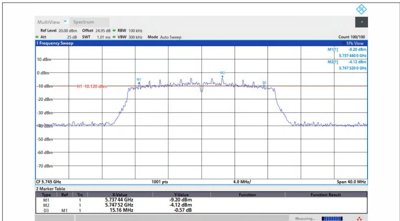
11AC20MIMO-Ant1-5745-PASS
