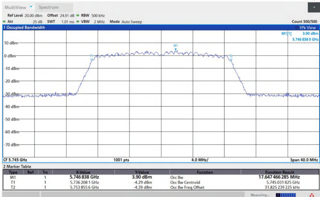
11AC20MIMO-Ant2-5745
