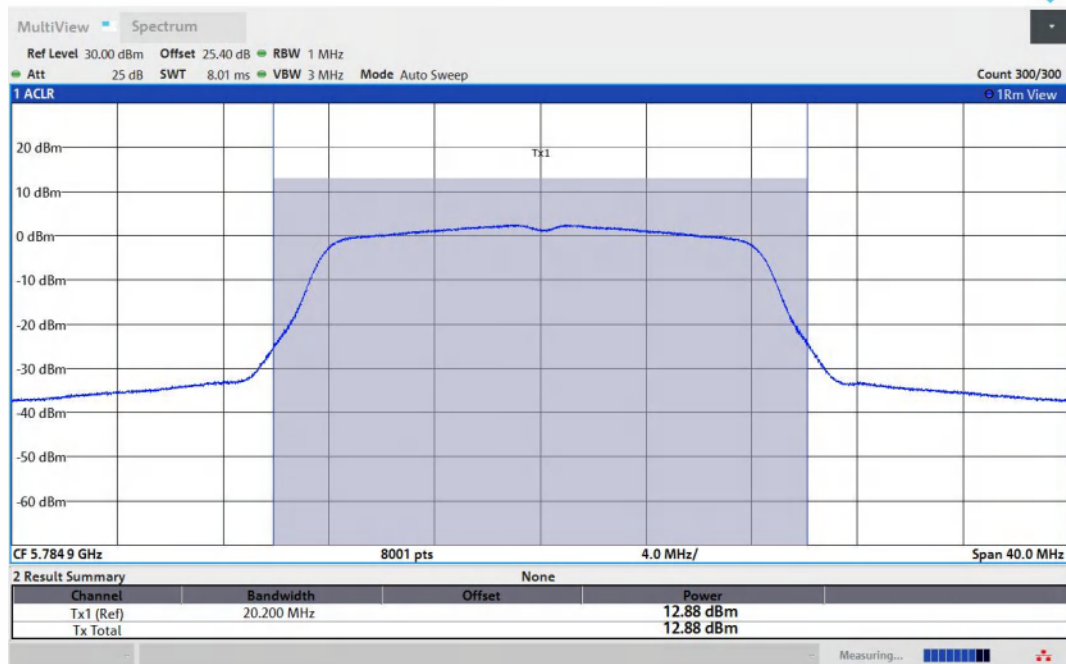
11A-Ant2-5785-PASS
