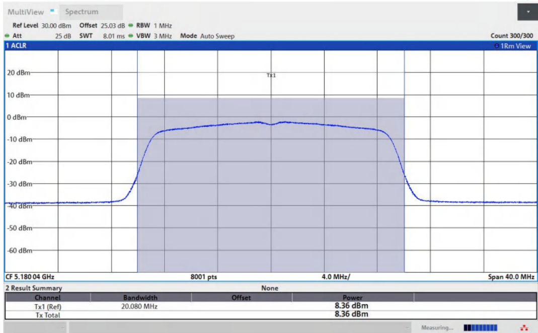
11AC20MIMO-Ant1-5180-PASS
