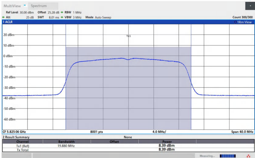
11AC20MIMO-Ant2-5825-PASS
