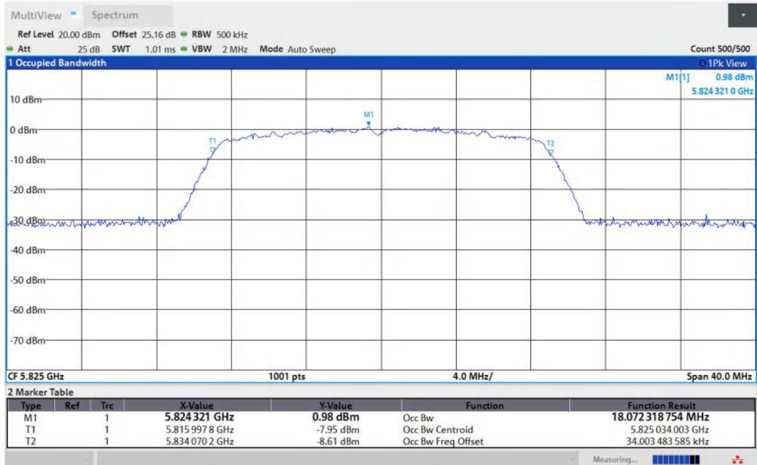
11AC20MIMO-Ant1-5825
