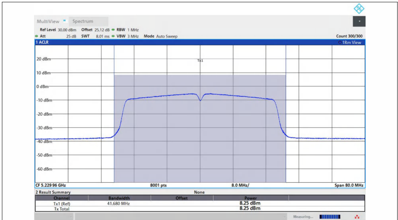
11N40MIMO-Ant1-5230-PASS
