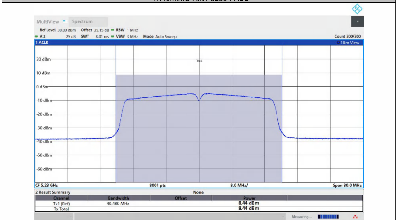
11N40MIMO-Ant2-5230-PASS
