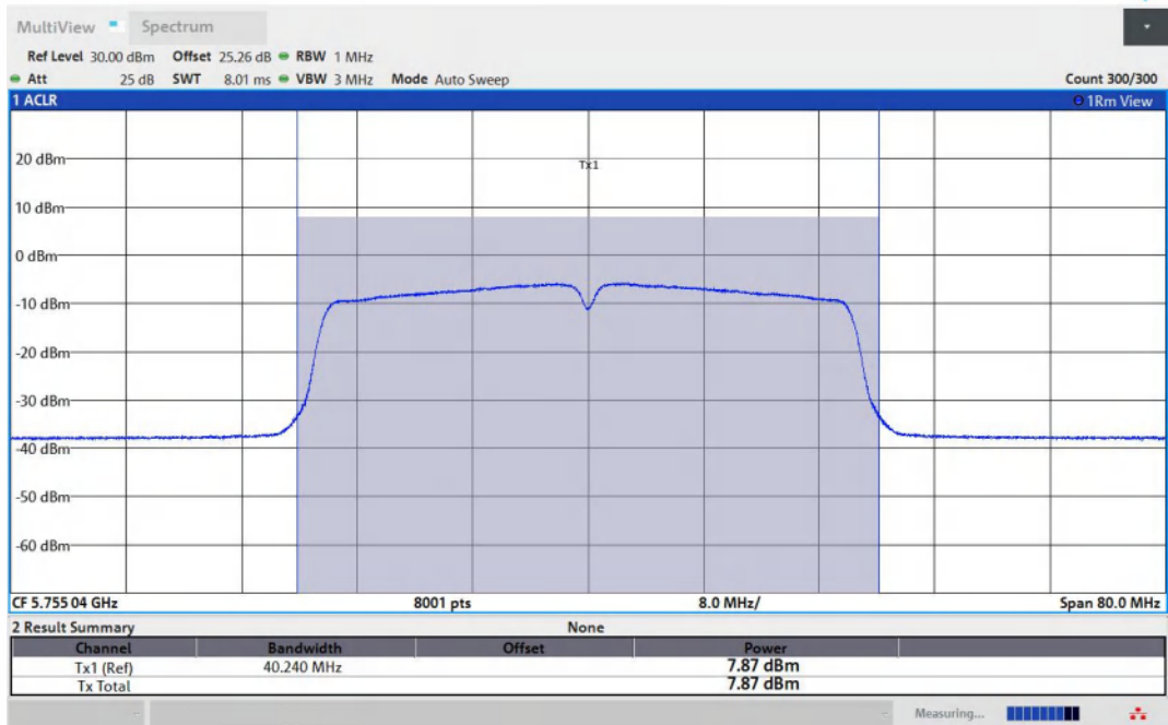
11N40MIMO-Ant2-5755-PASS
