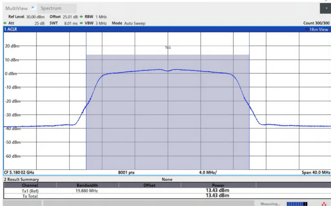
11A-Ant2-5180-PASS
