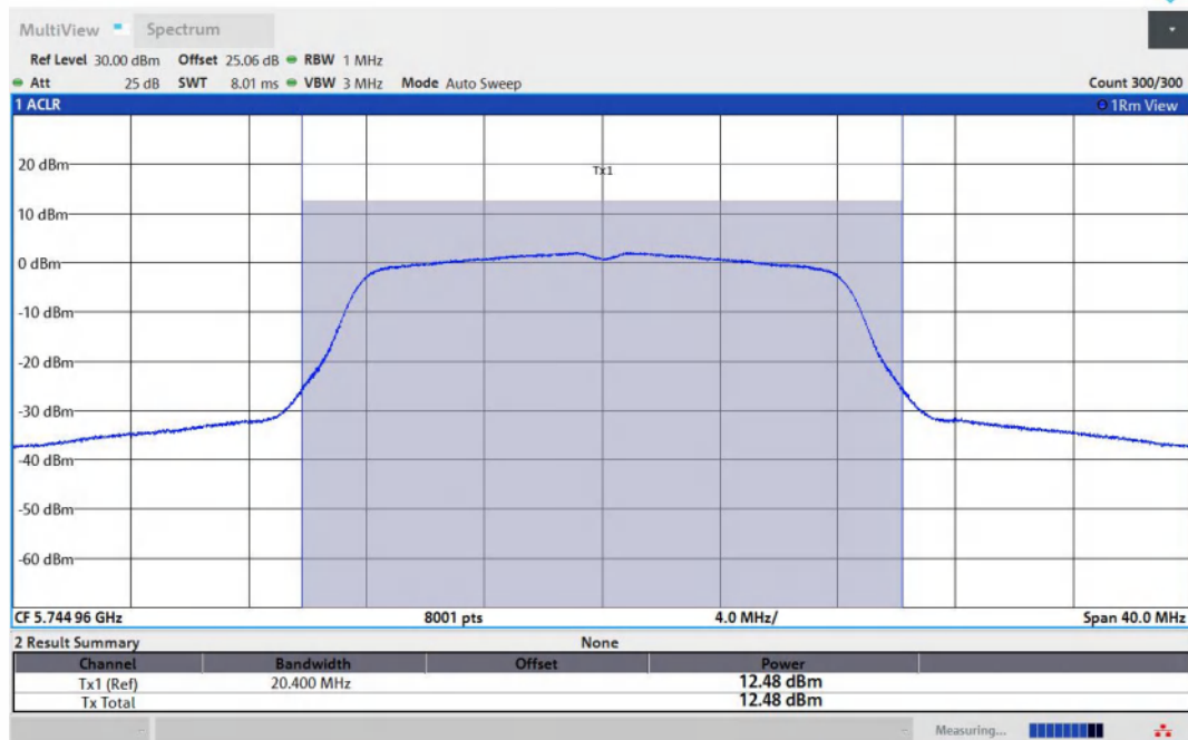
11A-Ant2-5745-PASS
