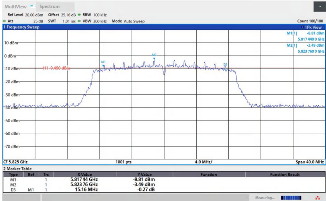
11AC20MIMO-Ant1-5825-PASS
