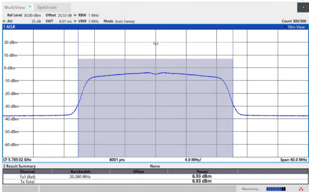
11N20MIMO-Ant1-5785-PASS
