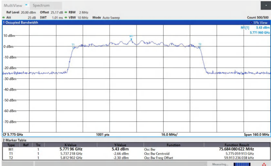
11AC80MIMO-Ant2-5775
