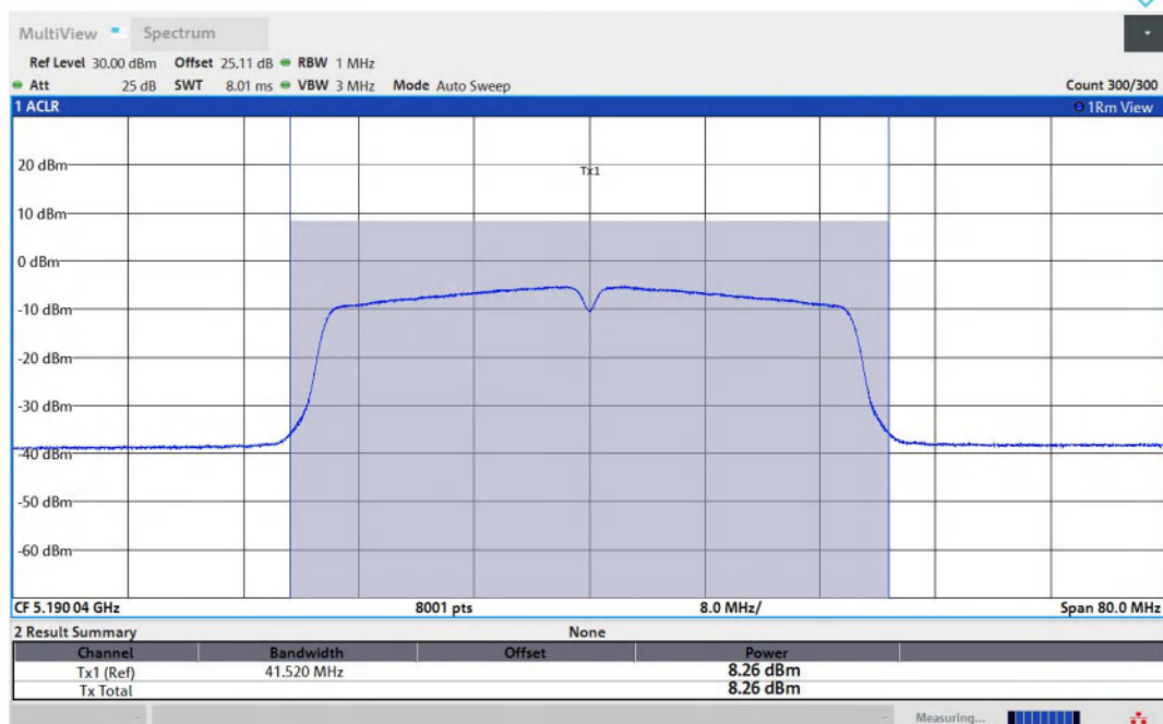
11N40MIMO-Ant1-5190-PASS
