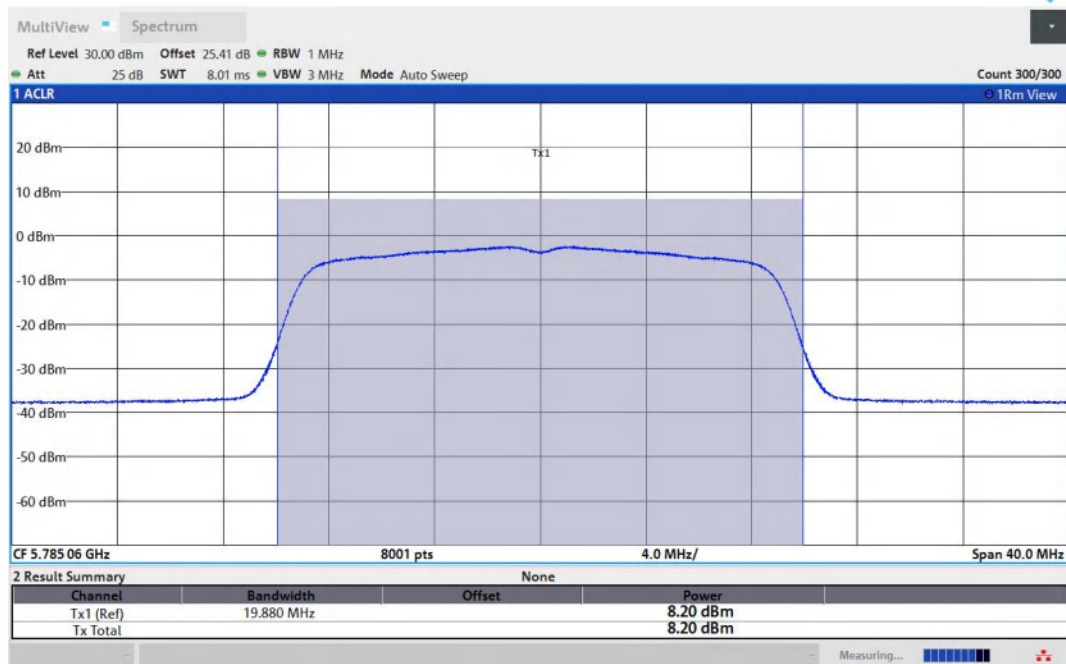
11AC20MIMO-Ant2-5785-PASS
