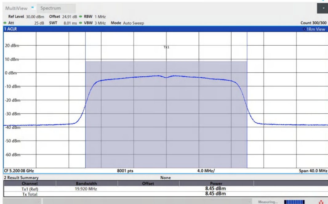
11AC20MIMO-Ant2-5200-PASS
