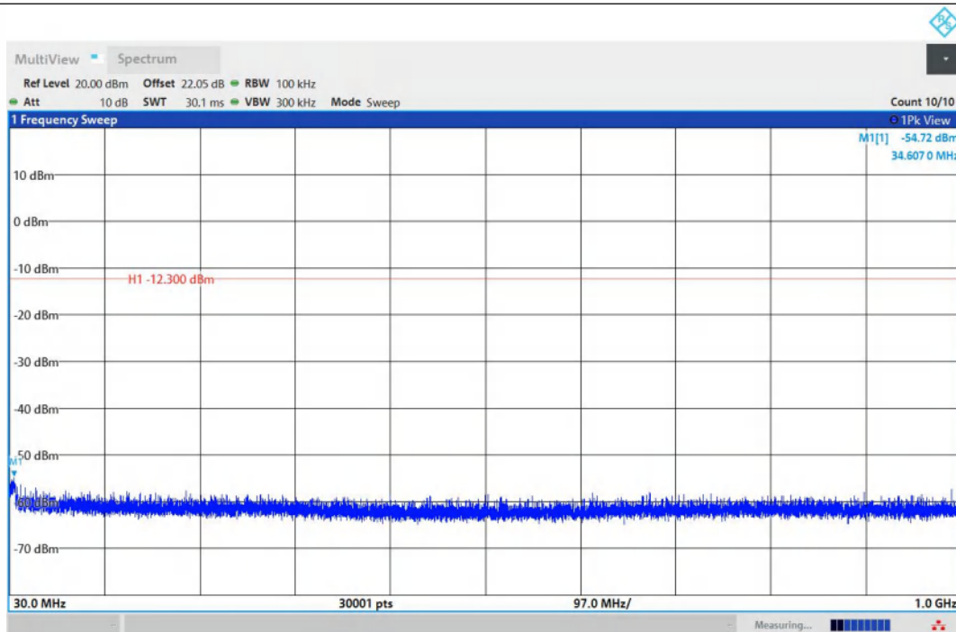
3DH5-Ant1-2402-30~1000-PASS
