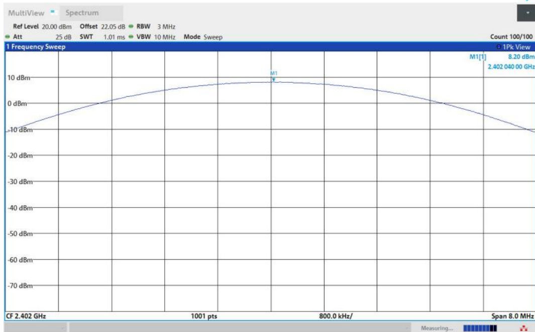
DH5-Ant1-2402-PASS
