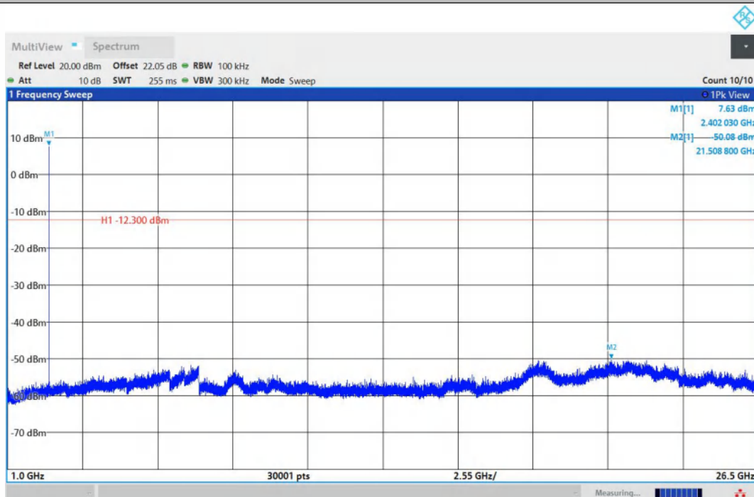
3DH5-Ant1-2402-1000~26500-PASS
