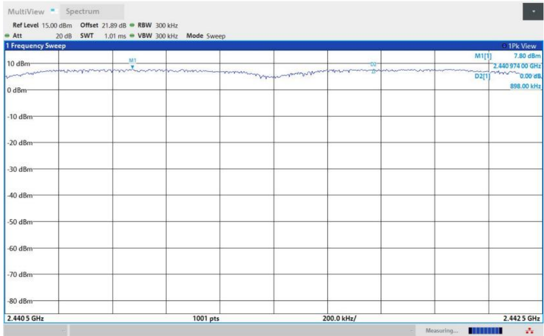
3DH5-Ant1-Hop_2441-PASS
