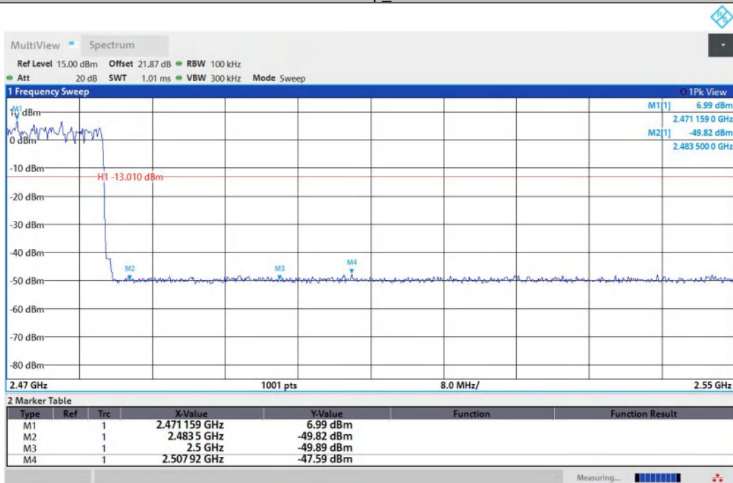
2DH5-Ant1-Hop_2480-PASS
