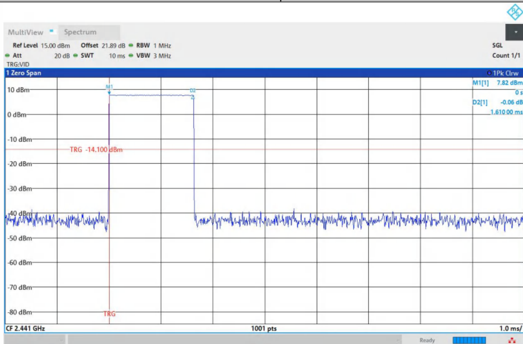
DH3-Ant1-Hop-PASS
