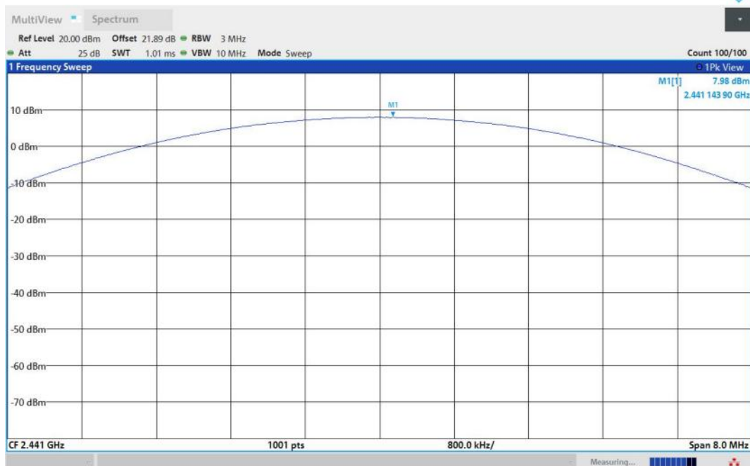
DH5-Ant1-2441-PASS
