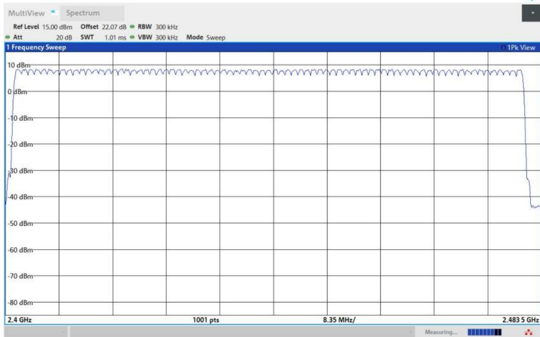
3DH5-Ant1-Hop-PASS
