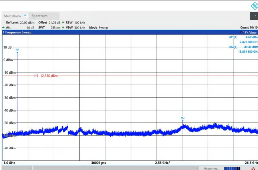
3DH5-Ant1-2480-1000~26500-PASS
