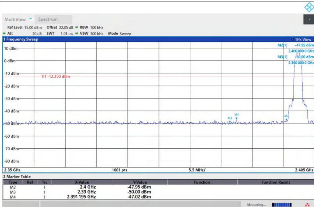
2DH5-Ant1-2402-PASS
