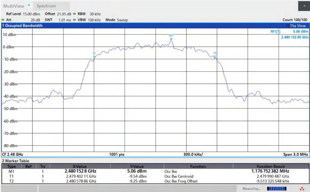
3DH5-Ant1-2480
