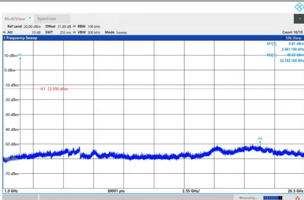
DH5-Ant1-2441-1000~26500-PASS
