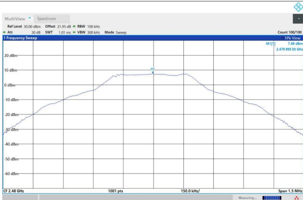
DH5-Ant1-2480-PASS
