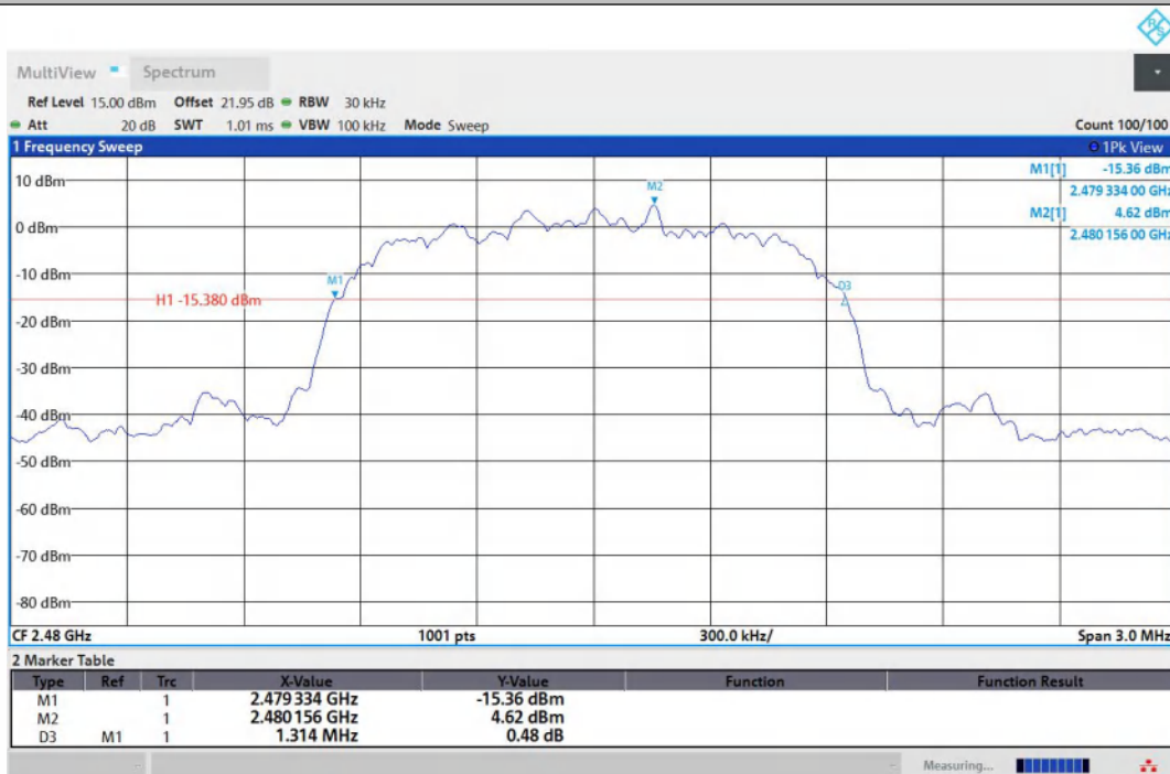
2DH5-Ant1-2480
