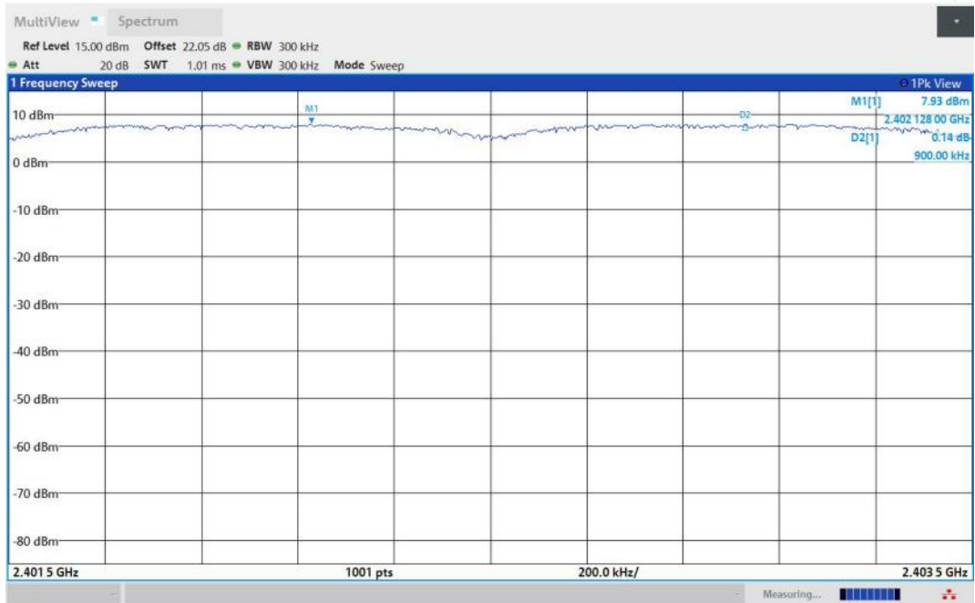
3DH5-Ant1-Hop_2402-PASS
