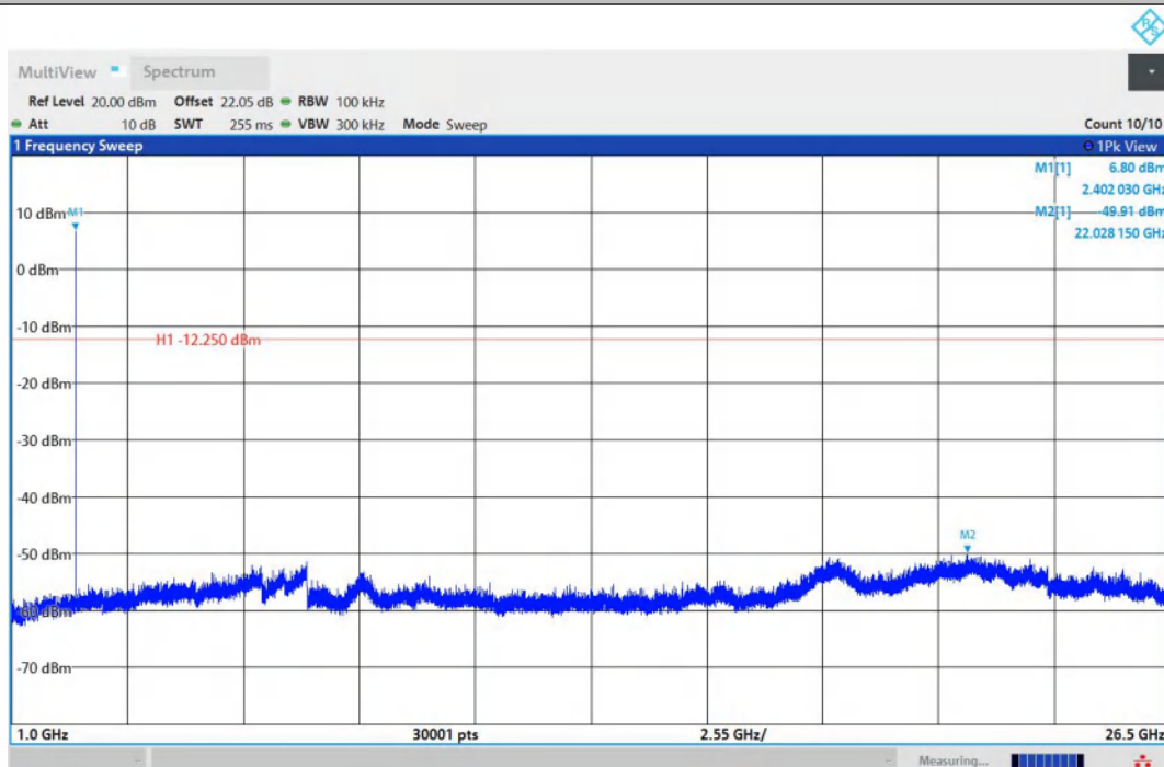
2DH5-Ant1-2402-1000~26500-PASS
