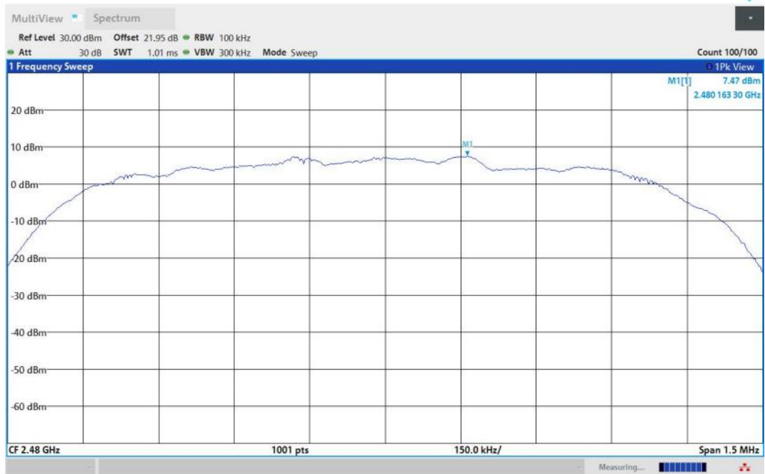
3DH5-Ant1-2480-PASS
