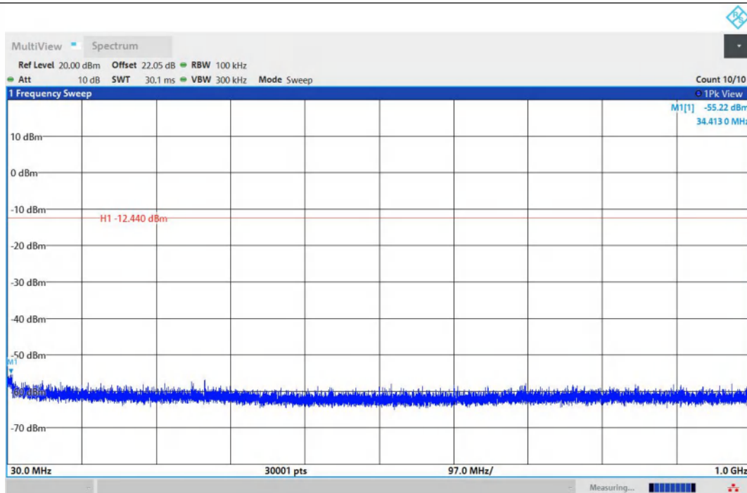
DH5-Ant1-2402-30~1000-PASS
