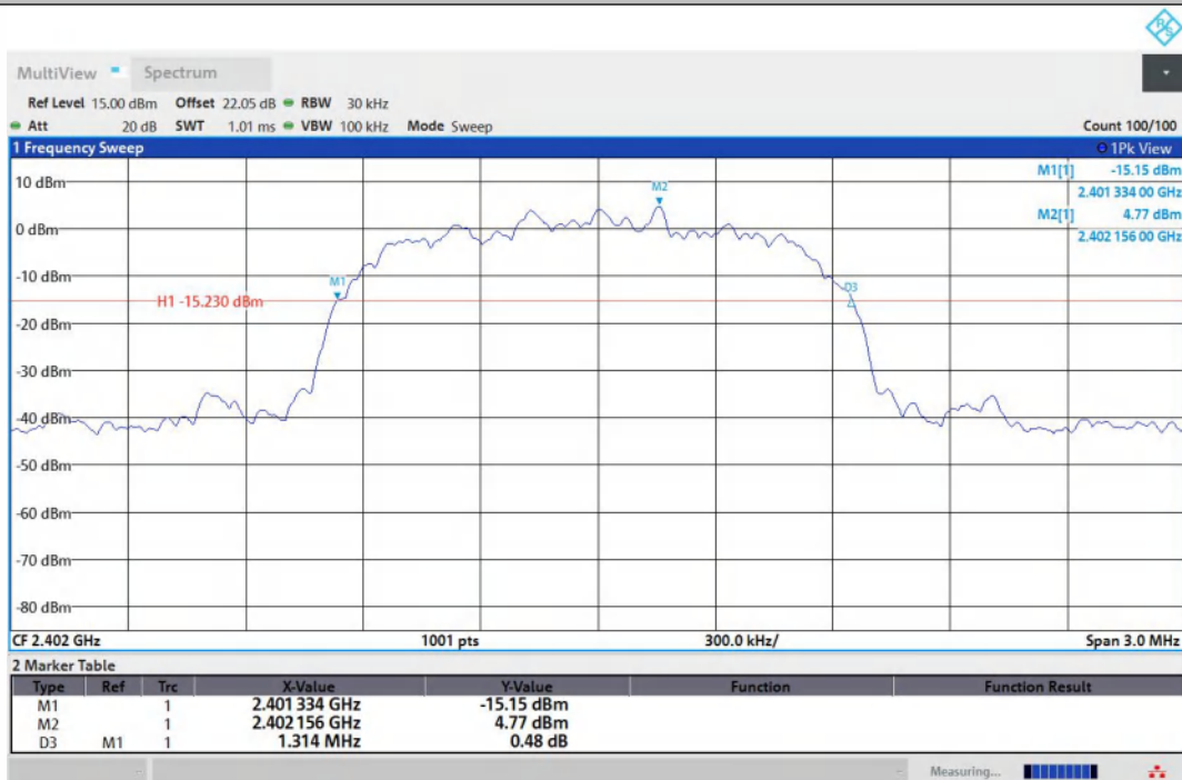
2DH5-Ant1-2402
