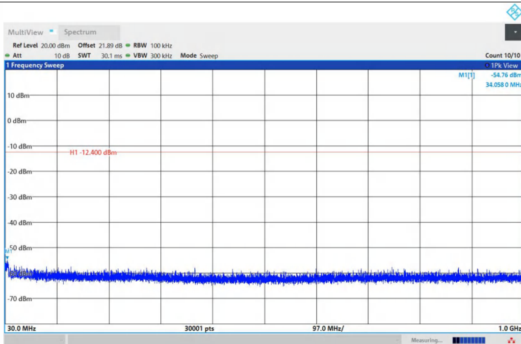
2DH5-Ant1-2441-30~1000-PASS
