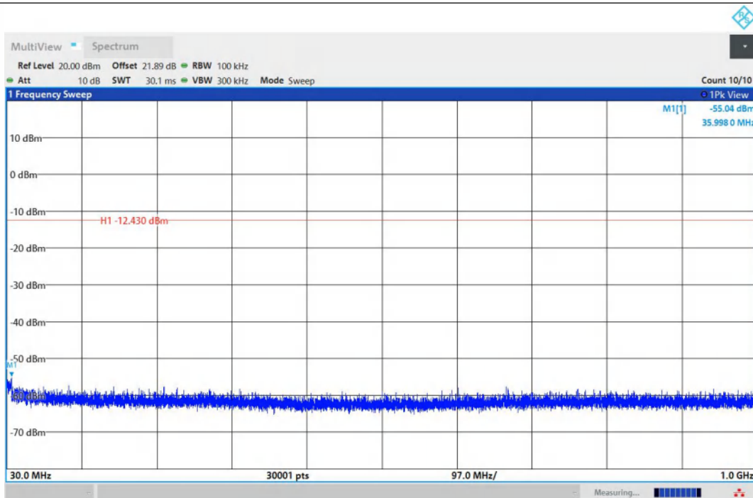
3DH5-Ant1-2441-30~1000-PASS
