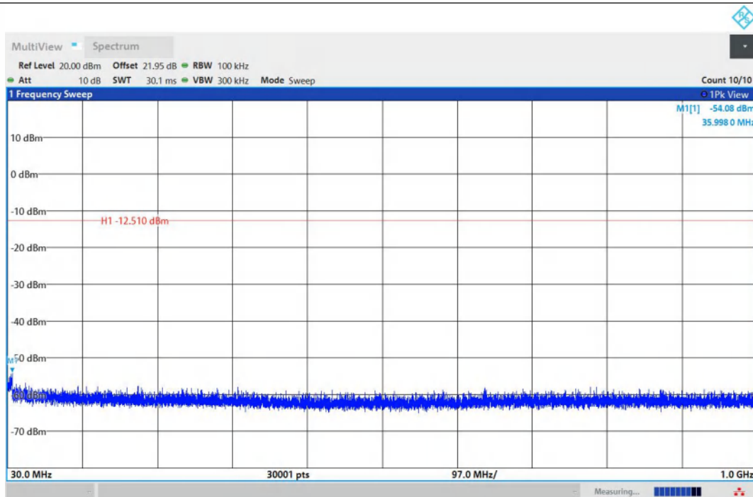
DH5-Ant1-2480-30~1000-PASS
