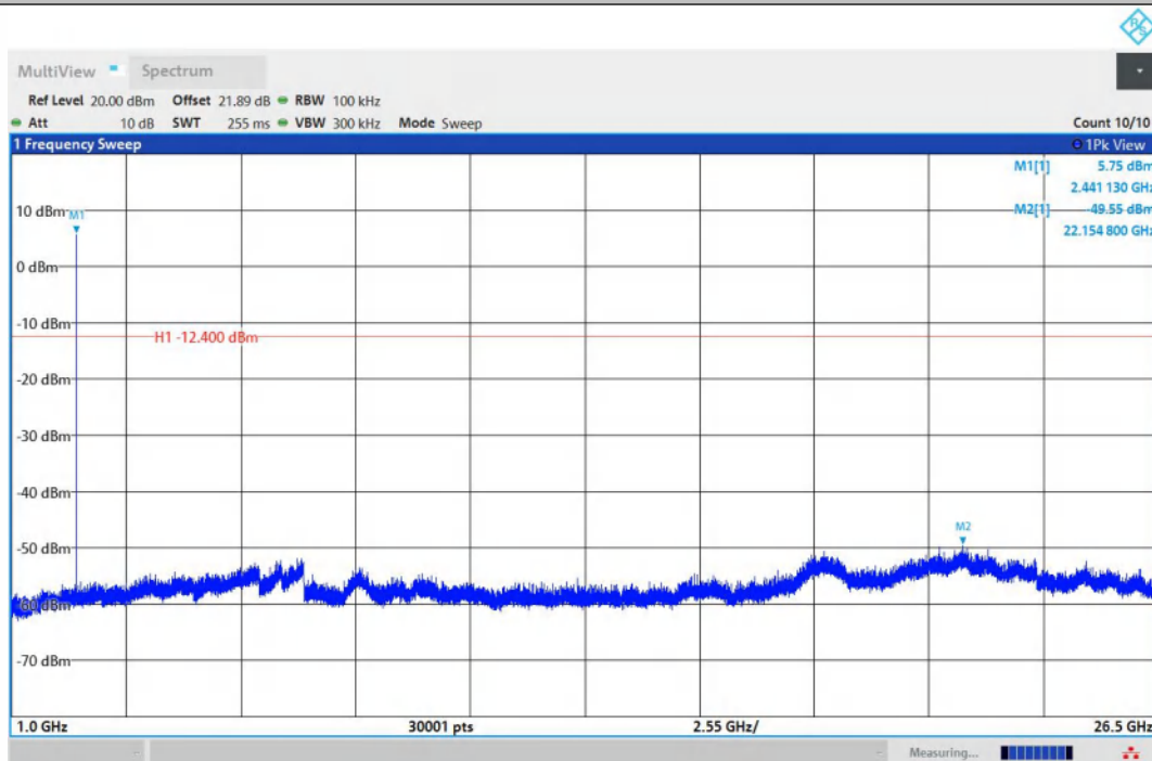
2DH5-Ant1-2441-1000~26500-PASS
