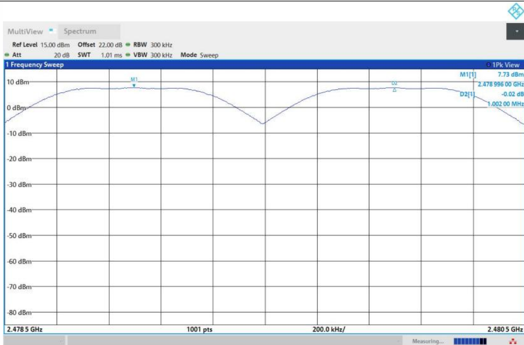
DH5-Ant1-Hop_2480-PASS
