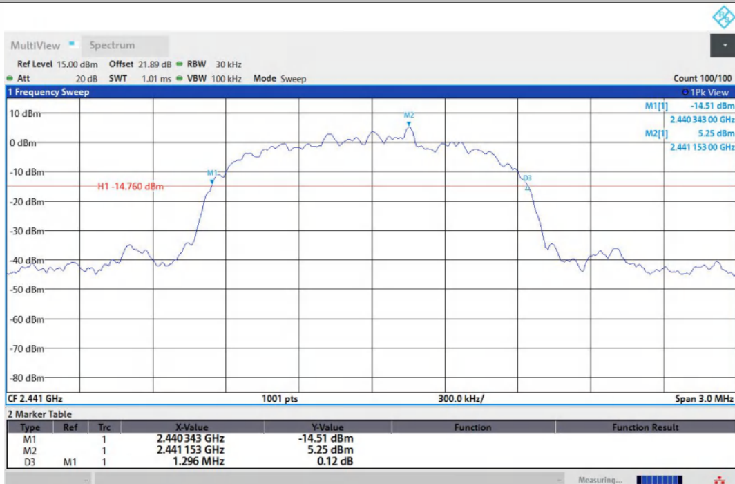
3DH5-Ant1-2441
