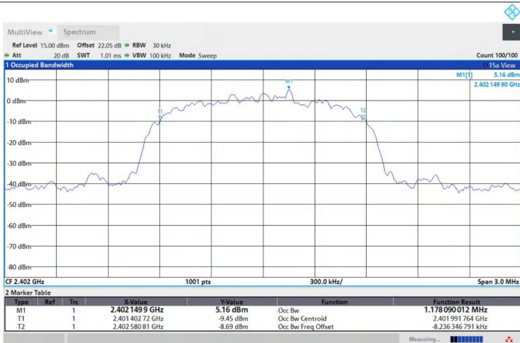
3DH5-Ant1-2402
