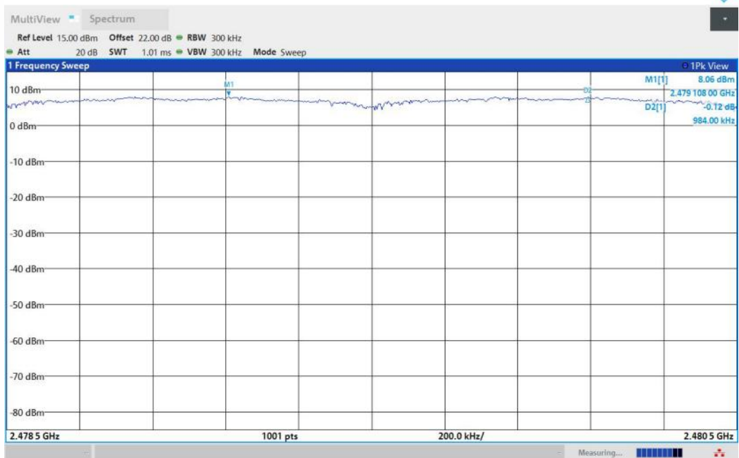
2DH5-Ant1-Hop_2480-PASS
