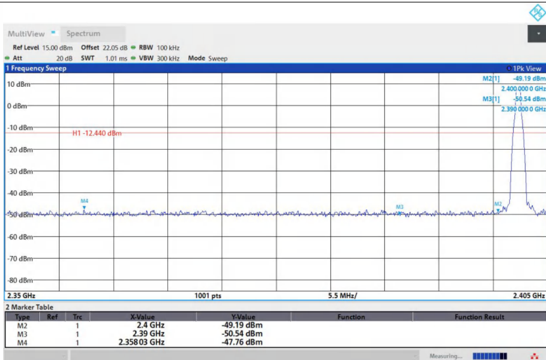
DH5-Ant1-2402-PASS
