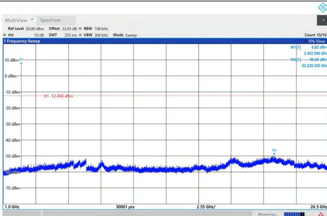
DH5-Ant1-2402-1000~26500-PASS
