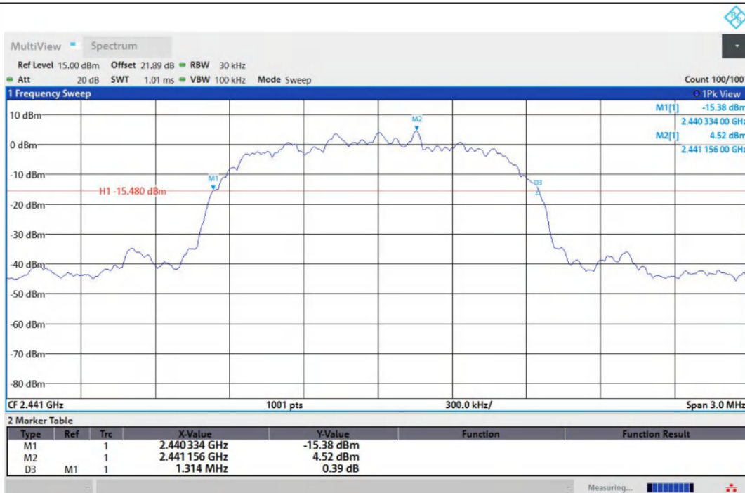
2DH5-Ant1-2441
