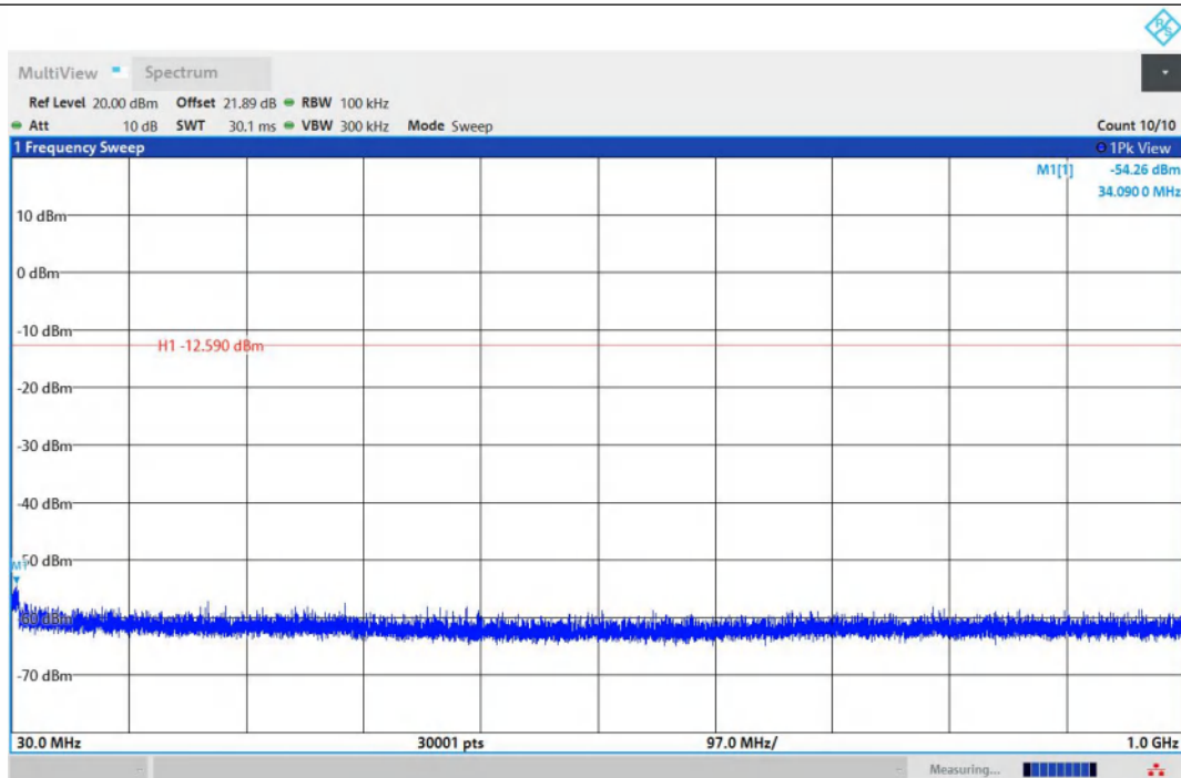
DH5-Ant1-2441-30~1000-PASS
