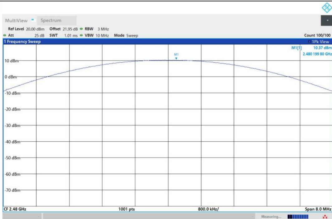
2DH5-Ant1-2480-PASS
