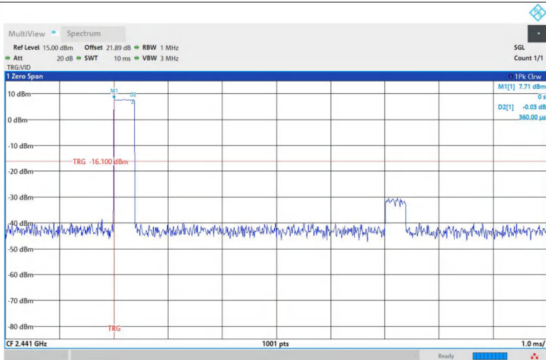
DH1-Ant1-Hop-PASS
