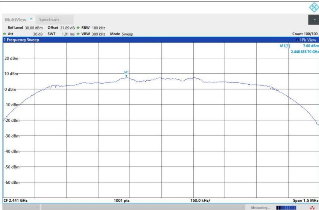
2DH5-Ant1-2441-PASS
