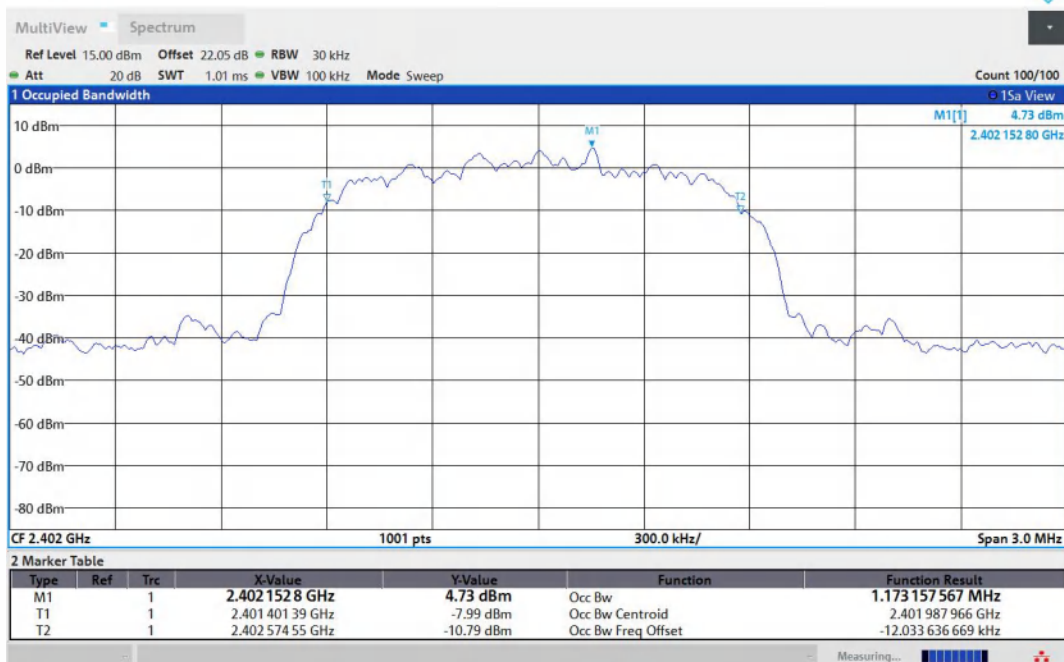
2DH5-Ant1-2402
