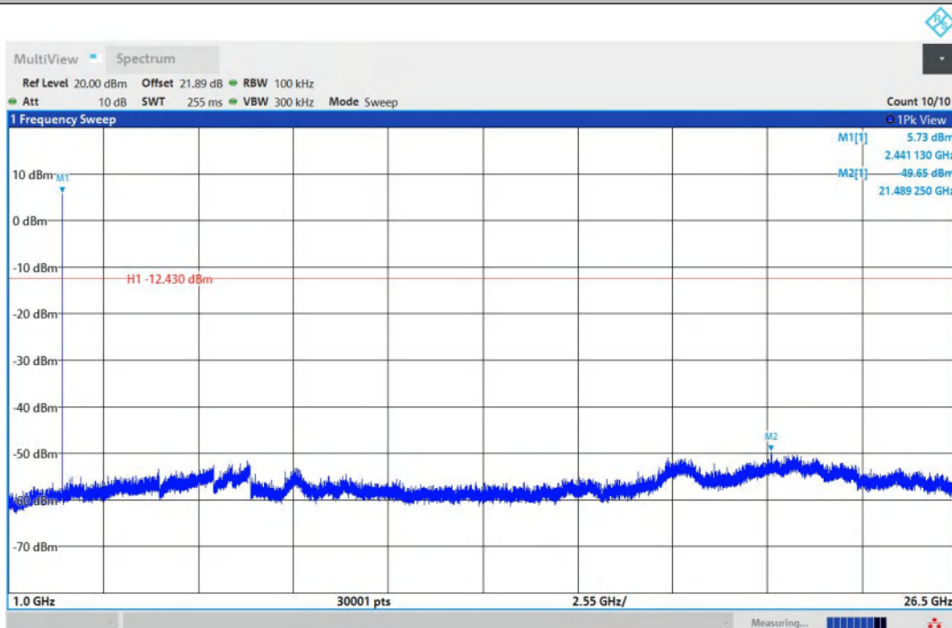
3DH5-Ant1-2441-1000~26500-PASS
