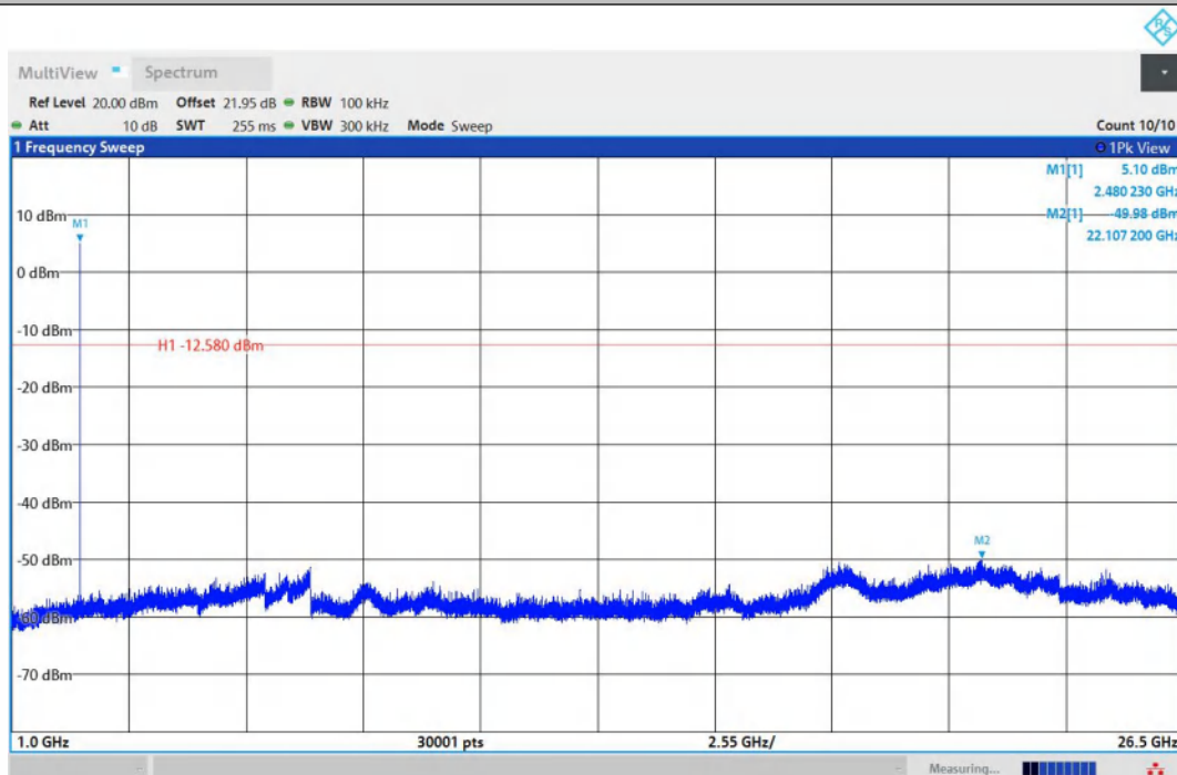
2DH5-Ant1-2480-1000~26500-PASS
