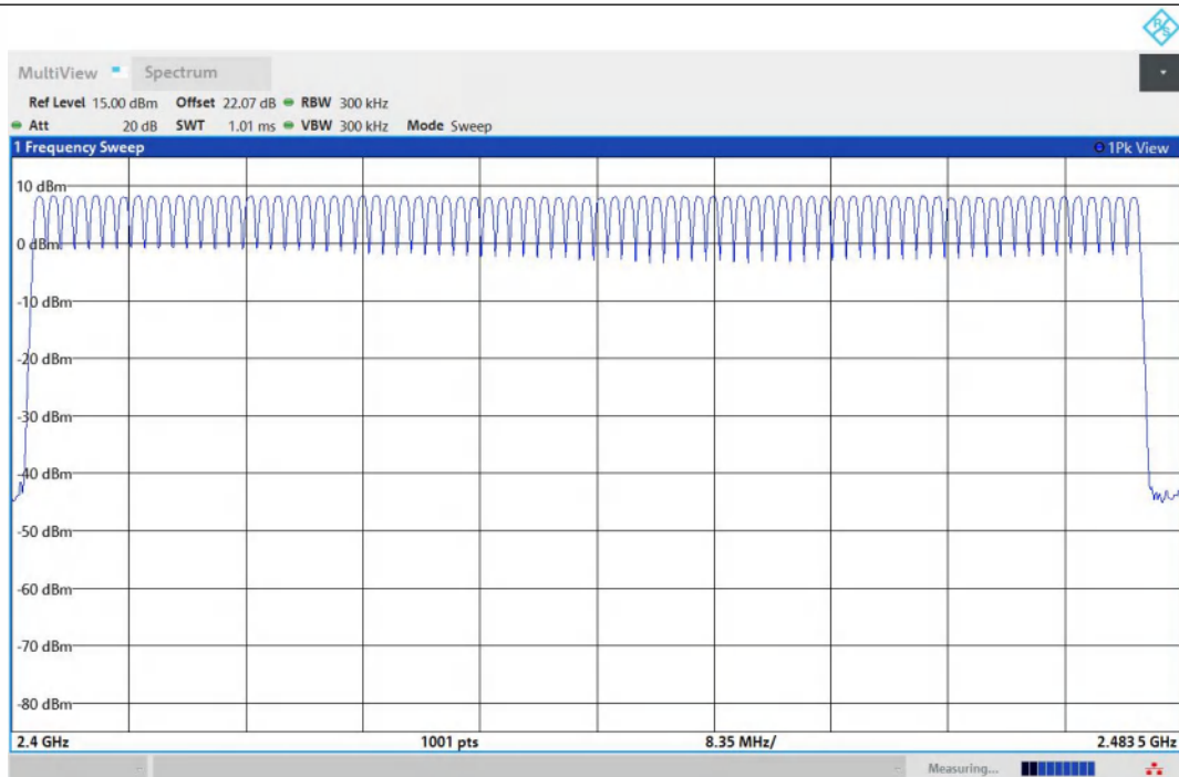
DH5-Ant1-Hop-PASS
