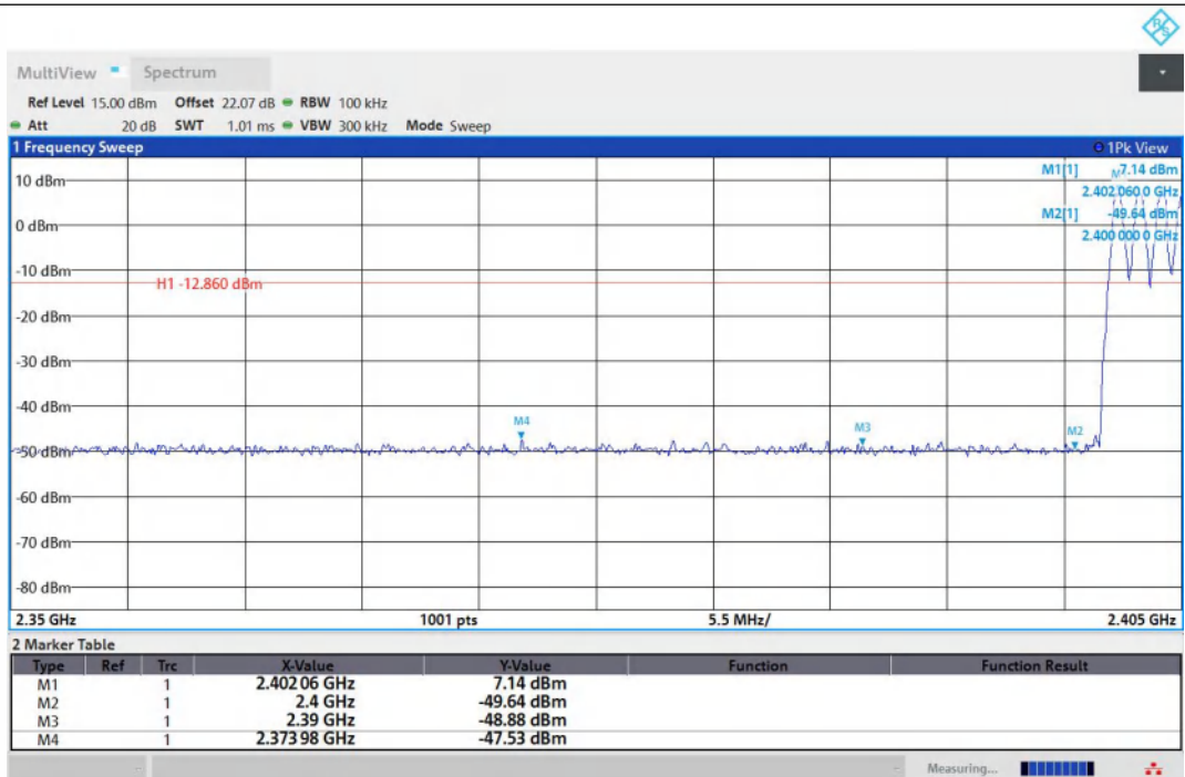
DH5-Ant1-Hop_2402-PASS
