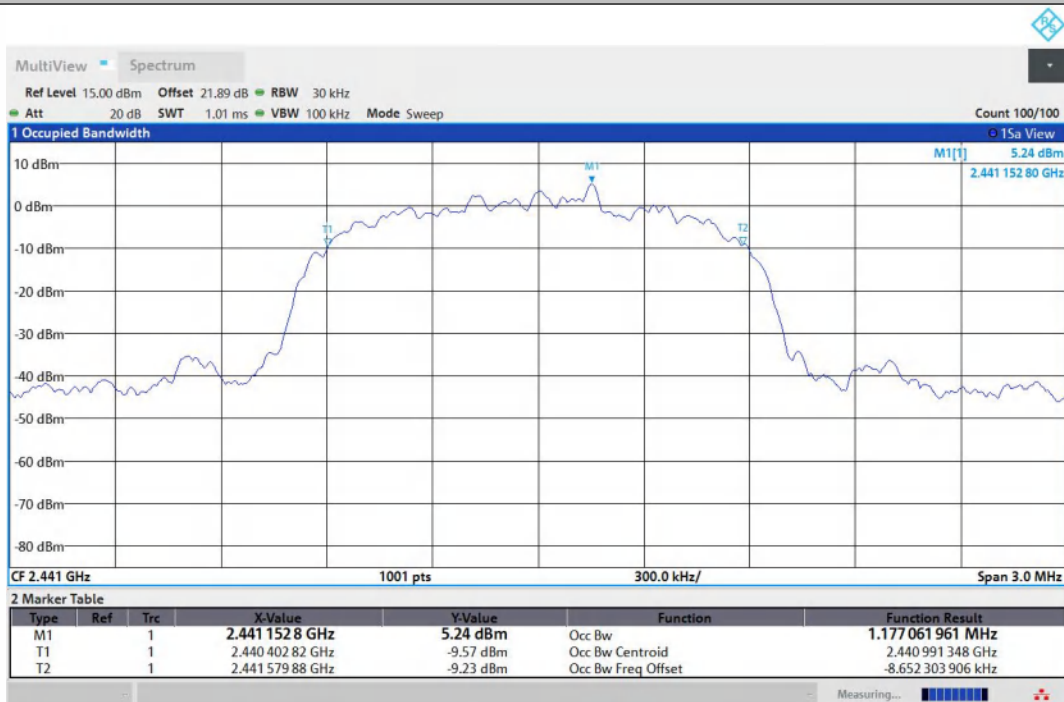
3DH5-Ant1-2441
