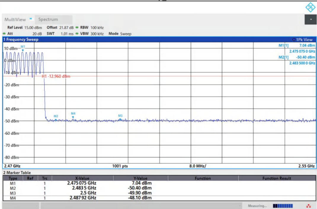
DH5-Ant1-Hop_2480-PASS
