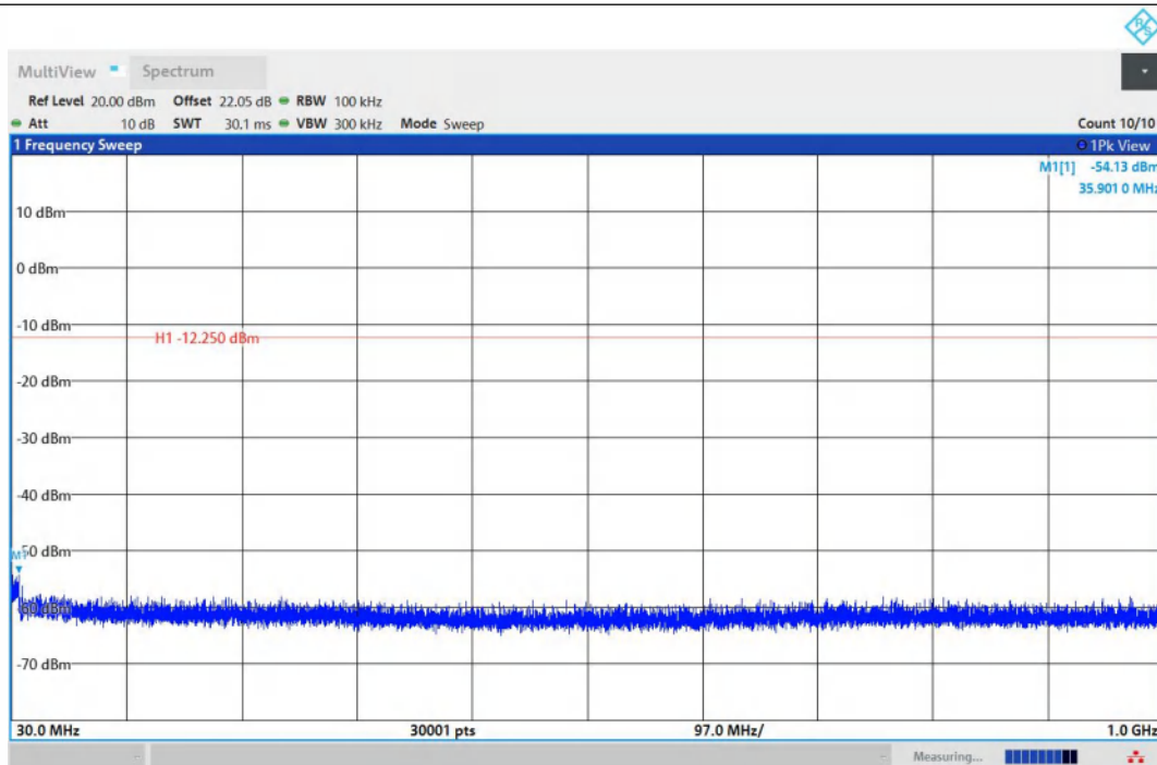
2DH5-Ant1-2402-30~1000-PASS
