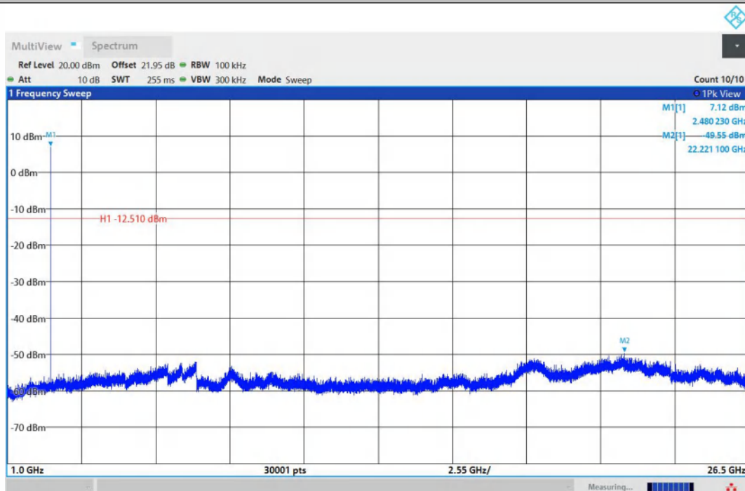
DH5-Ant1-2480-1000~26500-PASS
