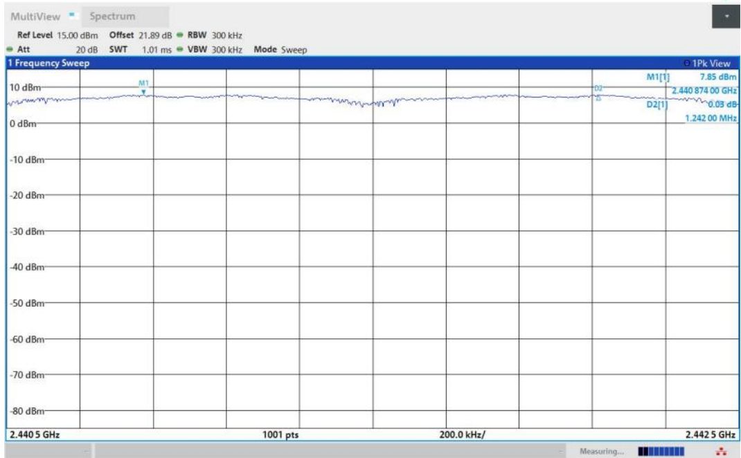
2DH5-Ant1-Hop_2441-PASS
