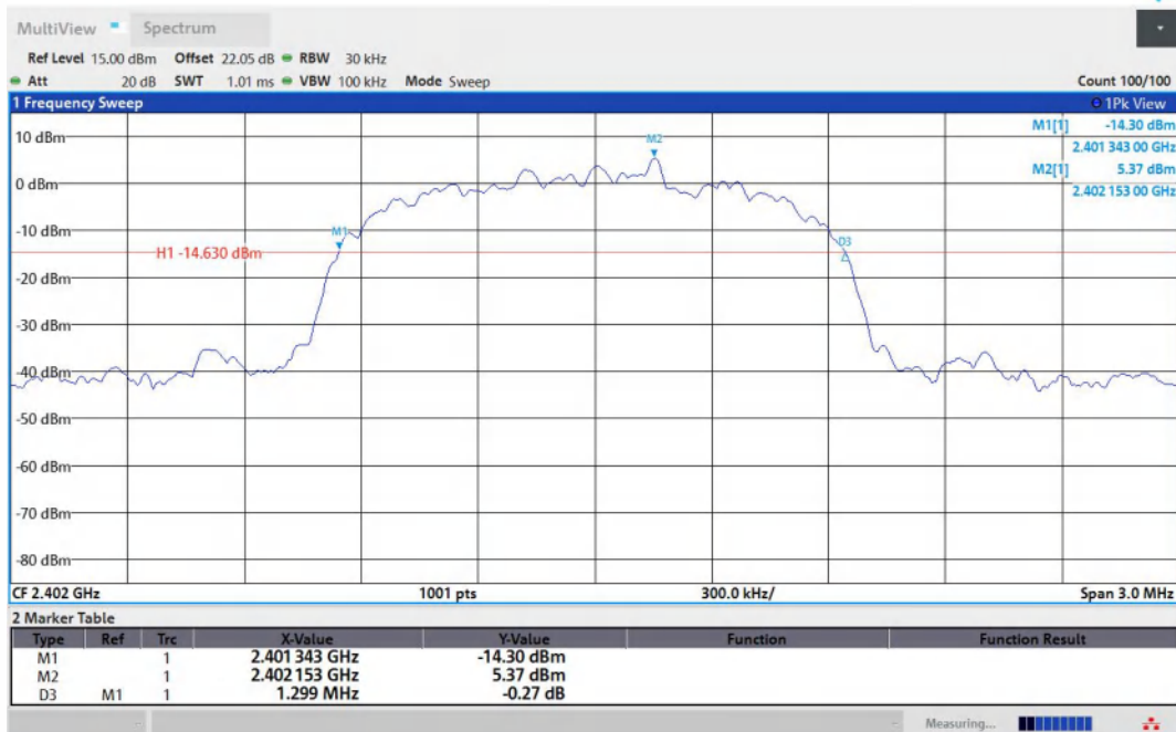
3DH5-Ant1-2402
