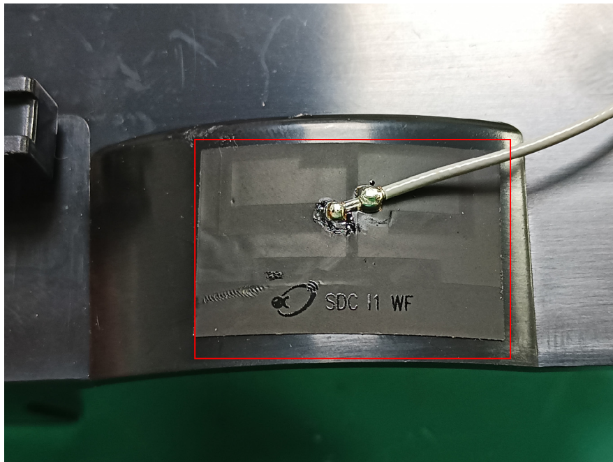
BT/BLE ANT
