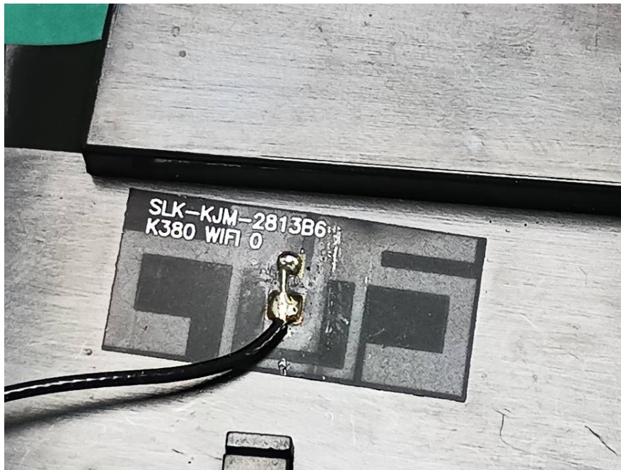
Wi-Fi ANT 0
