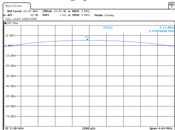
DH1_High 5.14dBm
