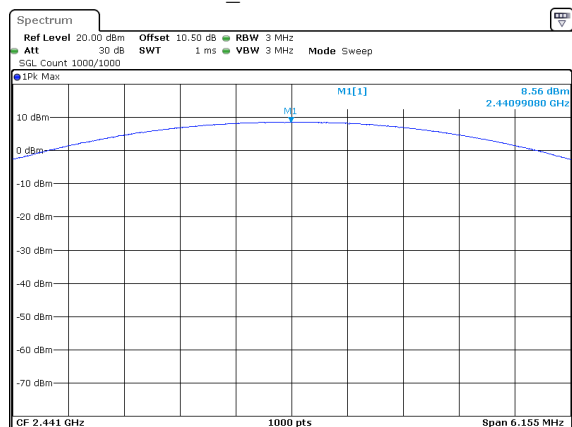
2DH1_Middle 8.56dBm
