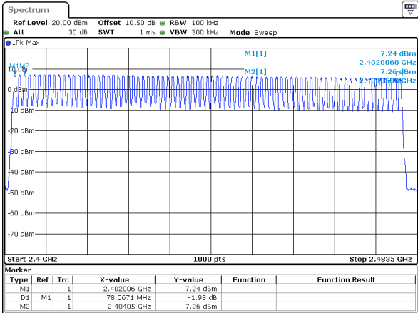
DH1_Hopping 79
