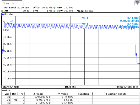
3DH1_Hopping 79
