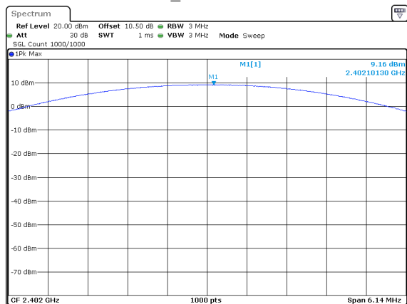
2DH1_Low 9.16dBm
