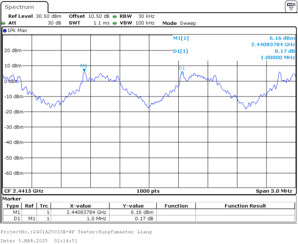
DH1_Middle
