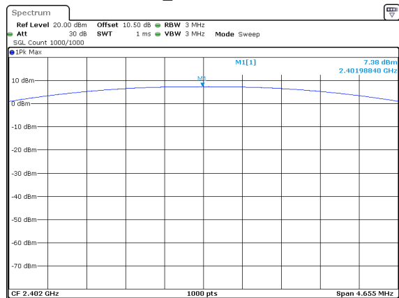
DH1_Low 7.38dBm
