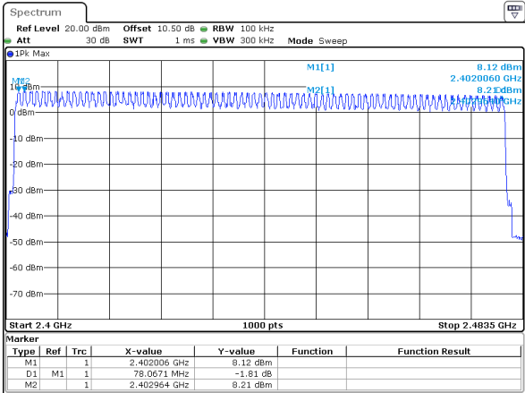
2DH1_Hopping 79
