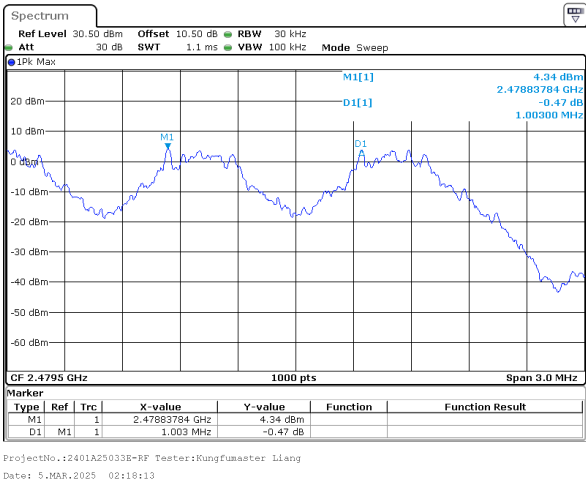
DH1_High
