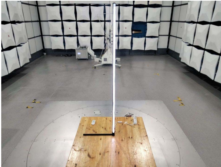
Model: BK-MF-A85D Radiated Emissions
