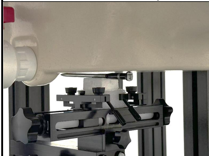
Side 3 of EUT with 0 cm Gap
