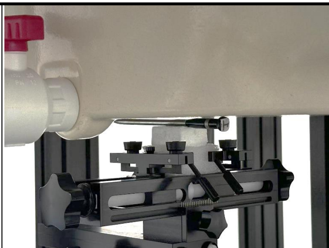
Side 2 of EUT with 0 cm Gap
