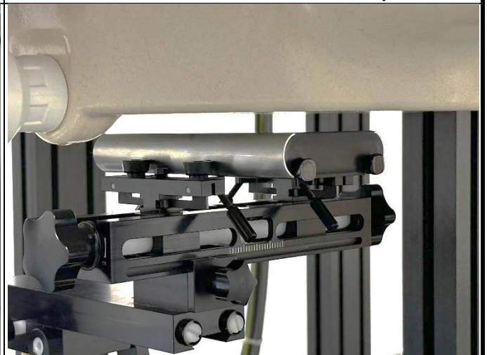
Front Face of EUT + Probe with 10mm Gap
