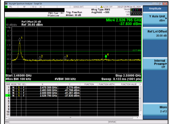
Channel 3 / 2470 MHz
