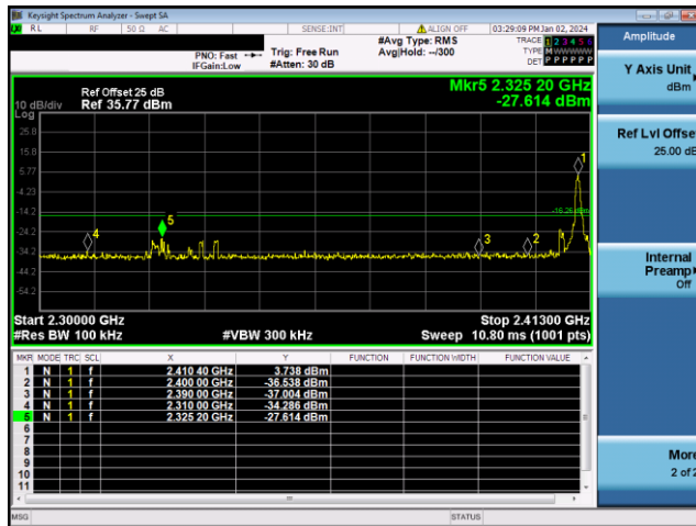
Channel 1 / 2410 MHz
