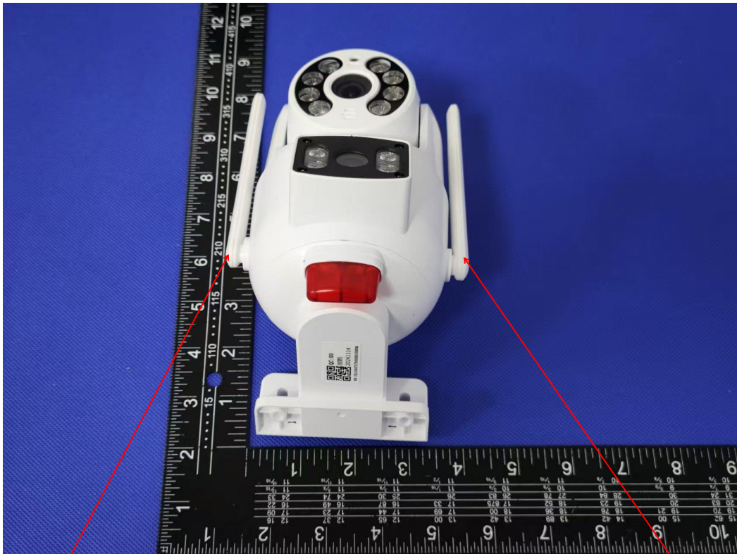
Antenna position
