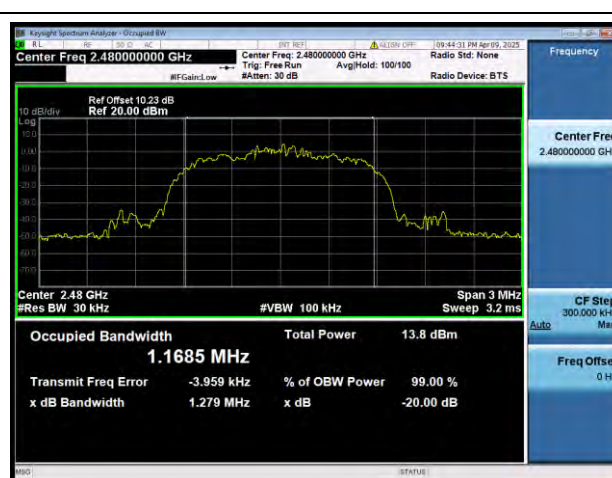
Bluetooth For Classic 2-DH5 2480MHz
