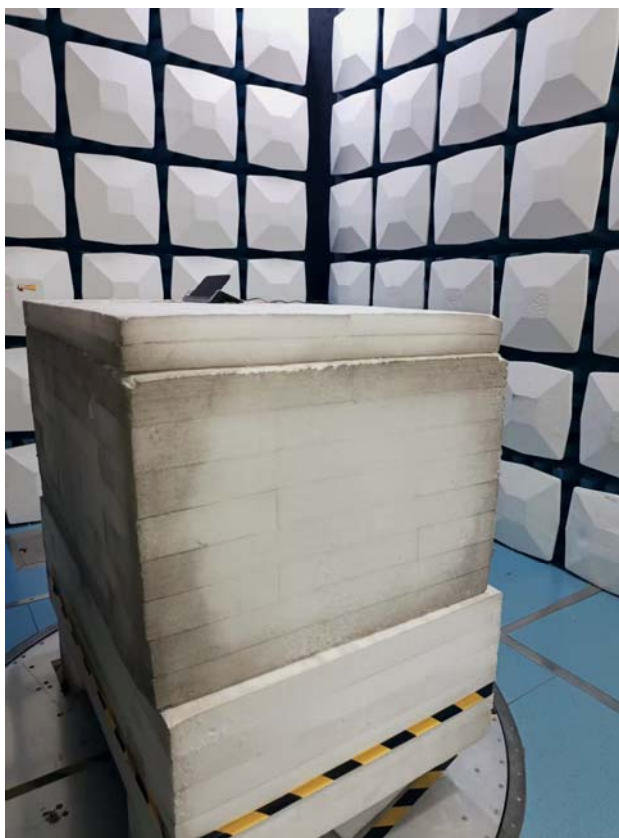
Radiated Emission 90-100GHz View
