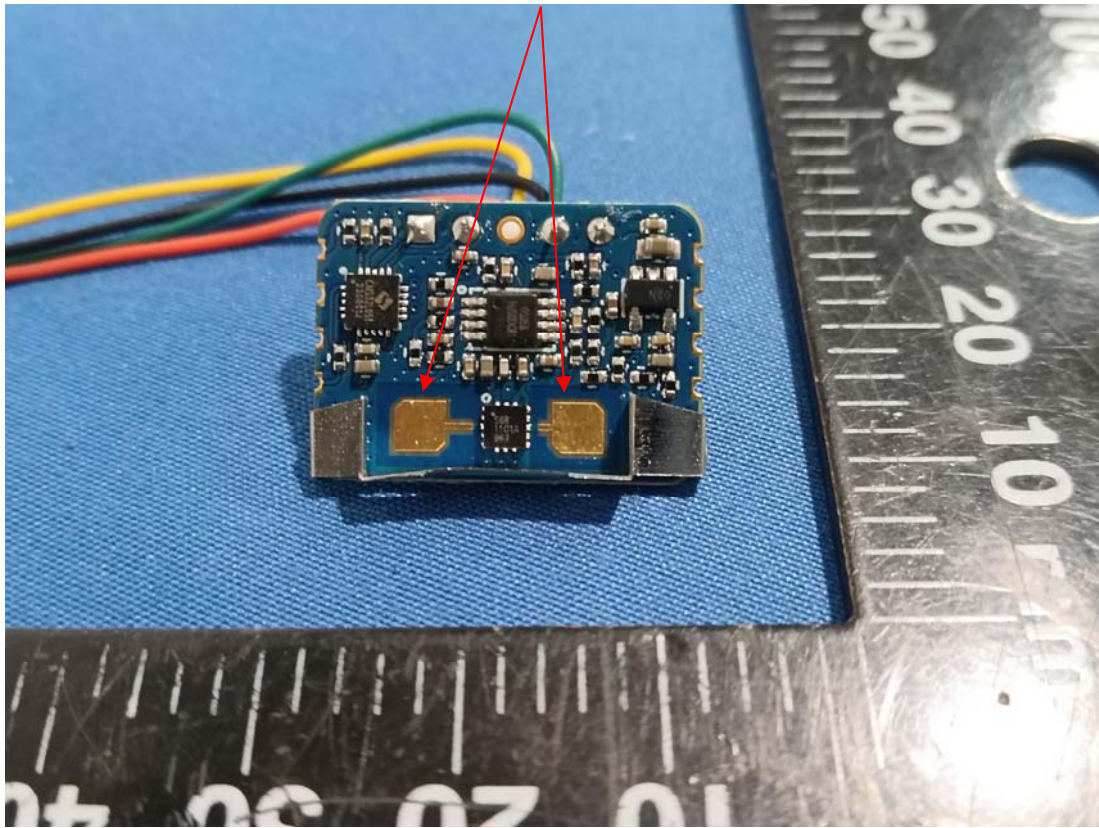
Radar Antenna
