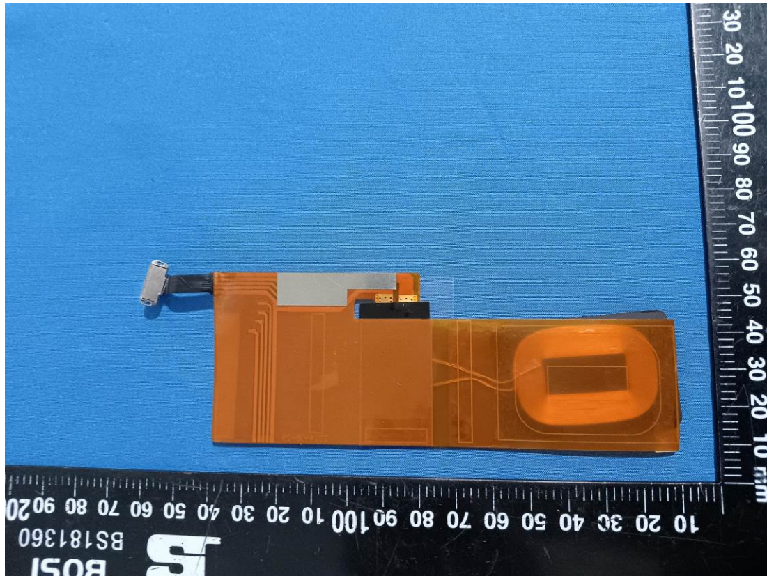
Wireless charge receiving Antenna
