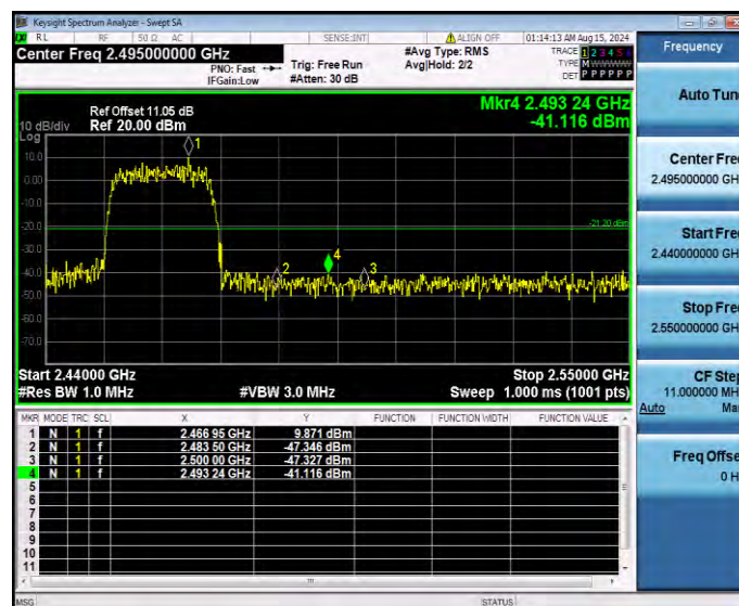
11AX20SISO_Ant1_High_2462_Peak
