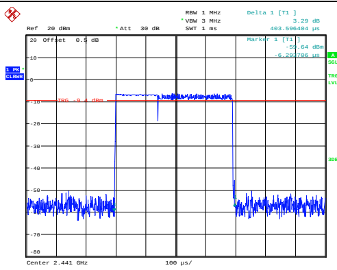
\pi/4 -DQPSK_Hopping_2DH1 0.404ms
