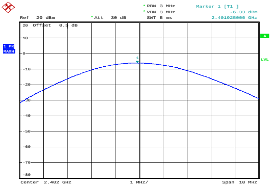
GFSK_Low&-6.33 dBm
