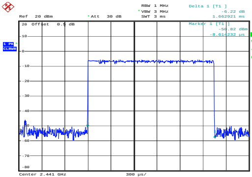
PI/4-DQPSK_Hopping_2DH3&1.663ms
