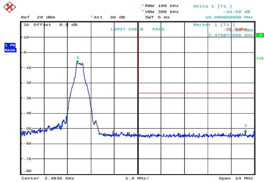
GFSK_High&44.50 dB
