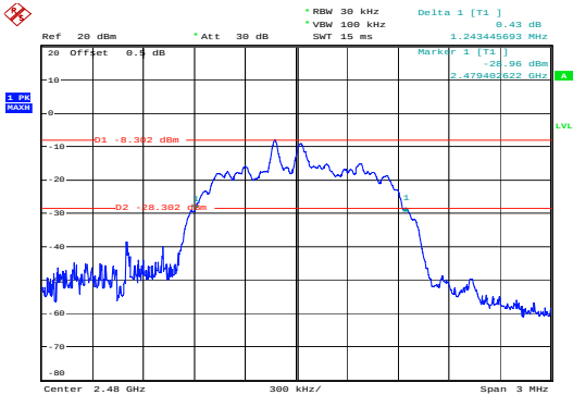
PI/4-DQPSK_High&1.243 MHz
