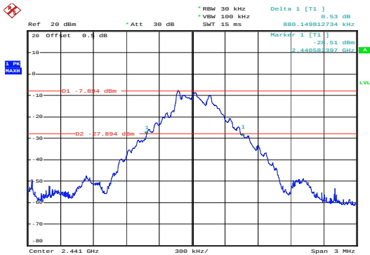
GFSK_Middle&0.880 MHz
