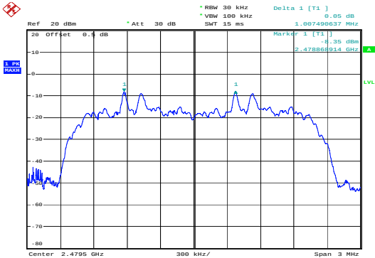
PI/4-DQPSK_High&1.007 MHz
