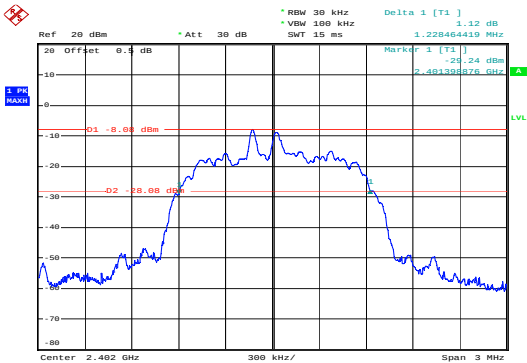
PI/4-DQPSK_Low&1.228 MHz
