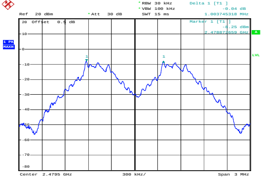
GFSK_High&1.004 MHz
