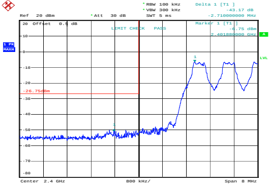
GFSK_Hopping_Lower&43.17 dB
