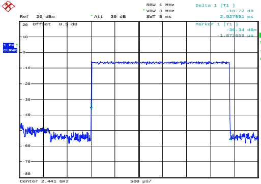
PI/4-DQPSK_Hopping_2DH5&2.928ms
