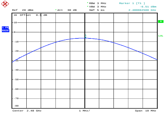
GFSK_High&-6.51 dBm
