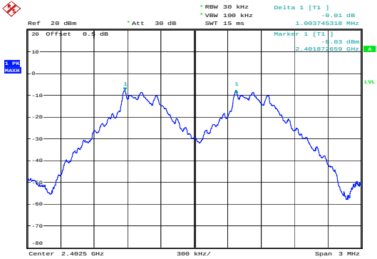
GFSK_Low&1.004 MHz
