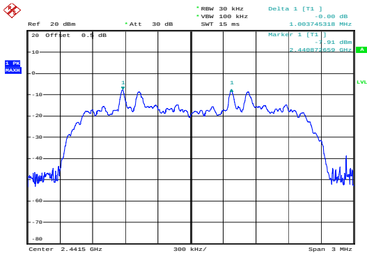
PI/4-DQPSK_Middle&1.004 MHz
