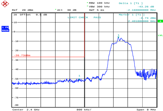
PI/4-DQPSK_Low&43.26 dB
