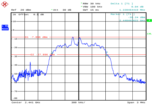
PI/4-DQPSK_Middle&1.228 MHz
