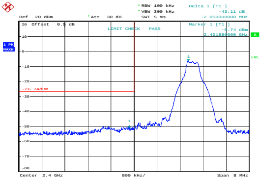
GFSK_Low&43.11 dB
