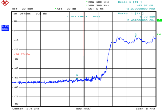
PI/4-DQPSK_Hopping_Lower&43.57 dB
