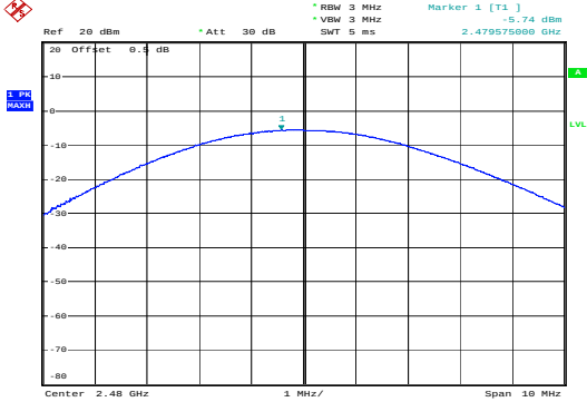
PI/4-DQPSK_High&-5.74 dBm
