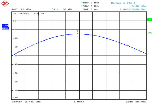
PI/4-DQPSK_Middle&-5.38 dBm
