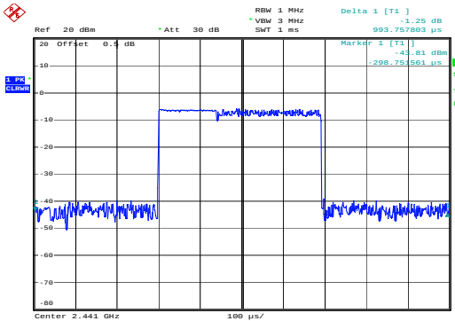
PI/4-DQPSK_Hopping_2DH1&0.994ms
