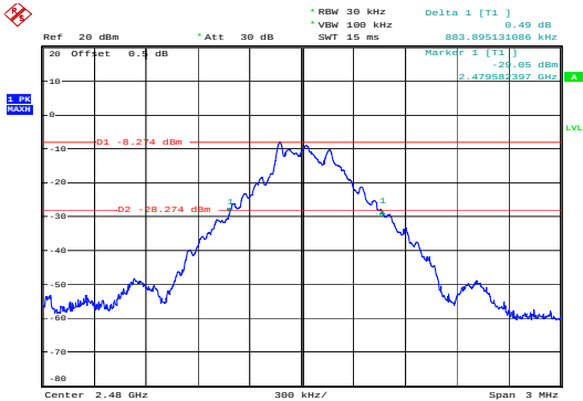
GFSK_High&0.884 MHz
