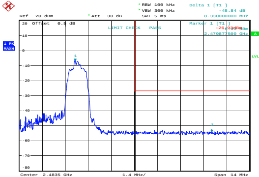
PI/4-DQPSK_High&45.84 dB
