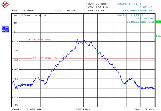
GFSK_Low&0.884 MHz
